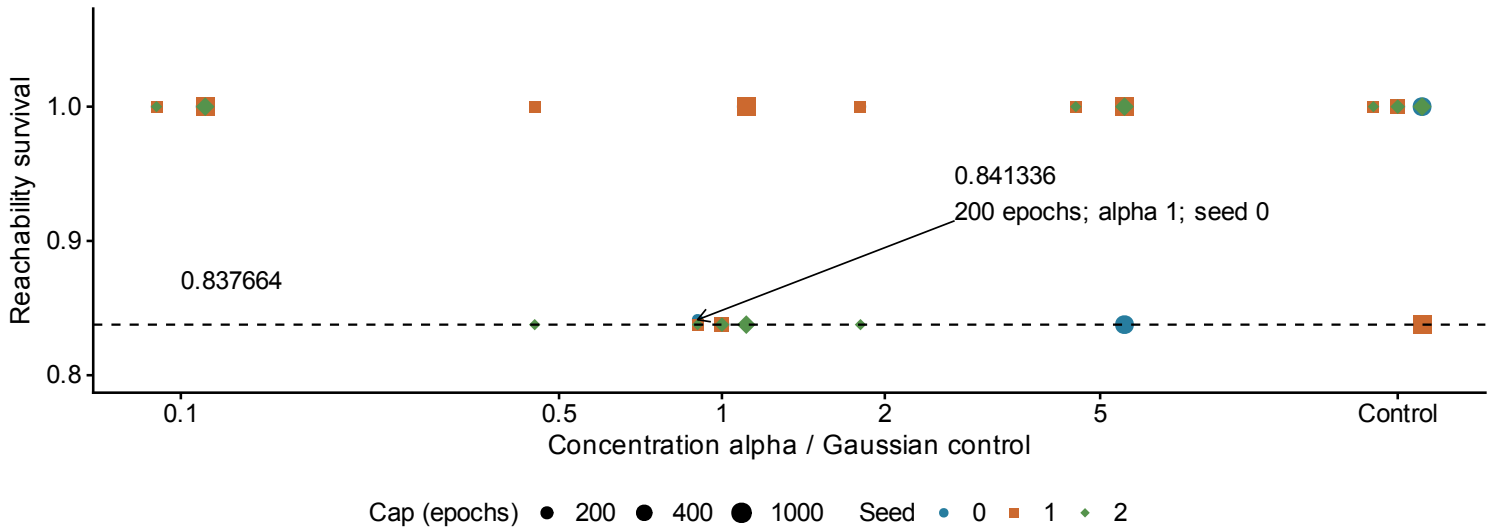
Setty reachability across concentrations and budgets
