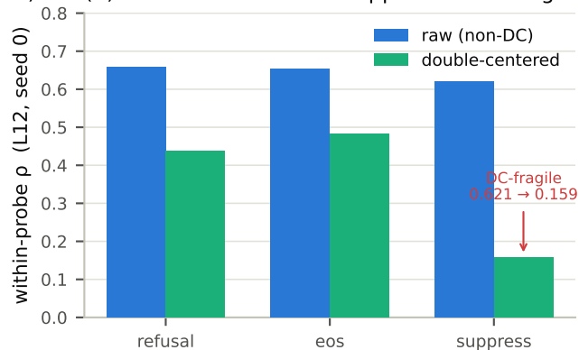
(b) Deletion variants — suppress is DC-fragile
