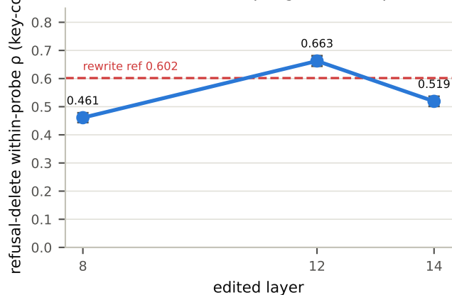
(c) AlphaEdit-delete collapse (3-seed)
