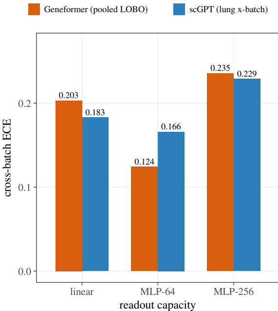
A MLP-256 readout worsens ECE on both FMs
