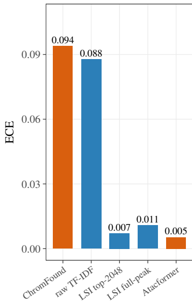
C calibration error
