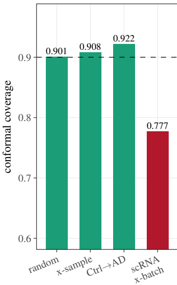
A conformal coverage
