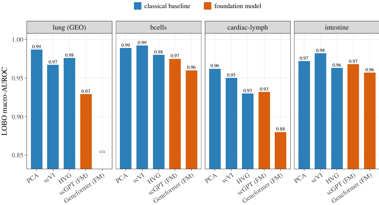
cross-batch LOBO
