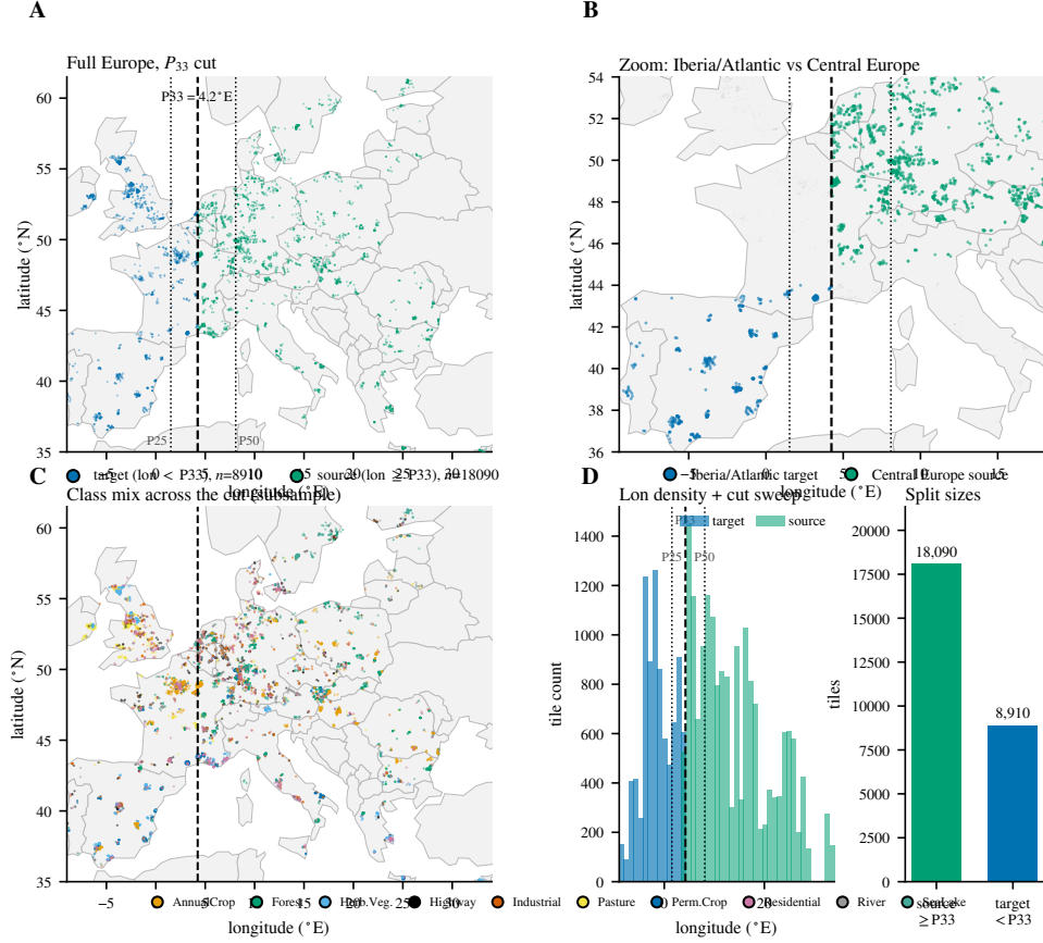
Figure 2: The geographic-shift construction on the map it is defined on (EuroSAT-MS centroids; frozen P_{33} cut = 4.2^{\circ}\text{E} ; source n=18,090 , target n=8,910 ). (a) Full-Europe scatter (4,000/27,000 seeded subsample) colored by split side, with P_{25}/P_{33}/P_{50} longitude guides. (b) Zoom contrasting Iberia/Atlantic target tiles against Central Europe source tiles around the cut. (c) Class-colored geographic mix (same cut; seeded subsample), showing land-cover labels present on both sides. (d) Longitude density with the same percentile guides, and the source/target tile counts. No image transform is applied — the shift is purely geographic.
