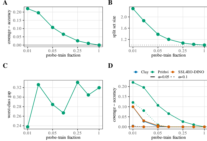
Figure 8: Singleton / low-shot validity boundary from the frozen EuroSAT low-shot sweep (no new runs). Panels (A)–(C) show the Prithvi series at \alpha=0.05 vs. probe-train fraction ( \log-x ). (A) Coverage-accuracy gap: as the budget rises, gap \rightarrow 0 and coverage collapses onto accuracy (degenerate regime). (B) Mean split set size on the same x -axis—a different quantity from (A), not a restatement of the gap; the dotted line at size = 1 is the singleton floor. (C) Worst-class coverage gap vs. fraction (conditional residual under the same sweep). (D) Multi-encoder comparison (Clay, Prithvi, SSL4EO-DINO): coverage-accuracy vs. fraction with colour = encoder and linestyle solid \alpha=0.05 / dotted \alpha=0.10 . Panels (A) and (B) are related through the singleton transition but are not redundant: gap measures coverage-accuracy decoupling, while set size measures how large the prediction sets become once that decoupling appears.
