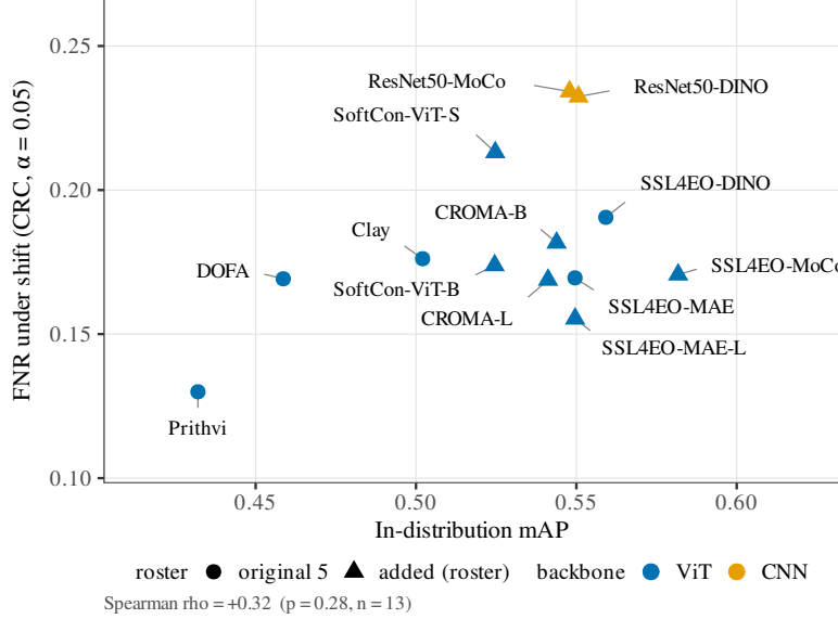
Figure 5: The five-encoder inversion does not survive expansion to thirteen. FNR under shift vs. in-distribution mAP on m-bigeathnet ( \alpha=0.05 , CRC arm); circles are the original five encoders, triangles the eight added at pull. The rank correlation is a weak, non-significant positive (Spearman +0.32 , permutation p=0.28 , n=13 ; no trend line is drawn, since the correlation does not reach significance): accuracy never buys better FNR robustness, but the strong +0.90 inversion of the five-encoder slice regresses toward zero. Prithvi (least accurate) remains the most FNR-robust; the two ResNet50 CNNs are the most fragile at mid accuracy.
