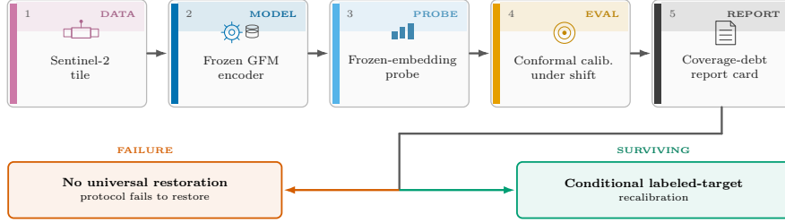
Figure 1: Overview of the pre-deployment reliability report-card protocol. Stages 1–5 (left to right), role-tagged DATA / MODEL / PROBE / EVAL / REPORT: (1) optical Sentinel-2 tile (EuroSAT-MS / GEO-Bench BigEarthNet-S2 / m-so2sat); (2) one frozen, interchangeable optical GFM encoder under audit on EuroSAT/BigEarthNet (Prithvi, Clay, SSL4EO-DINO, SSL4EO-MAE, DOFA; on m-so2sat the ViT-S slot substitutes SSL4EO ViT-S/16 MAE for DINO—same five-encoder size , not an identical checkpoint roster); (3) frozen-embedding probe (logistic for single-label tasks, multi-label otherwise); (4) conformal calibration under real geographic region-transfer shift (source split-conformal vs. spatial-Mondrian target-region calibration; source = E/Central Europe, target = W/Iberian-Atlantic Europe), yielding per-class conformal sets; (5) coverage-debt report card with four practitioner-facing numbers—in-distribution FNR guarantee, geographic debt under shift, target-slice repair cost, and worst-class coverage a marginal guarantee alone would miss. Cross-sensor transfer (Sentinel-1) failed in-distribution control and is withheld. Fork from the report card: vermillion marks the failure path (no universal restoration); bluish green marks the surviving path (conditional, encoder-dependent labeled-target recalibration).
