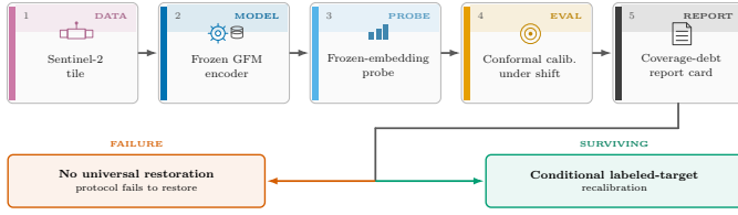
Fig. 1. Overview of the pre-deployment reliability report-card protocol. A Sentinel-2 tile (EuroSAT-MS / GEO-Bench BigEarthNet-S2 / m-so2sat) is passed through one of the frozen, interchangeable GFM encoders under audit (five illustrated: Prithvi, Clay, SSL4EO-DINO, SSL4EO-MAE, DOFA) and a frozen-embedding probe (logistic for the single-label tasks, multi-label otherwise), then conformally calibrated under the real geographic (region-transfer) shift—source split-conformal vs. spatial-Mondrian target-region calibration, source = E/Central Europe, target = W/Iberian-Atlantic Europe—yielding per-class conformal sets. The protocol reads off four practitioner-facing numbers for any frozen GFM: the in-distribution FNR guarantee, the geographic debt under shift, the target-slice repair cost, and the hidden worst-class coverage a marginal guarantee alone would miss. Vermillion marks the failure path (no universal restoration); bluish green marks the surviving path (conditional, encoder-dependent labeled-target recalibration).
