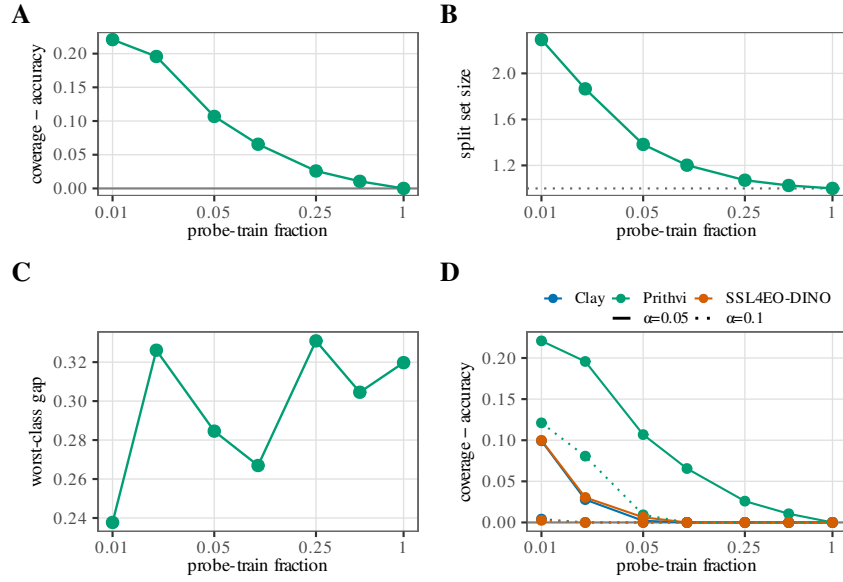
Figure 8: Singleton / low-shot validity boundary from the frozen EuroSAT low-shot sweep (no new runs). Panels (A)–(C) show the Prithvi series at \alpha=0.05 vs. probe-train fraction ( \log-x ). (A) Coverage–accuracy gap: as the budget rises, gap \rightarrow 0 and coverage collapses onto accuracy (degenerate regime). (B) Mean split set size on the same x -axis—a different quantity from (A), not a restatement of the gap; the dotted line at size = 1 is the singleton floor. (C) Worst-class coverage gap vs. fraction (conditional residual under the same sweep). (D) Multi-encoder comparison (Clay, Prithvi, SSL4EO-DINO): coverage–accuracy vs. fraction with colour = encoder and linestyle solid \alpha=0.05 / dotted \alpha=0.10 . Panels (A) and (B) are related through the singleton transition but are not redundant: gap measures coverage–accuracy decoupling, while set size measures how large the prediction sets become once that decoupling appears.
