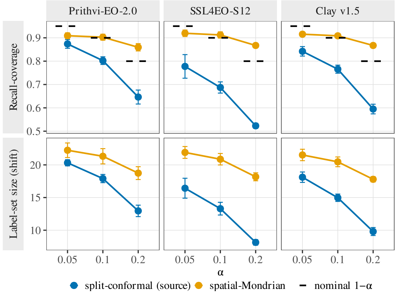
Fig. 13. Per-label multi-label conformal on GEO-Bench (26) m-bigearthnet (BigEarthNet-S2; 27 active labels after per-split filtering; real geographic E→W shift). Columns are frozen encoders; rows are (top) mean per-label recall-coverage \Pr(c \in \mathcal{C}(x) \mid y_c = 1) and (bottom) mean predicted label-set size per tile. Blue = source-only split-conformal; orange = target-side spatial-Mondrian; \alpha \in \{0.05, 0.10, 0.20\} . Short black dashed segments in the top row are nominal 1 - \alpha guides (legend: “nominal 1 - \alpha ”), not error bars; vertical whiskers on the points are seed-level Student t intervals ( n=5 ). Mondrian restores per-label coverage at \alpha \in \{0.10, 0.20\} (paired CI across labels excludes 0) for all three FMs. Relative to the dominant-label proxy, this per-label analysis is primary: it supplies independent per-class recall guarantees rather than a single-label reduction.
