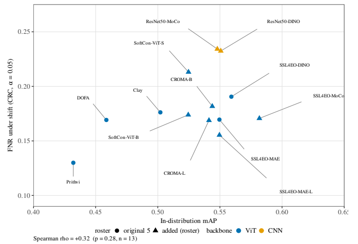
Fig. 4. The five-encoder inversion does not survive expansion to thirteen. FNR under shift vs. in-distribution mAP on m-bigearthnet ( \alpha=0.05 , CRC arm); circles are the original five encoders, triangles the eight added at pull. The rank correlation is a weak, non-significant positive (Spearman = +0.32 , permutation p=0.28 , n=13 ; no trend line is drawn, since the correlation does not reach significance); accuracy never buys better FNR robustness, but the strong +0.90 inversion of the five-encoder slice regresses toward zero. Prithvi (least accurate) remains the most FNR-robust; the two ResNet50 CNNs are the most fragile at mid accuracy.
