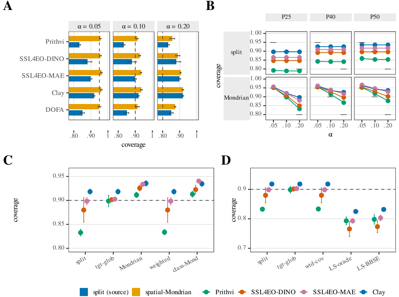
Fig. 10. Coverage restoration under real geographic shift (error bars = seed-level t -CIs, n=5 ; dashed = nominal 1 - \alpha ). (a) EuroSAT P_{33} : source split-conformal vs. spatial-Mondrian coverage by encoder and \alpha (five encoders, including DOFA). (b) Same split vs. Mondrian contrast at non- P_{33} spatial cuts (P25/P40/P50); row = arm, colour = encoder (four-encoder battery; DOFA absent from this frozen record). (c) Five conformal arms at \alpha=0.10 (ticks: split, tgt-glob, Mondrian, weighted, class-Mond). (d) Label-shift controls at \alpha=0.10 (ticks: split, tgt-glob, wtd-cov, LS-oracle, LS-BBSE). Spatial-Mondrian restores where debt exists; DOFA's shifted split coverage is 0.851 at every \alpha and spatial-Mondrian lifts it to 0.951/0.913/0.873.
