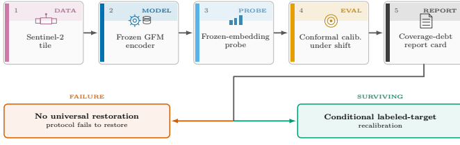
Fig. 1. Overview of the pre-deployment reliability report-card protocol. A Sentinel-2 tile (EuroSAT-MS / GEO-Bench BigEarthNet-S2 / m-so2sat) is passed through one of the frozen, interchangeable GFM encoders under audit (five illustrated: Prithvi, Clay, SSL4EO-DINO, SSL4EO-MAE, DOFA) and a frozen-embedding probe (logistic for the single-label tasks, multi-label otherwise), then conformally calibrated under the real geographic (region-transfer) shift—source split-conformal vs. spatial-Mondrian target-region calibration, source = E/Central Europe, target = W/Iberian-Atlantic Europe—yielding per-class conformal sets. The protocol reads off four practitioner-facing numbers for any frozen GFM: the in-distribution FNR guarantee, the geographic debt under shift, the target-slice repair cost, and the hidden worst-class coverage a marginal guarantee alone would miss. Vermillion marks the failure path (no universal restoration); bluish green marks the surviving path (conditional, encoder-dependent labeled-target recalibration).
