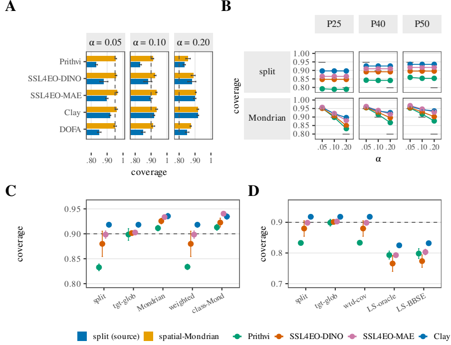
Figure 10: Coverage restoration under real geographic shift (error bars = seed-level t -CIs, n=5 ; dashed = nominal 1 - \alpha ). (a) EuroSAT P_{33} : source split-conformal vs. spatial-Mondrian coverage by encoder and \alpha (five encoders, including DOFA). (b) Same split vs. Mondrian contrast at non- P_{33} spatial cuts (P25/P40/P50); row = arm, colour = encoder (four-encoder battery; DOFA absent from this frozen record). (c) Five conformal arms at \alpha=0.10 (ticks: split, tgt-glob, Mondrian, weighted, class-Mond). (d) Label-shift controls at \alpha=0.10 (ticks: split, tgt-glob, wtd-cov, LS-oracle, LS-BBSE). Spatial-Mondrian restores where debt exists; DOFA’s shifted split coverage is 0.851 at every \alpha and spatial-Mondrian lifts it to 0.951/0.913/0.873.
