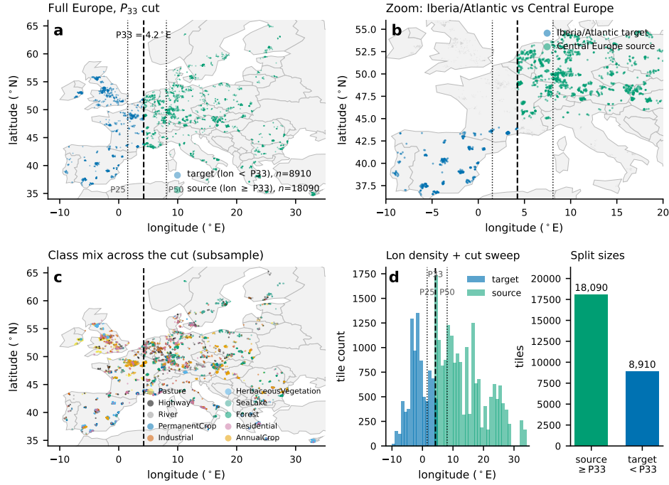
Figure 2: The geographic-shift construction on the map it is defined on (EuroSAT-MS centroids; frozen P_{33} cut = 4.2^\circ \text{E} ; source n=18,090 , target n=8,910 ). (a) Full-Europe scatter (4,000/27,000 seeded subsample) colored by split side, with P_{25}/P_{33}/P_{50} longitude guides. (b) Zoom contrasting Iberia/Atlantic target tiles against Central Europe source tiles around the cut. (c) Class-colored geographic mix (same cut; seeded subsample), showing land-cover labels present on both sides. (d) Longitude density with the same percentile guides, and the source/target tile counts. No image transform is applied — the shift is purely geographic.
