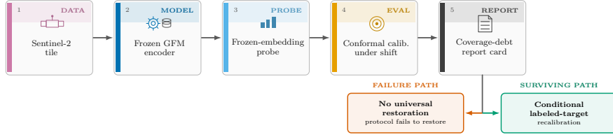
Figure 1: Overview of the pre-deployment reliability report-card protocol. Stages 1–5 (left to right): (1) optical Sentinel-2 tile (EuroSAT-MS / GEO-Bench BigEarthNet-S2 / m-so2sat); (2) one frozen, interchangeable optical GFM encoder under audit on EuroSAT/BigEarthNet (Prithvi, Clay, SSL4EO-DINO, SSL4EO-MAE, DOFA; on m-so2sat the ViT-S slot substitutes SSL4EO ViT-S/16 MAE for DINO—same five-encoder size , not an identical checkpoint roster); (3) frozen-embedding probe (logistic for single-label tasks, multi-label otherwise); (4) conformal calibration under real geographic region-transfer shift (source split-conformal vs. spatial-Mondrian target-region calibration; source = E/Central Europe, target = W/Iberian-Atlantic Europe), yielding per-class conformal sets; (5) coverage-debt report card with four practitioner-facing numbers—in-distribution FNR guarantee, geographic debt under shift, target-slice repair cost, and worst-class coverage a marginal guarantee alone would miss. Cross-sensor transfer (Sentinel-1) failed in-distribution control and is withheld. Fork from the report card: the protocol fails to restore coverage universally; the surviving path is conditional, encoder-dependent labeled-target recalibration.
