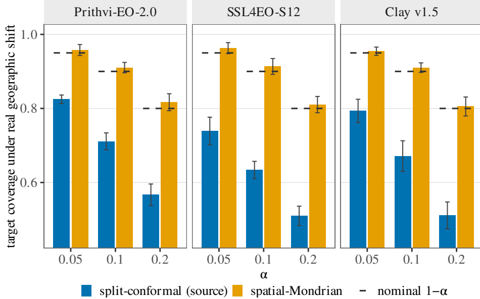
Figure 12: Dominant-label proxy on GEO-Bench m-bigearthnet : multi-hot BigEarthNet-S2 tiles reduced to the most frequent of 12 well-populated classes under a real geographic E→W shift (single-label LAC harness unchanged). Columns are the three frozen encoders (Prithvi-EO-2.0, SSL4EO-S12, Clay v1.5). Within each panel, blue bars are source-only split-conformal and orange bars are target-side spatial-Mondrian at \alpha \in \{0.05, 0.10, 0.20\} . Short black dashed segments mark the nominal coverage level 1 - \alpha at each \alpha (legend: “nominal 1 - \alpha ”); vertical whiskers on the bars are seed-level Student t intervals ( n=5 ), not the same mark. Coverage debt and Mondrian restoration replicate across all three encoders. This proxy is a coarse, qualitative replication; the per-label multi-label analysis in Fig. 13 is the primary BigEarthNet evidence.
