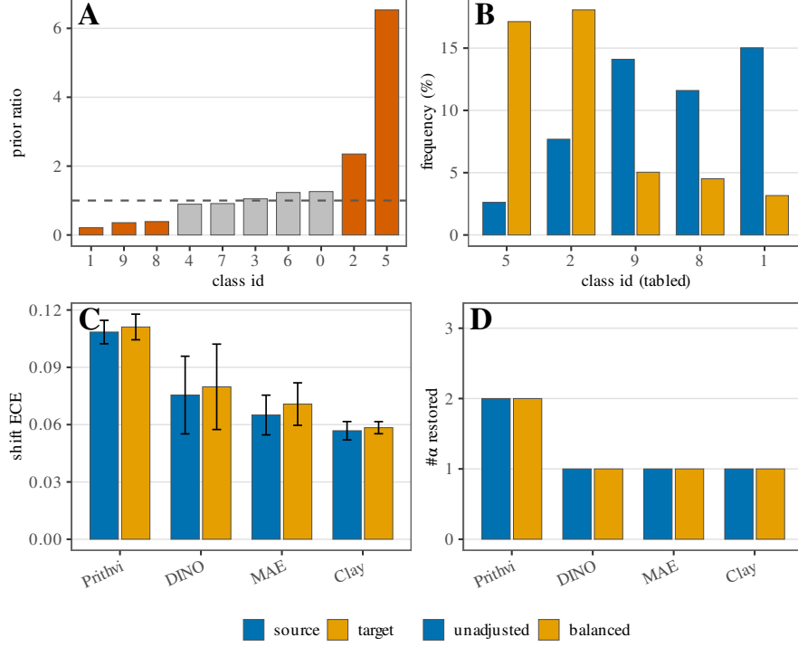
Figure 4: Class-prior / balanced-probe control at the frozen P_{33} cut (no new runs). A: target/source class-prior ratio by EuroSAT class id (orange = five tabled extremes; grey = others); dashed line at ratio 1 (no prior shift). B: source vs. target class frequency (%) for those five classes. C: shift ECE at \alpha=0.05 under the unadjusted (headline) vs. class-balanced probe; error bars are 5-seed t -CIs. D: count of \alpha \in \{0.05, 0.10, 0.20\} at which spatial-Mondrian restores coverage (CI excludes 0)—the “ \#\alpha repaired” count, not Mondrian coverage itself. Shared bottom legend: frequency (B) = source/target; probe (C–D) = unadjusted/balanced (same blue/orange hues, distinct meanings). Principle: the balanced probe is a control —encoder ranking by shift-ECE and repair counts should be stable if the P_{33} class-prior mismatch is not driving the finding.
