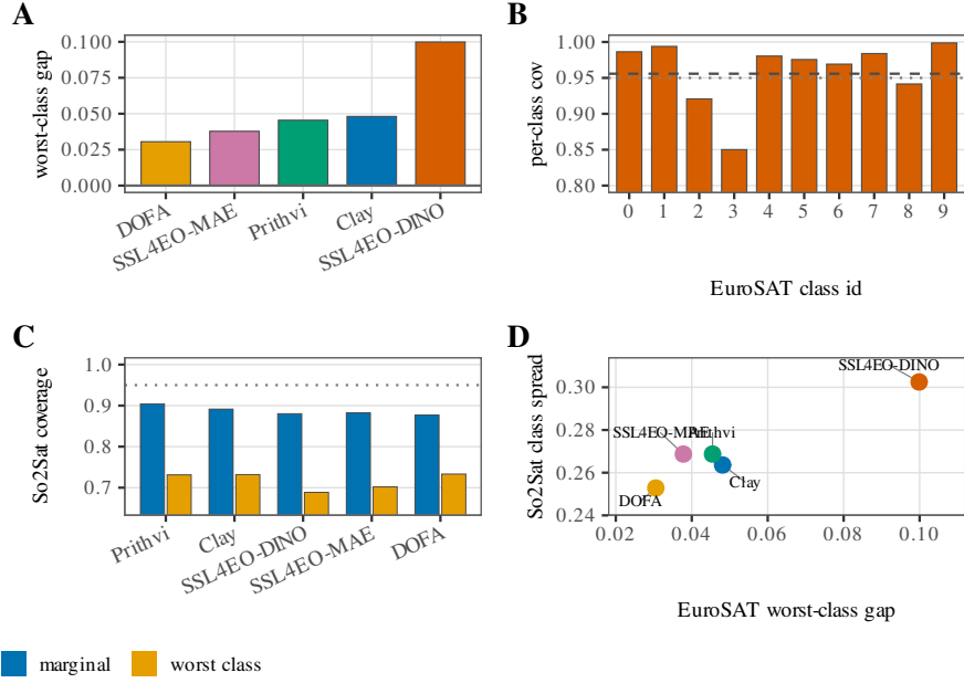
Figure 6: Conditional-coverage panels from the frozen EuroSAT and So2Sat roster summaries (Tables 4 and 11; no new runs; \alpha=0.05 ). (a) EuroSAT worst-class coverage gap G_{\text{worst}} by encoder (Okabe–Ito colours). (b) SSL4EO-DINO per-class conditional coverage on EuroSAT (dashed = encoder marginal; dotted = nominal 0.95). (c) So2Sat source-only split coverage by encoder: marginal (blue) vs. worst class (gold); dotted = nominal 0.95. (d) Encoder scatter of EuroSAT worst-class gap vs. So2Sat class-coverage spread (same encoder colours as (a)).
