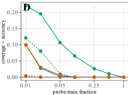
● Clay ● Prithvi ● SSL4EO-DINO — \alpha = 0.05 ... \alpha = 0.10
