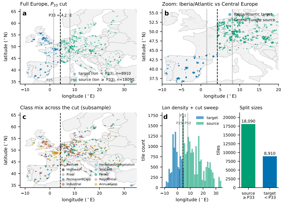
Figure 2: The geographic-shift construction on the map it is defined on (EuroSAT-MS centroids; frozen P_{33} cut = 4.2^\circ\text{E} ; source n=18,090 , target n=8,910 ). (a) Full-Europe scatter (4,000/27,000 seeded subsample) colored by split side, with P_{25}/P_{33}/P_{50} longitude guides. (b) Zoom contrasting Iberia/Atlantic target tiles against Central Europe source tiles around the cut. (c) Class-colored geographic mix (same cut; seeded subsample), showing land-cover labels present on both sides. (d) Longitude density with the same percentile guides, and the source/target tile counts. No image transform is applied — the shift is purely geographic.
