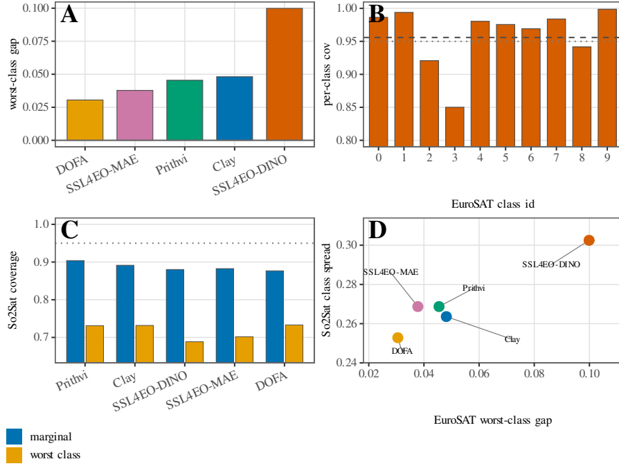
Figure 7: Conditional-coverage panels from the frozen EuroSAT and So2Sat roster summaries (Tables 4 and 11; no new runs; \alpha=0.05 ). (a) EuroSAT worst-class coverage gap G_{\text{worst}} by encoder (Okabe–Ito colours). (b) SSL4EO-DINO per-class conditional coverage on EuroSAT (dashed = encoder marginal; dotted = nominal 0.95). (c) So2Sat source-only split coverage by encoder: marginal (blue) vs. worst class (gold); dotted = nominal 0.95. (d) Encoder scatter of EuroSAT worst-class gap vs. So2Sat class-coverage spread (same encoder colours as (a)).
