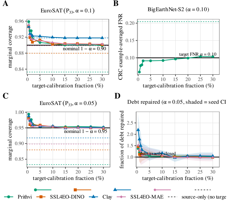
Figure 12: Target-recalibration planning curves: annotation budget versus guarantee tightness. (A) EuroSAT-MS ( P_{33} , \alpha=0.10 ): marginal coverage of the target-calibrated arm versus the labeled fraction of the target region (%). (B) GEO-Bench BigEarthNet-S2 ( \alpha=0.10 ): CRC example-averaged false-negative rate (FNR) on the same x -axis (Prithvi only; vacuous CRC budgets with \alpha < 1/(n_{\text{eff}}+1) omitted). (C) EuroSAT-MS at the stricter \alpha=0.05 , same coverage axes as (A). (D) Normalized EuroSAT reading at \alpha=0.05 : fraction of coverage debt repaired versus budget (shaded bands = five-seed intervals; values >1 are over-repair). Solid coloured curves are encoders; matching dashed horizontals are budget-independent source-only baselines (no target labels); black horizontals mark the nominal coverage 1-\alpha , target FNR \alpha , or exact debt clearance ( =1 in (D)). The repair is not a rising ramp: wherever debt exists, the smallest usable budget already clears the nominal level, after which curves converge onto it from the conservative side. That shape is finite-sample conformal correction—the effective quantile \lceil (n+1)(1-\alpha) \rceil / n inflates above 1-\alpha at small n (e.g. 0.932 vs. 0.900 at n=44 , \alpha=0.10 ), over-covering and paying for the slack in larger sets—so extra labels buy tightness to nominal, not validity of the guarantee. Descriptive secondary analysis (§5); So2Sat excluded (no local features).
