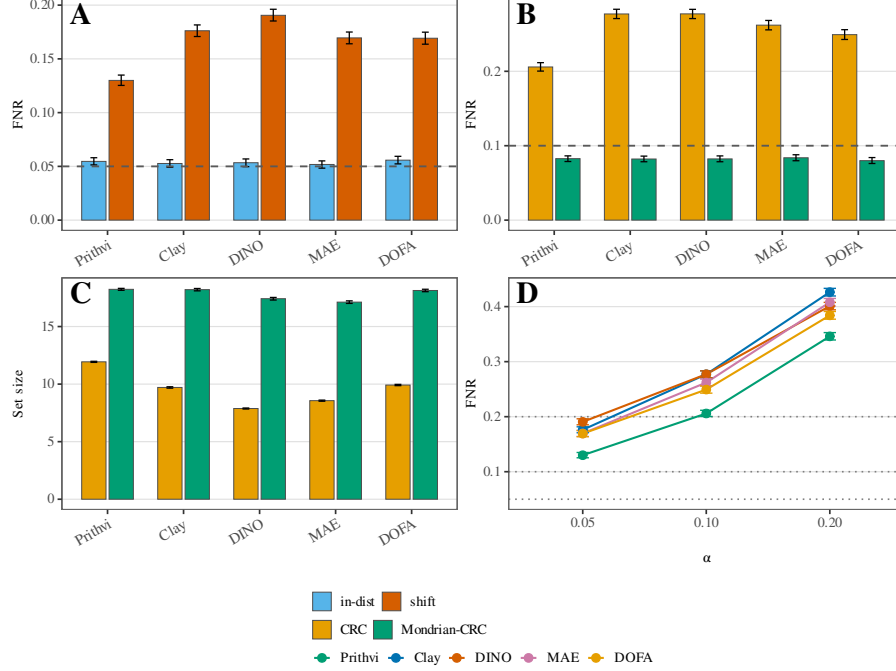
Figure 15: CRC on BigEarthNet (Table 9; frozen multi-seed bootstrap means with 95% CIs; no new runs). All panels use example-averaged FNR (or set size) of Eqs. (10)–(11) pooled over five seeds; error bars are percentile bootstrap intervals ( B=2000 ). Encoder ticks and the panel-(d) colour key abbreviate SSL4EO-DINO/MAE as DINO/MAE. (a) Source-calibrated CRC FNR in-distribution vs. under the E→W geographic shift at \alpha=0.05 (blue = in-dist, vermillion = shift; dashed = nominal FNR level \alpha ). In-distribution meets the risk level; the same \hat{\lambda} incurs large FNR debt under shift. (b) Shift FNR at \alpha=0.10 : source-calibrated CRC vs. target-side Mondrian-CRC (blue/green; dashed = nominal \alpha ). Mondrian-CRC restores FNR to at-or-below nominal for every encoder. (c) Mean set-size cost under shift at the same \alpha=0.10 (labels/tile of \sim 27 active; Eq. (4)): Mondrian-CRC’s restore comes with larger sets than source-calibrated CRC (shared method colours with (b)). (d) Source-calibrated CRC FNR under shift across \alpha \in \{0.05, 0.10, 0.20\} by encoder (coloured lines; dotted horizontals = nominal \alpha at each risk level).
