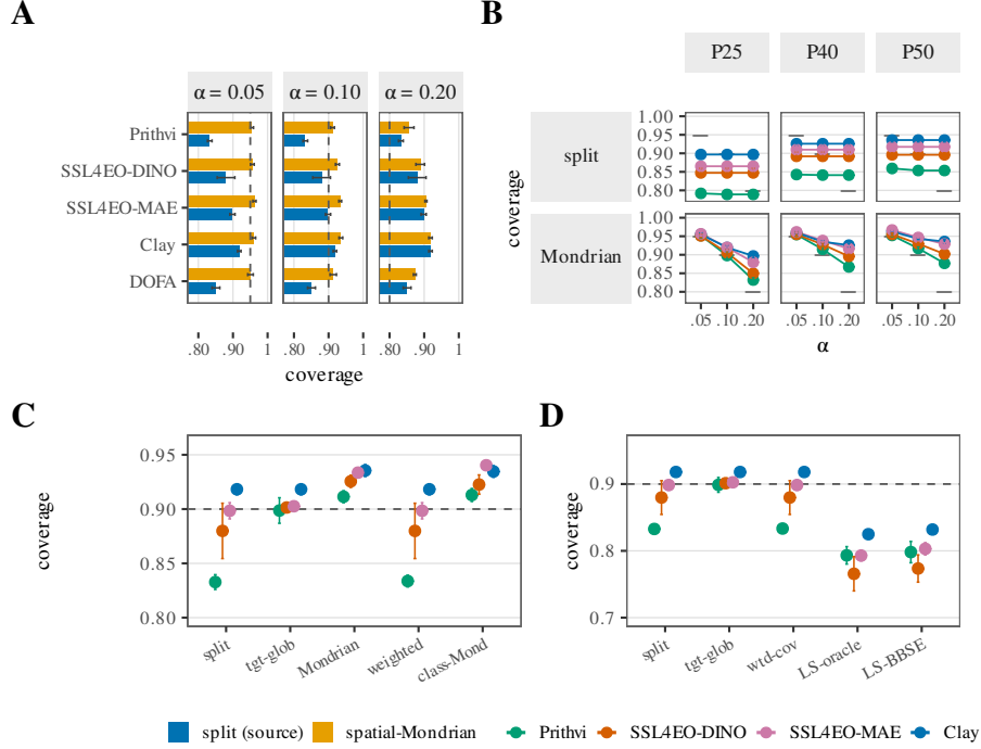
Figure 11: Coverage restoration under real geographic shift (error bars = seed-level t -CIs, n=5 ; dashed = nominal 1 - \alpha ). (a) EuroSAT P_{33} : source split-conformal vs. spatial-Mondrian coverage by encoder and \alpha (five encoders, including DOFA). (b) Same split vs. Mondrian contrast at non- P_{33} spatial cuts (P25/P40/P50); row = arm, colour = encoder (four-encoder battery; DOFA absent from this frozen record). (c) Five conformal arms at \alpha=0.10 (ticks: split, tgt-glob, Mondrian, weighted, class-Mond). (d) Label-shift controls at \alpha=0.10 (ticks: split, tgt-glob, wtd-cov, LS-oracle, LS-BBSE). Spatial-Mondrian restores where debt exists; DOFA’s shifted split coverage is 0.851 at every \alpha and spatial-Mondrian lifts it to 0.951/0.913/0.873.
