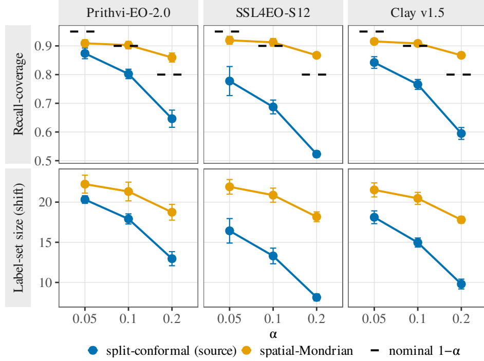
Figure 14: Per-label multi-label conformal on GEO-Bench (Lacoste et al., 2023) m-bigearthnet (BigEarthNet-S2; 27 active labels after per-split filtering; real geographic E \rightarrow W shift). Columns are frozen encoders; rows are (top) mean per-label recall-coverage \Pr(c \in \mathcal{C}(x) \mid y_c = 1) (Eq. (9)) and (bottom) mean predicted label-set size per tile. Blue = source-only split-conformal; orange = target-side spatial-Mondrian; \alpha \in \{0.05, 0.10, 0.20\} . Short black dashed segments in the top row are nominal 1 - \alpha guides (legend: “nominal 1 - \alpha ”), not error bars; vertical whiskers on the points are seed-level Student t intervals ( n=5 ). Mondrian restores per-label coverage at \alpha \in \{0.10, 0.20\} (paired CI across labels excludes 0) for all three FMs. Relative to the dominant-label proxy of Fig. 13, this per-label analysis is primary: it supplies independent per-class recall guarantees rather than a single-label reduction.
