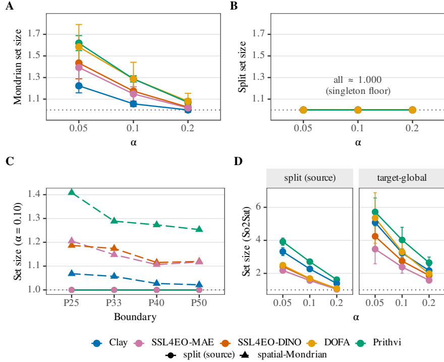
Figure 8: Four-panel set-size cost of restoration (error bars seed-level t -CIs, n=5 ; dotted line = singleton floor of set size 1). Shared encoder colours throughout; panel (c) uses linetype/shape for split vs. spatial-Mondrian. (a) EuroSAT spatial-Mondrian mean set size vs. \alpha (rises above the floor only where Mondrian repays coverage debt; DOFA 1.58/1.29/1.08 at \alpha = 0.05/0.10/0.20 ). (b) Source split-conformal set size on the same y -scale as (a): every encoder sits on the singleton floor ( \approx 1.000 ), so the excess size in (a) is the restoration cost. (c) Set size vs. spatial boundary percentile at \alpha=0.10 (solid = source split; dashed = spatial-Mondrian). (d) So2Sat LCZ (17 classes) source-split vs. target-global set size in side-by-side facets—larger absolute sets than EuroSAT, on its own y -scale.
