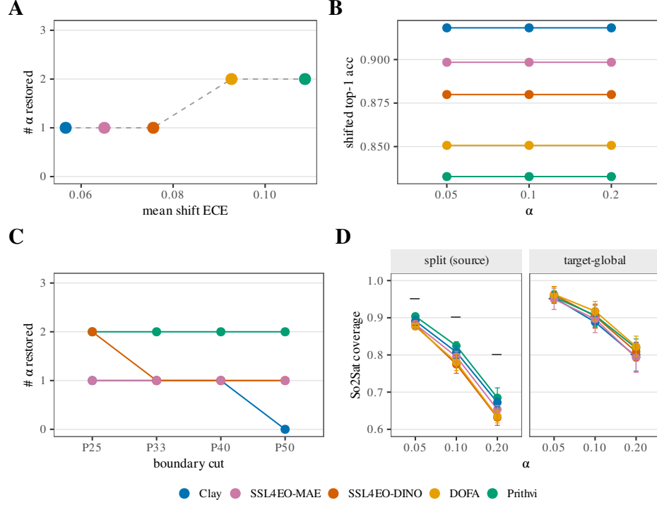
Figure 10: Four-panel coverage-debt diagnostic across five frozen encoders (shared colour legend: Clay, SSL4EO-MAE, SSL4EO-DINO, DOFA, Prithvi). (A) Mean in-shift ECE (coverage debt) vs. the number of risk levels \alpha \in \{0.05, 0.10, 0.20\} where spatial-Mondrian restores target coverage—i.e. the paired gap CI excludes 0 in the positive direction. Debt orders Prithvi > DOFA > SSL4EO-DINO > SSL4EO-MAE > Clay; repair counts are weakly monotone (Prithvi = DOFA 2, others 1). (B) Shifted top-1 accuracy vs. \alpha (flat across risk levels; ranking matches debt). (C) Boundary-sweep check on the four battery encoders (DOFA absent from that frozen sweep): # \alpha restored at spatial cuts P25–P50. (D) So2Sat LCZ cross-continent label-access check: source-split vs. target-global coverage (facets), with grey ticks marking nominal 1 - \alpha and error bars seed-level CIs. Set-size cost of repair is in Fig. 8.
