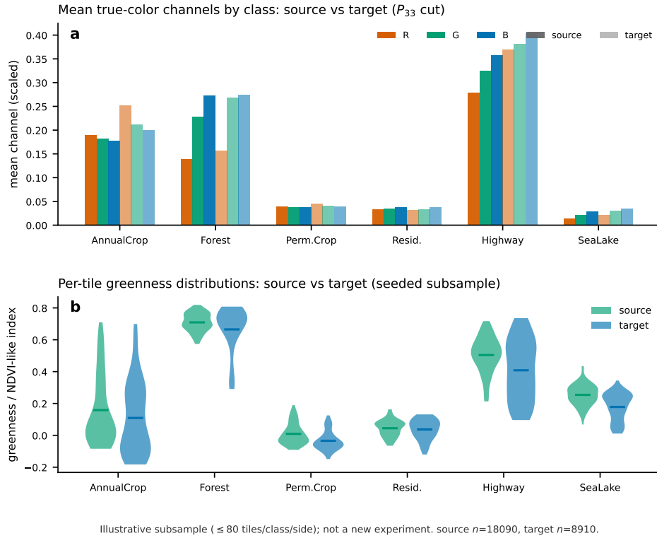
Figure 4: Spectral fingerprint of the same geographic cut (frozen local tiles keyed to the MS manifest; seeded subsample, not a new experiment). (a) Per-class mean true-color channels on the source vs. target side of P_{33} . (b) Per-tile greenness / NDVI-like index distributions by class and side (MS: (B_{08} - B_{04}) / (B_{08} + B_{04}) ; RGB fallback: (G - R) / (G + R) ). This panel is geographic-shift visualization only; class-prior mass shift is already shown in Fig. 5.
