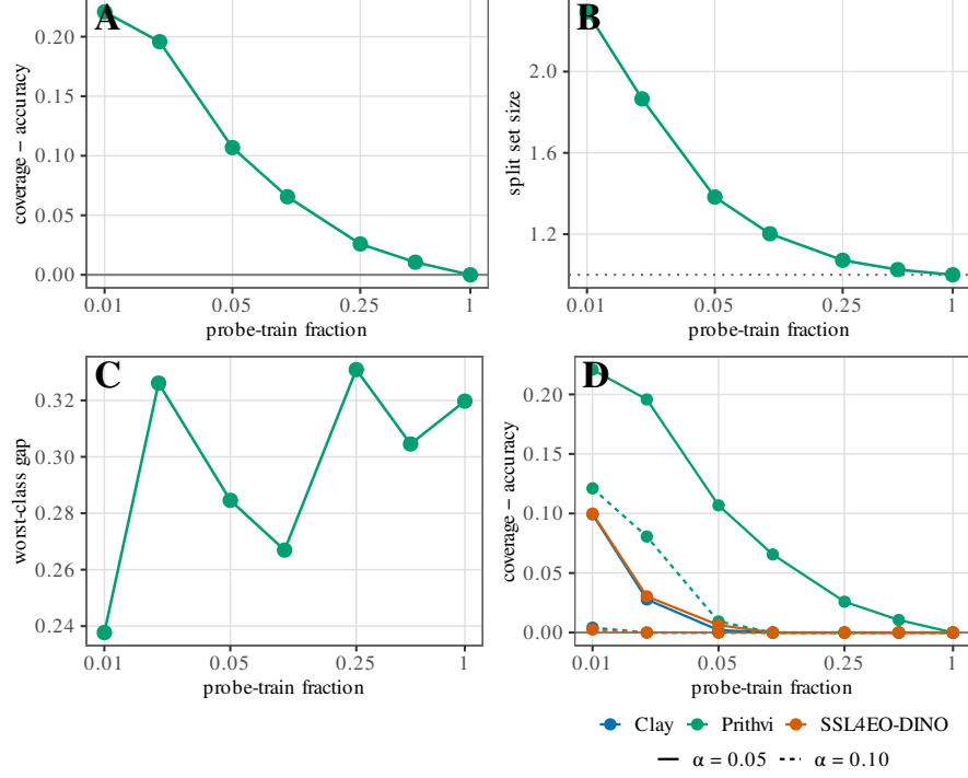
Figure 9: Singleton / low-shot validity boundary from the frozen EuroSAT low-shot sweep (Table 5; no new runs). Panels (a)–(c) show the Prithvi series at \alpha=0.05 vs. probe-train fraction ( \log x ). (a) Coverage–accuracy gap: as the budget rises, gap \rightarrow 0 and coverage collapses onto accuracy (degenerate regime). (b) Mean split set size on the same x -axis—a different quantity from (a), not a restatement of the gap; the dotted line at size = 1 is the singleton floor. (c) Worst-class coverage gap vs. fraction (conditional residual under the same sweep). (d) Multi-encoder comparison (Clay, Prithvi, SSL4EO-DINO): coverage–accuracy vs. fraction with colour = encoder and linestyle solid \alpha=0.05 / dotted \alpha=0.10 . Panels (a) and (b) are related through the singleton transition but are not redundant: gap measures coverage–accuracy decoupling, while set size measures how large the prediction sets become once that decoupling appears.
