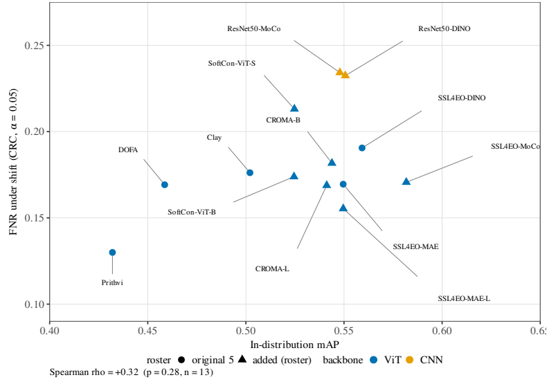
Figure 6: The five-encoder inversion does not survive expansion to thirteen. FNR under shift vs. in-distribution mAP on m-bigearthnet ( \alpha=0.05 , CRC arm); circles are the original five encoders, triangles the eight added at pull. The rank correlation is a weak, non-significant positive (Spearman +0.32, permutation p=0.28 , n=13 ; no trend line is drawn, since the correlation does not reach significance): accuracy never buys better FNR robustness, but the strong +0.90 inversion of the five-encoder slice regresses toward zero. Prithvi (least accurate) remains the most FNR-robust; the two ResNet50 CNNs are the most fragile at mid accuracy.
