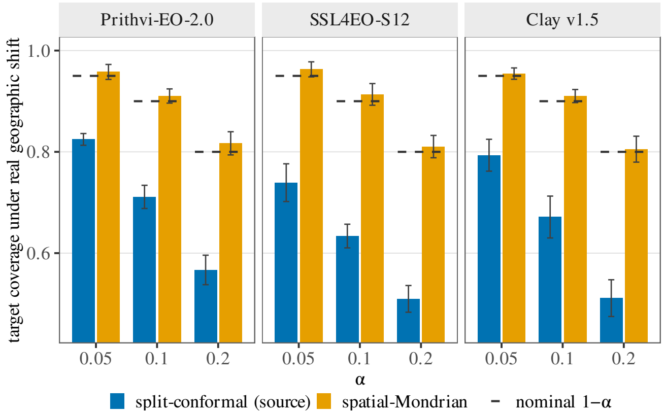
Fig. 12. Dominant-label proxy on GEO-Bench m-bigearthnet (single-label reduction; 12 classes): coverage debt and spatial-Mondrian restoration replicate across all three frozen FMs (dashed = nominal 1 - \alpha ; error bars seed-level t -CIs, n=5 ). A coarse, qualitative replication; the per-label analysis of Fig. 13 is primary.
