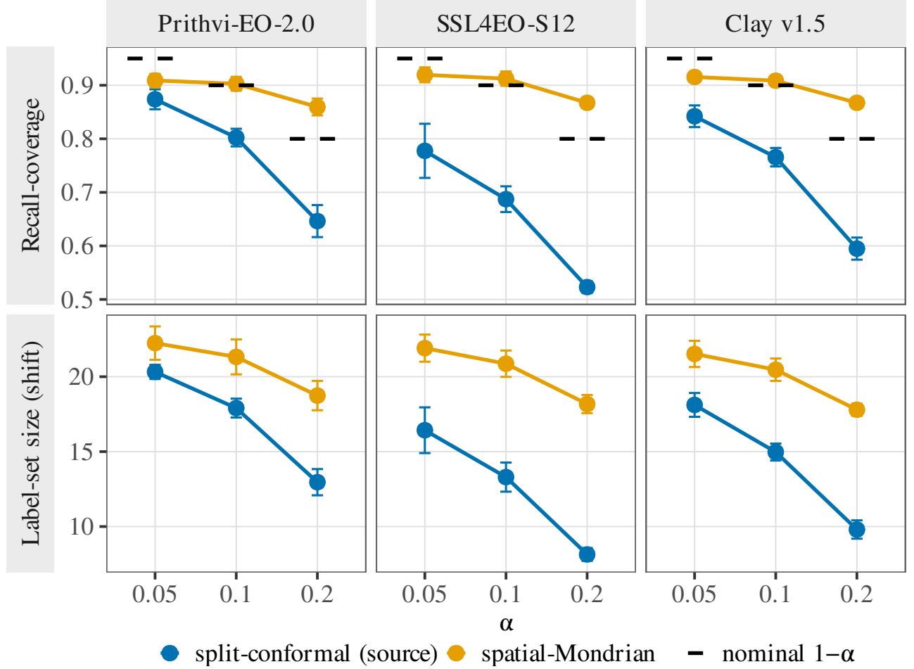
Fig. 13. Per-label multi-label conformal on GEO-Bench (26) m-bigearthnet (BigEarthNet-S2; 27 active labels; real geographic E→W shift; 5 seeds). Top: mean per-label recall-coverage \Pr(c \in \mathcal{C}(x) \mid y_c = 1) for source split-conformal and target-side spatial-Mondrian per FM and \alpha (dash = 1 - \alpha ). Bottom: mean predicted label-set size per tile. Mondrian restores per-label coverage at \alpha \in \{0.10, 0.20\} (paired CI across labels excludes 0) for all three FMs, confirming coverage debt in a rigorous multi-label setting.
