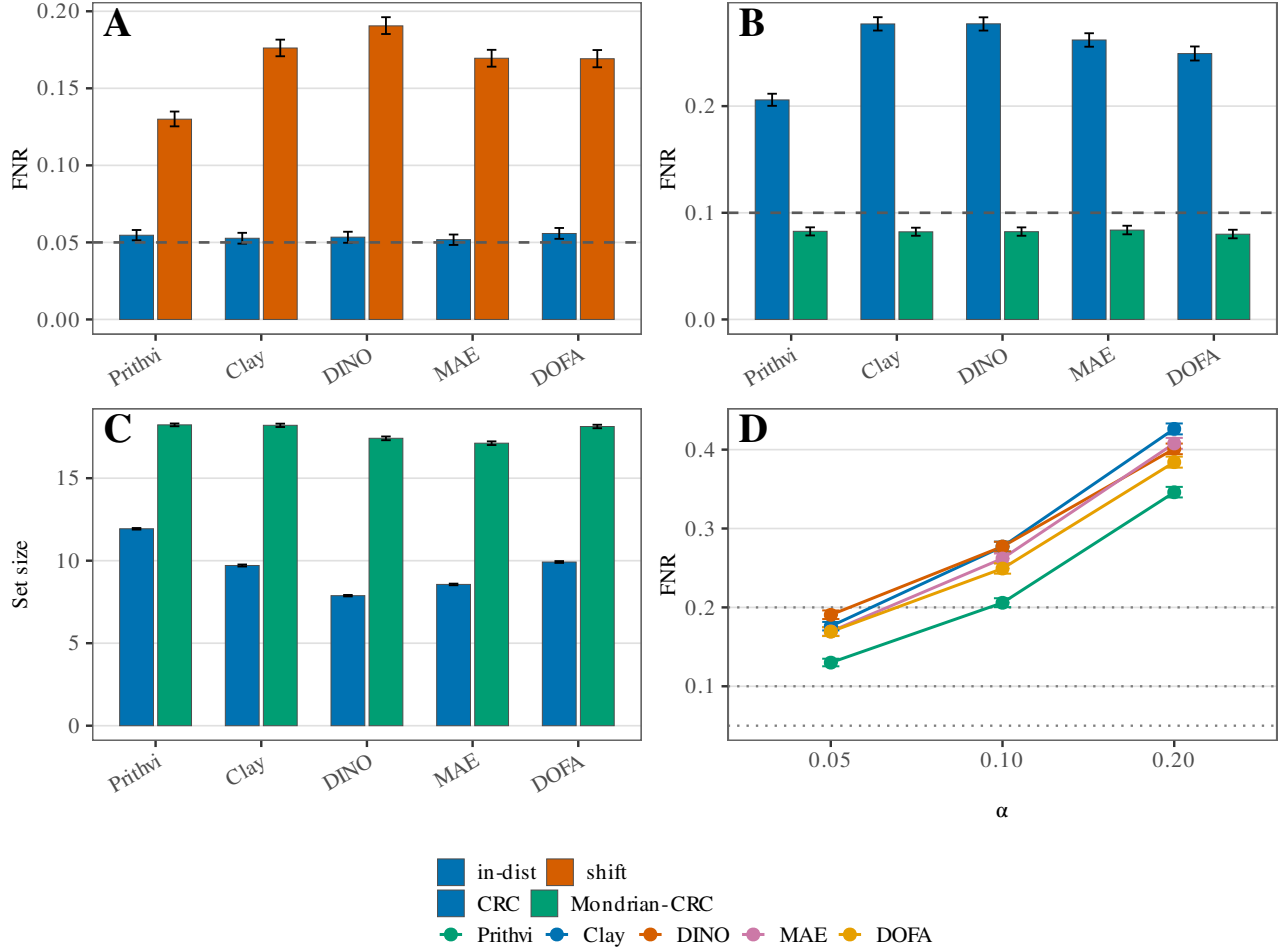
Fig. 8. CRC on BigEarthNet (Table VI; frozen multi-seed bootstrap means with 95% CIs; no new runs). All panels use example-averaged FNR (or set size) pooled over five seeds; error bars are percentile bootstrap intervals ( B=2000 ). Encoder ticks and the panel-(d) colour key abbreviate SSL4EO-DINO/MAE as DINO/MAE. (a) Source-calibrated CRC FNR in-distribution vs. under the E \rightarrow W geographic shift at \alpha=0.05 (blue = in-dist, vermillion = shift; dashed = nominal \alpha ). In-distribution meets the risk level; the same \lambda incurs large FNR debt under shift. (b) Shift FNR at \alpha=0.10 : source-calibrated CRC vs. target-side Mondrian-CRC (blue/green; dashed = nominal \alpha ). Mondrian-CRC restores FNR to at-or-below nominal for every encoder. (c) Mean set-size cost under shift at the same \alpha=0.10 (labels/tile of \sim 27 active): Mondrian-CRC's restore comes with larger sets than source-calibrated CRC (shared method colours with (b)). (d) Source-calibrated CRC FNR under shift across \alpha \in \{0.05, 0.10, 0.20\} by encoder (coloured lines; dotted horizontals = nominal \alpha at each risk level).
