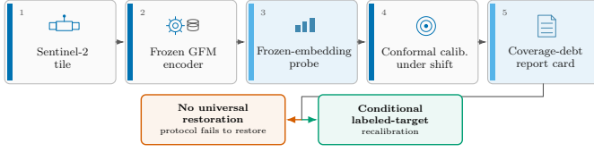
Fig. 1. Overview of the pre-deployment reliability report-card protocol (§IV-B, Table XI). A Sentinel-2 tile (EuroSAT-MS / GEO-Bench BigEarthNet-S2 / m-so2sat) is passed through one of the frozen, interchangeable GFM encoders under audit (five illustrated: Prithvi, Clay, SSL4EO-DINO, SSL4EO-MAE, DOFA) and a frozen-embedding probe (logistic for the single-label tasks, multi-label otherwise), then conformally calibrated under the real geographic (region-transfer) shift—source split-conformal vs. spatial-Mondrian target-region calibration, source = E/Central Europe, target = W/Iberian-Atlantic Europe—yielding per-class conformal sets. The protocol reads off four practitioner-facing numbers for any frozen GFM: the in-distribution FNR guarantee, the geographic debt under shift, the target-slice repair cost, and the hidden worst-class coverage a marginal guarantee alone would miss. The protocol fails to restore coverage universally; the surviving path is conditional, encoder-dependent labeled-target recalibration (§V).
