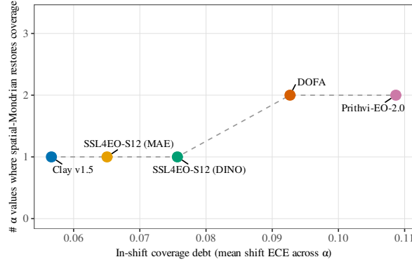
Figure 5: Encoder-dependent coverage debt (mean shift ECE) vs. the number of risk levels spatial-Mondrian conformal restores, for all five frozen encoders. Debt orders Prithvi > DOFA > SSL4EO-DINO > SSL4EO-MAE > Clay; repair count is weakly monotone (Prithvi = DOFA 2; SSL4EO-DINO = SSL4EO-MAE = Clay 1), and the repair magnitude (Fig. 7) is monotone in debt. The five frozen encoders comprise the four-encoder battery plus the corrected DOFA fifth-encoder block.
