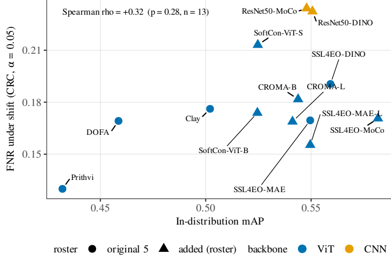
Figure 4: The five-encoder inversion does not survive expansion to thirteen. FNR under shift vs. in-distribution mAP on m-bigeearthnet ( \alpha=0.05 , CRC arm); circles are the original five encoders, triangles the eight added at pull. The rank correlation is a weak, non-significant positive (Spearman = +0.32, permutation p=0.28 , n=13 ; no trend line is drawn, since the correlation does not reach significance): accuracy never buys better FNR robustness, but the strong +0.90 inversion of the five-encoder slice regresses toward zero. Prithvi (least accurate) remains the most FNR-robust; the two ResNet50 CNNs are the most fragile at mid accuracy.
