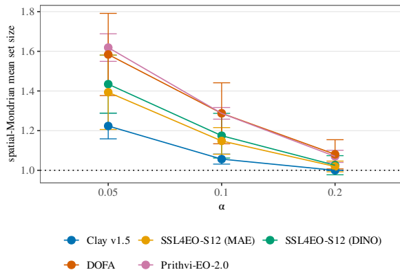
Figure 7: Restoration is paid in prediction-set size: spatial-Mondrian set size exceeds the split-conformal singleton baseline (dotted line at set size 1) only where it repays coverage debt, across all five frozen encoders (roster as in Fig. 5; DOFA’s set size 1.58/1.29/1.08 at \alpha = 0.05/0.10/0.20 ). Error bars are seed-level t -CIs ( n=5 ).
