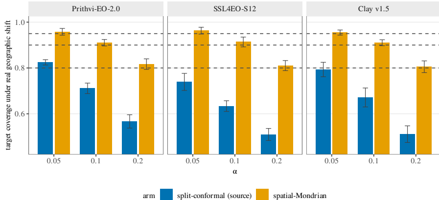
Figure 8: Dominant-label proxy on GEO-Bench m-bigeearthnet (single-label reduction; 12 classes): coverage debt and spatial-Mondrian restoration replicate across all three frozen FMs (dashed = nominal 1 - \alpha ; error bars seed-level t -CIs, n=5 ). A coarse, qualitative replication; the per-label analysis of Fig. 9 is primary.
