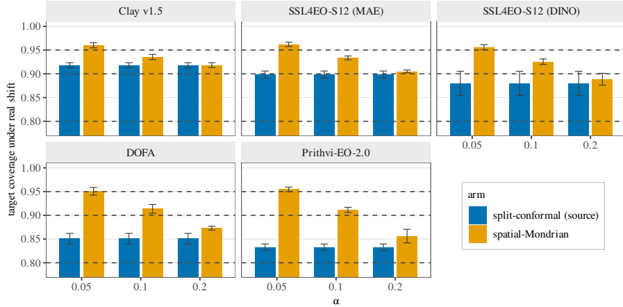
Figure 6: Target coverage under real shift: source split-conformal (under-covers) vs. spatial-Mondrian, per encoder and \alpha (dashed = nominal 1 - \alpha ; error bars seed-level t -CIs, n=5 ), for all five frozen encoders (roster as in Fig. 5). Restoration occurs where debt exists; DOFA’s shifted split coverage is 0.851 at every \alpha and spatial-Mondrian lifts it to 0.951/0.913/0.873.
