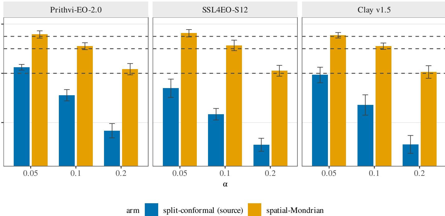
target coverage under real geographic shift
