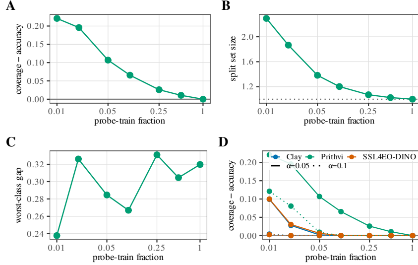
Figure 8: Singleton / low-shot validity boundary from the frozen EuroSAT low-shot sweep (no new runs). Panels (A)–(C) show the Prithvi series at \alpha=0.05 vs. probe-train fraction (log- x ). (A) Coverage–accuracy gap: as the budget rises, gap \rightarrow 0 and coverage collapses onto accuracy (degenerate regime). (B) Mean split set size on the same x -axis—a different quantity from (A), not a restatement of the gap; the dotted line at size = 1 is the singleton floor. (C) Worst-class coverage gap vs. fraction (conditional residual under the same sweep). (D) Multi-encoder comparison (Clay, Prithvi, SSL4EO-DINO): coverage–accuracy vs. fraction with colour = encoder and linestyle solid \alpha=0.05 / dotted \alpha=0.10 . Panels (A) and (B) are related through the singleton transition but are not redundant: gap measures coverage–accuracy decoupling, while set size measures how large the prediction sets become once that decoupling appears.
