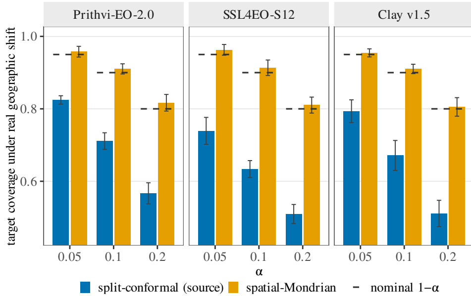
Figure 12: Dominant-label proxy on GEO-Bench m-bigearthnet : multi-hot BigEarthNet-S2 tiles reduced to the most frequent of 12 well-populated classes under a real geographic E \rightarrow W shift (single-label LAC harness unchanged). Columns are the three frozen encoders (Prithvi-EO-2.0, SSL4EO-S12, Clay v1.5). Within each panel, blue bars are source-only split-conformal and orange bars are target-side spatial-Mondrian at \alpha \in \{0.05, 0.10, 0.20\} . Short black dashed segments mark the nominal coverage level 1 - \alpha at each \alpha (legend: “nominal 1 - \alpha ”); vertical whiskers on the bars are seed-level Student t intervals ( n=5 ), not the same mark. Coverage debt and Mondrian restoration replicate across all three encoders. This proxy is a coarse, qualitative replication; the companion per-label multi-label analysis is the primary BigEarthNet evidence.
