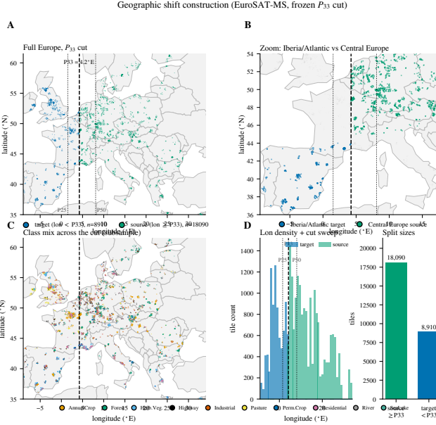
Figure 2: The geographic-shift construction on the map it is defined on (EuroSAT-MS centroids; frozen P_{33} cut = 4.2^\circ\text{E} ; source n=18,090 , target n=8,910 ). (a) Full-Europe scatter (4,000/27,000 seeded subsample) colored by split side, with P_{25}/P_{33}/P_{50} longitude guides. (b) Zoom contrasting Iberia/Atlantic target tiles against Central Europe source tiles around the cut. (c) Class-colored geographic mix (same cut; seeded subsample), showing land-cover labels present on both sides. (d) Longitude density with the same percentile guides, and the source/target tile counts. No image transform is applied — the shift is purely geographic.
