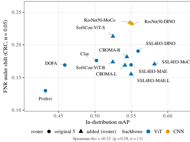
Fig. 4. The five-encoder inversion does not survive expansion to thirteen. FNR under shift vs. in-distribution mAP on BigEarthNet ( \alpha=0.05 , CRC arm); circles are the original five encoders, triangles the eight added at pull. The rank correlation is a weak, non-significant positive ( \text{Spearman} = +0.32 , permutation p=0.28 , n=13 ; no trend line is drawn, since the correlation does not reach significance): accuracy never buys better FNR robustness, but the strong +0.90 inversion of the five-encoder slice regresses toward zero. Prithvi (least accurate) remains the most FNR-robust; the two ResNet50 CNNs are the most fragile at mid accuracy.
