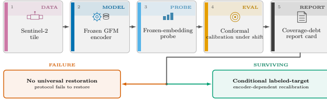
Fig. 1. Overview of the pre-deployment reliability report-card protocol. A Sentinel-2 tile (EuroSAT-MS / GEO-Bench BigEarthNet-S2 / So2Sat LCZ42) is passed through one of the frozen, interchangeable GFM encoders under audit (five illustrated: Prithvi, Clay, SSL4EO-DINO, SSL4EO-MAE, DOFA) and a frozen-embedding probe (logistic for the single-label tasks, multi-label otherwise), then conformally calibrated under the real geographic (region-transfer) shift—source split-conformal vs. spatial-Mondrian target-region calibration, source = E/Central Europe, target = W/Iberian-Atlantic Europe—yielding per-class conformal sets. The protocol reads off four practitioner-facing numbers for any frozen GFM: the in-distribution FNR guarantee, the geographic debt under shift, the target-slice repair cost, and the hidden worst-class coverage a marginal guarantee alone would miss. Stages 1–5 are role-tagged DATA / MODEL / PROBE / EVAL / REPORT. Vermillion marks FAILURE (no universal restoration); bluish green marks SURVIVING (conditional, encoder-dependent labeled-target recalibration).
