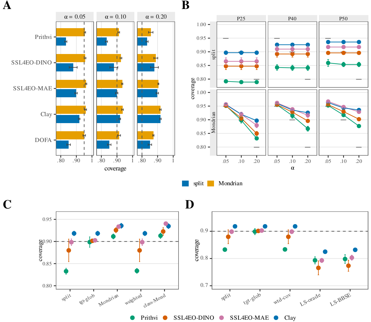
Fig. 10. Coverage restoration under real geographic shift (error bars = seed-level t -CIs, n=5 ; dashed = nominal 1 - \alpha ). (a) EuroSAT P_{33} : source split-conformal vs. spatial-Mondrian coverage by encoder and \alpha (five encoders, including DOFA). (b) Same split vs. Mondrian contrast at non- P_{33} spatial cuts (P25/P40/P50); row = arm, colour = encoder (four-encoder battery; DOFA absent from this frozen record). (c) Five conformal arms at \alpha=0.10 (ticks: split, tgt-glob, Mondrian, weighted, class-Mond). (d) Label-shift controls at \alpha=0.10 (ticks: split, tgt-glob, wtd-cov, LS-oracle, LS-BBSE). Spatial-Mondrian restores where debt exists; DOFA's shifted split coverage is 0.851 at every \alpha and spatial-Mondrian lifts it to 0.951/0.913/0.873.
