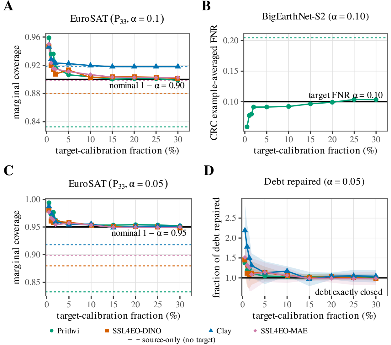
Fig. 7. Target-recalibration planning curves: annotation budget versus guarantee tightness. (A) EuroSAT-MS ( P_{33} , \alpha=0.10 ): marginal coverage of the target-calibrated arm versus the labeled fraction of the target region (%). (B) GEO-Bench BigEarthNet-S2 ( \alpha=0.10 ): CRC example-averaged false-negative rate (FNR) on the same x -axis (Prithvi only; vacuous CRC budgets with \alpha < 1/(n_{\text{eff}}+1) omitted). (C) EuroSAT-MS at the stricter \alpha=0.05 , same coverage axes as (A). (D) Normalized EuroSAT reading at \alpha=0.05 : fraction of coverage debt repaired versus budget (shaded bands = five-seed intervals; values >1 are over-repair). Solid coloured curves are the four encoders. Matching coloured dashed horizontals are source-only (no target labels) baselines, independent of the annotation budget. Solid black horizontals are the design targets: nominal coverage 1-\alpha in (A) and (C), and exact debt clearance ( =1 ) in (D). The repair is not a rising ramp: wherever debt exists, the smallest usable budget already clears the nominal level, after which curves converge onto it from the conservative side. That shape is finite-sample conformal correction—the effective quantile \lceil (n+1)(1-\alpha) \rceil / n inflates above 1-\alpha at small n (e.g. 0.932 vs. 0.900 at n=44 , \alpha=0.10 ), over-covering and paying for the slack in larger sets—so extra labels buy tightness to nominal, not validity of the guarantee. Descriptive secondary analysis; So2Sat excluded (no local features).
