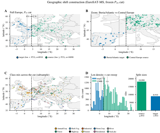
Fig. 2. The geographic-shift construction, shown on the map it is defined on: EuroSAT-MS tile centroids (4,000 of 27,000, seeded subsample) colored by split side at the P_{33} longitude cut ( = 4.2^\circ\text{E} ; P_{25}/P_{50} sweep boundaries dotted). Source tiles (E/Central Europe, n=18,090 ) calibrate; target tiles (W/Iberian-Atlantic Europe, n=8,910 ) are the deployment region. No image transform is applied — the shift is purely geographic.
