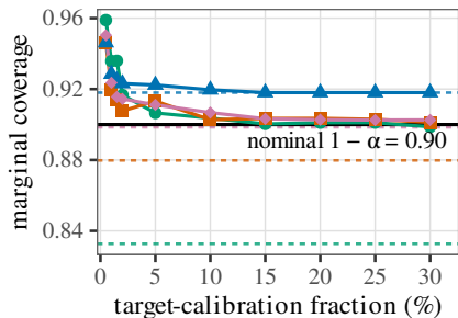
EuroSAT ( P_{33} , \alpha = 0.1 )
