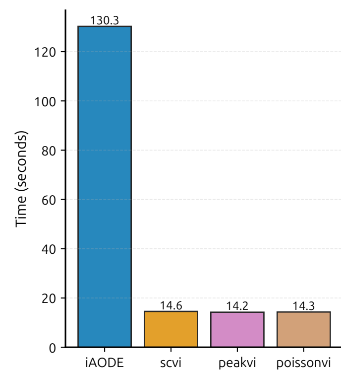
D. Training Time
