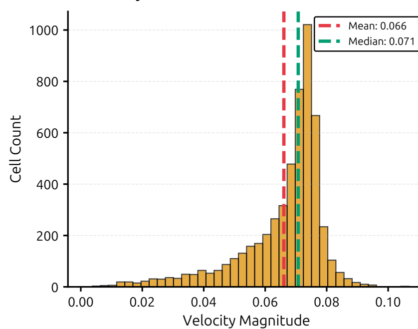
G. Velocity Distribution
