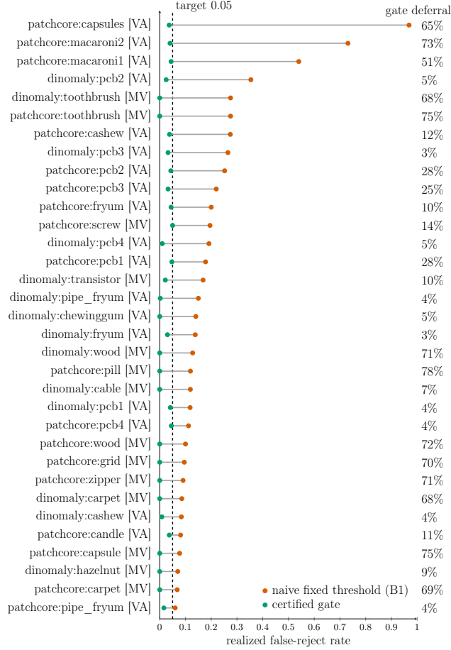
Figure 12: Binding cells on the false-reject axis (post-hoc). Same encoding as the escaped-defect binding figure; the dashed line is the \alpha_{fr} = 0.05 target. The VisA PatchCore capsules cell (top) is the extreme case: a global threshold auto-rejects 96.8% of good parts where the certified gate holds 3.7%.
