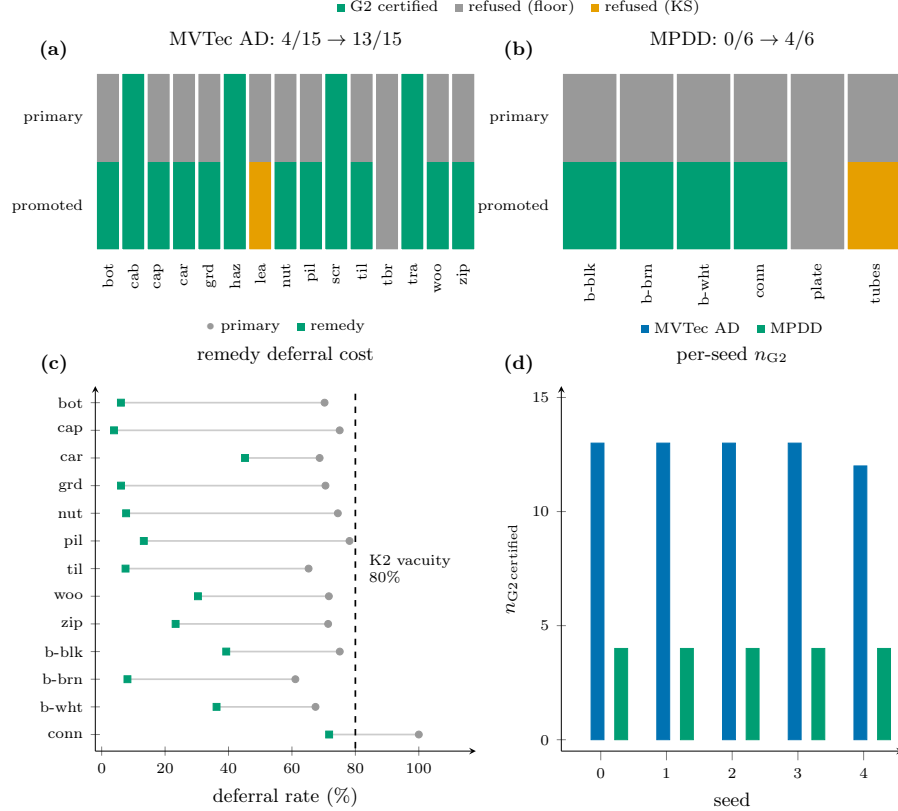
Figure 10: The G2 train-holdout remedy (PatchCore; seeds 0–3 identical, seed 4 differs on screw). a: MVTec AD: 4/15 \rightarrow 13/15 , leather KS-refused every seed. b: MPDD: 0/6 \rightarrow 4/6 . Category codes — MVTec AD: bot/cab/cap/car/grd/haz/lea/nut/pil/scr/til/tbr/tra/woo/zip; MPDD: b-blk/b-brn/b-wht/conn/plate/tubes. Tiles: certified (green), refused at floor (grey), refused by KS (amber); each panel stacks primary (top) vs. promoted (bottom) rows. c: Remedy deferral cost per rescued category (primary vs. promoted bars): promotion opens the auto-reject region and reduces deferral for most categories; connector (MPDD) remains near-vacuous at 71.7%. d: Per-seed n_{G2}^{\text{certified}} under the promoted arm: 13/15 stable in seeds 0–3 (screw degrades to 12/15 in seed 4 when KS fails); MPDD holdout certifies 4/6 in all five seeds.
