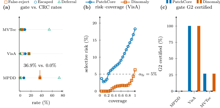
Figure 8: Dual gate versus single-threshold CRC baseline, pooled over both backbones and five seeds. a: Escaped-defect (open circles), false-reject (open squares), and deferral (open triangles) rates side by side across all three benchmarks; filled markers highlight CRC where it diverges. CRC has no deferral mechanism, so every non-passed image becomes an auto-reject; on MPDD this drives its false-reject rate to 36.9% against 0.0% for our gate at the same escaped-defect rate. b: Selective-prediction risk-at-coverage curves on VisA (PatchCore circles, Dinomally squares); the horizontal dashed line is \alpha_{fr} = 0.05 . The CRC baseline specializes to per-category selective classification with confidence-based abstention, but no coverage level reaches the 5% false-reject guarantee the gate certifies. c: Per-backbone G2 certification (PatchCore blue bars, Dinomally orange bars): the gate certifies both backbones on VisA (60/60 cells each), one on MVTec AD (20/75 each), and neither on MPDD (0/30 each); CRC certifies zero cells on every benchmark and backbone (0/75 MVTec AD, 0/60 VisA, 0/30 MPDD, per backbone) — it cannot deliver the false-reject guarantee at any coverage.
