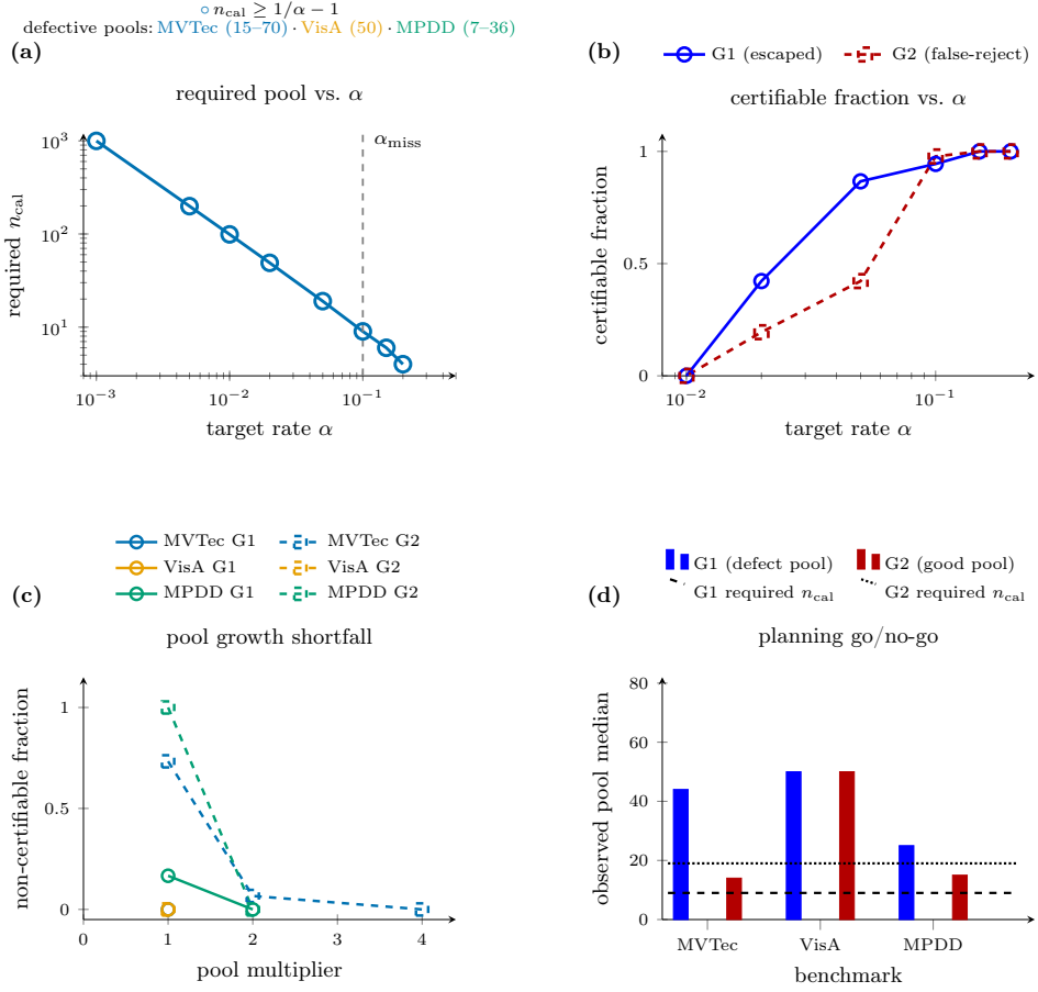
Figure 7: Calibration-pool planning curves from the frozen per-category pool sizes. (a) Required n_{\text{cal}} vs. target rate \alpha (finite-sample floor identity); the dashed line marks \alpha_{\text{miss}} = 0.10 , and the outside key lists observed per-category defective-pool extents (frozen min–max counts; not uncertainty intervals). (b) Certifiable category fraction vs. \alpha (G1 escaped-defect, solid; G2 false-reject, dashed), averaged over both backbones. (c) Pool-growth shortfall at the operating point as the non -certifiable fraction (zero = already fully certified). (d) Go/no-go check: bars are observed median pool sizes; horizontal dashed/dotted lines are the required n_{\text{cal}} on each axis (thresholds, not uncertainty intervals).
