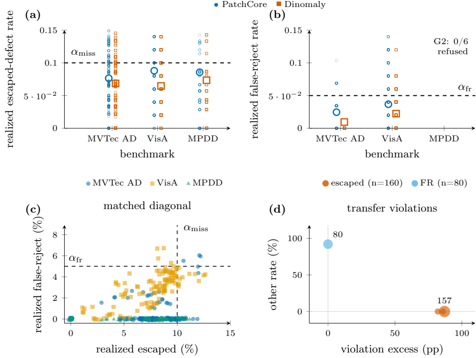
Figure 13: Per-repeat realized rates (frozen protocol; 6,400 escaped-defect and 3,200 false-reject certified-cell measurements). a : Escaped-defect rate vs. \alpha_{\text{miss}} = 0.10 ; b : false-reject rate vs. \alpha_{\text{fr}} = 0.05 (MPDD has no G2-certified cells under the primary protocol). Heavy dashes are per-(benchmark, backbone) means; every mean sits below target. c : Matched-diagonal validity cloud (330 cells, same-detector diagonal from the cross-detector transfer experiment): the certified region sits at or below both targets, confirming the guarantee holds on the same-detector reference. d : Transfer violation cloud: 160 escaped-defect violations (transfer adds 82–87 pp above \alpha_{\text{miss}} ) and 80 false-reject violations; the two violation types separate cleanly by direction.
