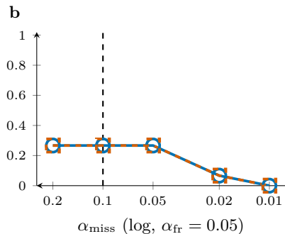
MVTec-AD: both-axis certified
