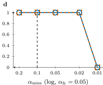
VisA: both-axis certified
