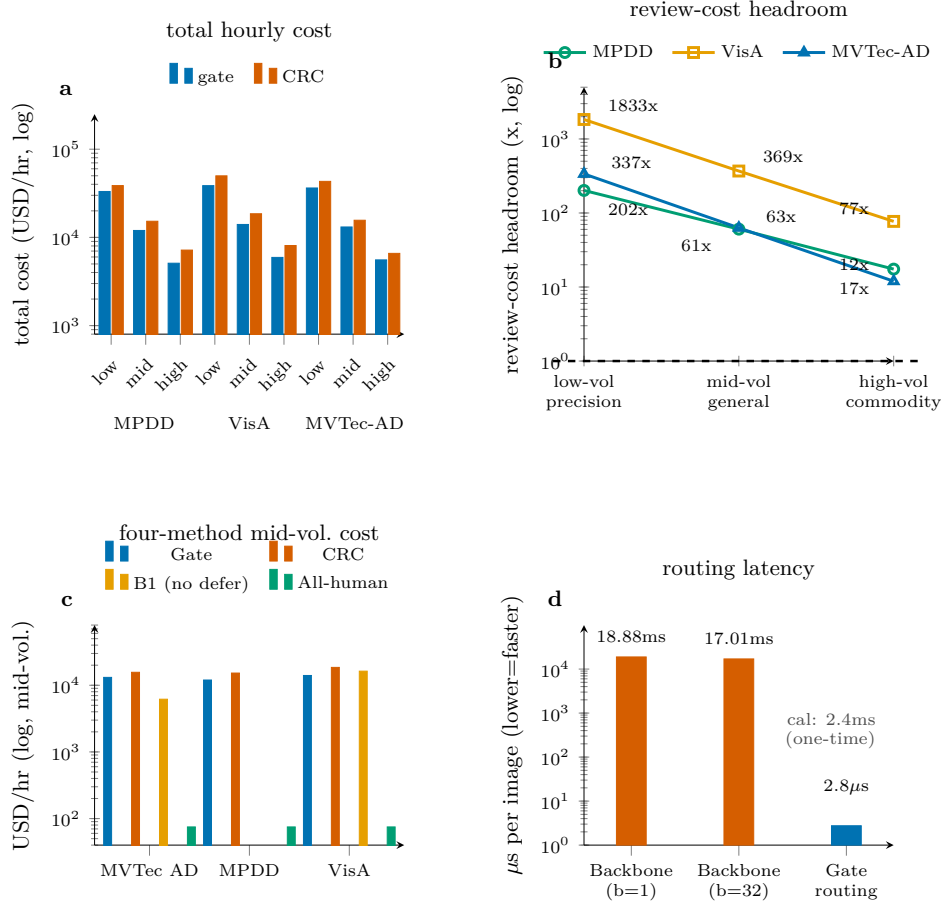
Figure 9: Deployment economics of the certified gate versus the CRC single-threshold baseline at frozen rates. Scenario groups: low-volume precision (100 parts/hour), mid-volume general (600), high-volume commodity (3,000); scenarios are assumed illustrative inputs. a: Total hourly cost (gate vs. CRC) across all nine benchmark-scenario cells: the gate is cheaper in every cell. b: Review-cost headroom — the multiple by which the assumed review cost can rise before the gate stops being cheaper: 12×–1833× (log; break-even at 1×). c: Four-method total hourly cost at mid-volume general, including the original B1 binding-demo arm (no deferral, post-hoc, unavailable for MPDD); the gate is cheapest on MVTEC AD and VisA. d: Routing latency: the gate adds 2.8 μs per image amortised (right bar), against 18.9 ms backbone inference at batch size 1 and 17.0 ms batched (left bars). Calibration is a one-time 2.4 ms per reset.
