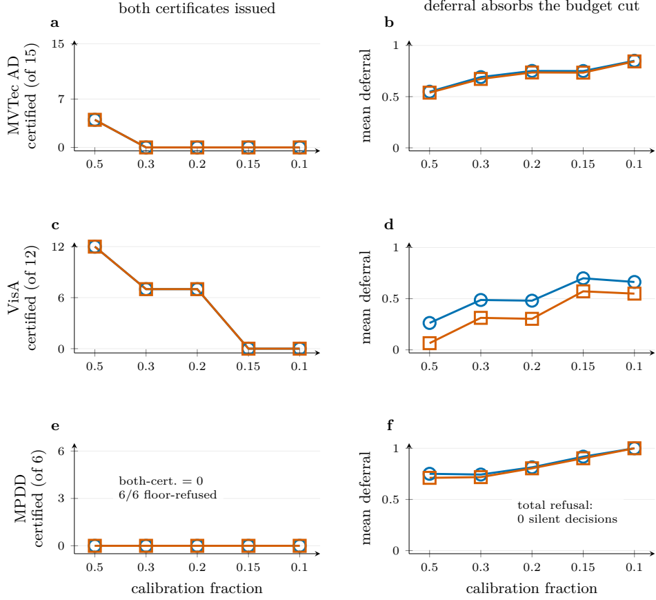
Figure 6: Calibration-budget sensitivity at the paper’s operating point ( \alpha_{\text{miss}} = 0.10 , \alpha_{\text{fr}} = 0.05 ; R = 20 , five seeds; post-freeze exploratory). Rows are MVTec AD (a,b), VisA (c,d), and MPDD (e,f). Left panels show categories certified on both axes as the calibration fraction shrinks; right panels show mean deferral. Shaded bands span seed minima to maxima. Lost budget is absorbed by deferral, never by silent error: at fraction 0.10 MPDD refuses everything (deferral exactly 1.0, zero silent decisions). The flat zero in panel (e) for MPDD at fraction 0.10 is a measured refusal across all 20 repeats and five seeds — the floors refuse all six categories, so both-certified is identically zero and deferral saturates at 1.0 rather than crossing into silent mis-coverage.
