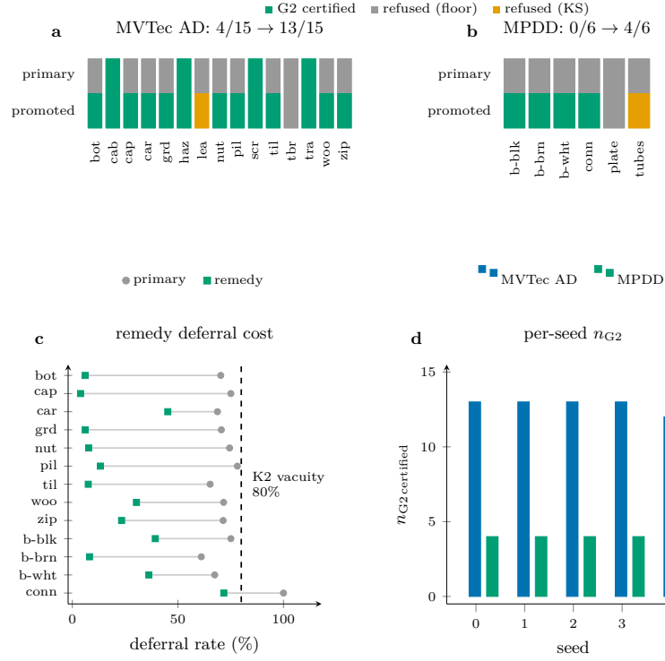
Figure 10: The G2 train-holdout remedy (PatchCore; seeds 0–3 identical, seed 4 differs on screw). a : MVTec AD: 4/15 → 13/15, leather KS-refused every seed. b : MPDD: 0/6 → 4/6. Category codes — MVTec AD: bot/cab/cap/car/grd/haz/lea/nut/pil/scr/til/tbr/tra/woo/zip; MPDD: b-blk/b-brn/b-wht/conn/plate/tubes. Tiles: certified (green), refused at floor (grey), refused by KS (amber). c : Remedy deferral cost per rescued category: promotion opens the auto-reject region and reduces deferral for most categories; connector (MPDD) remains near-vacuous at 71.7%. d : Per-seed n_{G2 \text{ certified}} under the promoted arm: 13/15 stable in seeds 0–3 (screw degrades to 12/15 in seed 4 when KS fails); MPDD holdout certifies 4/6 in all five seeds.
