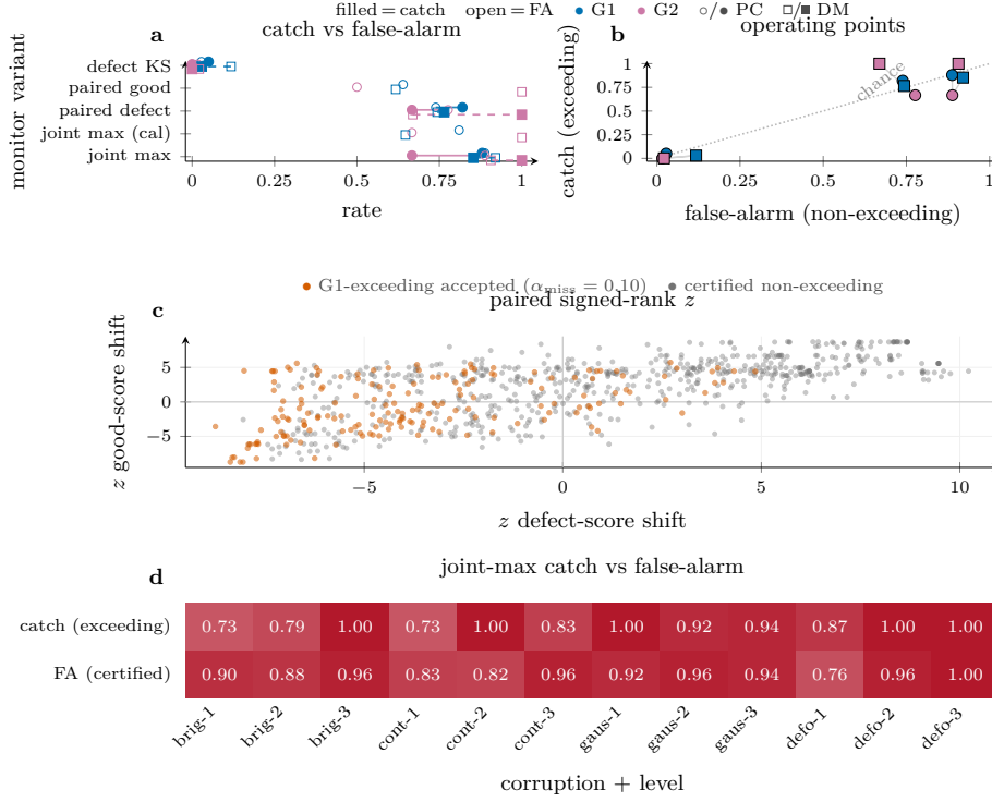
Figure 15: The drift-monitor design space, tested (post-freeze exploratory, seed 0; frozen joint record). a : catch rate (filled) vs. false-alarm rate (open) per monitor variant and detector \times guarantee arm — the frozen defect-marginal KS catches 5.0%/2.9%; the pairing-respecting variants catch more but at matching false-alarm. b : the same arms as operating points against the chance diagonal: no variant separates. c : per-cell paired signed-rank z of good- and defect-score shifts; G1-exceeding accepted cells (vermillion) sit inside the same cloud as certified cells — there is no location-only signature to detect. d : catch vs. false-alarm rate of the joint max-statistic by corruption and severity level: the two rows track each other at every cell, the indiscriminate regime in one view. From the frozen joint-monitor record (792 cells; reproduction gates passed: defect-marginal catches 5/100 and 1/34 reproduced exactly).
