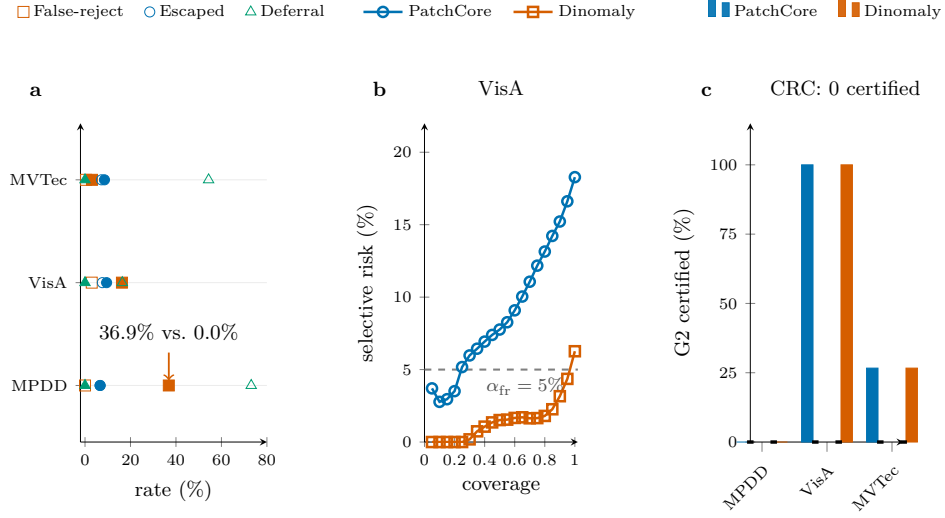
Figure 8: Dual gate versus single-threshold CRC baseline, pooled over both backbones and five seeds (Table 3). a: Escaped-defect, false-reject, and deferral rates side by side across all three benchmarks. CRC has no deferral mechanism, so every non-passed image becomes an auto-reject; on MPDD this drives its false-reject rate to 36.9% against 0.0% for our gate at the same escaped-defect rate. b: Selective-prediction risk-at-coverage curves per backbone on VisA — the CRC baseline specializes to per-category selective classification with confidence-based abstention, but no coverage level reaches the 5% false-reject guarantee the gate certifies. c: Per-backbone G2 certification: the gate certifies both backbones on VisA (60/60 cells each), one on MVTec AD (20/75 each), and neither on MPDD (0/30 each); CRC certifies zero cells on every benchmark and backbone (0/75 MVTec AD, 0/60 VisA, 0/30 MPDD, per backbone) — it cannot deliver the false-reject guarantee at any coverage.
