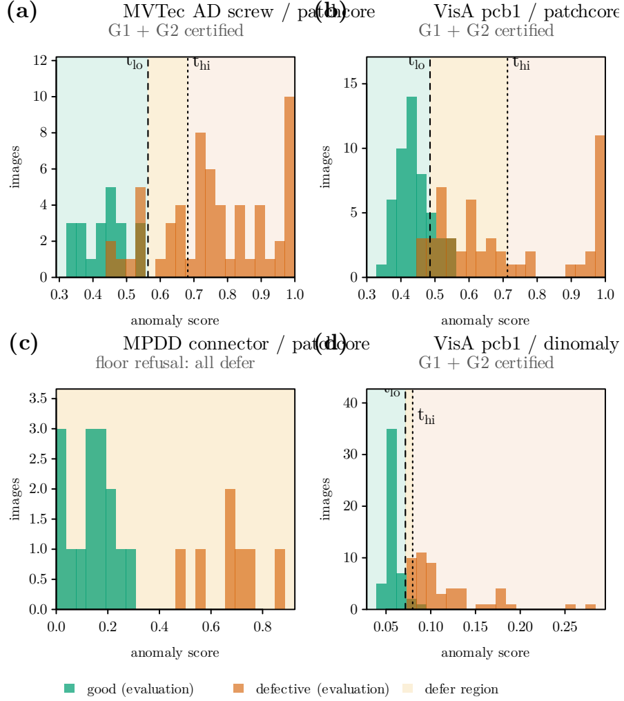
Figure 2: The gate’s mechanism on real scores (seed 0, repeat 0; evaluation-half histograms, thresholds calibrated on the calibration half). a: MVTec AD screw (PatchCore): both certificates, defer band absorbs the overlap region. b: VisA pcb1 (PatchCore): both certified with a wider band. c: MPDD connector (PatchCore): separation looks clean to the eye yet the gate refuses — pools too small for the 1/(n_{cal} + 1) floors, both thresholds at \pm\infty . d: VisA pcb1 under Dinomaly (contrast with b): same category, different scorer; both G1 and G2 certify with a narrow band ( t_{lo} = 0.072 , t_{hi} = 0.080 ), showing that a different detector with cleaner score separation can close the defer band substantially.
