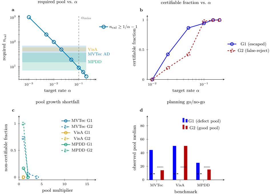
Figure 7: Calibration-pool planning curves, derived from the frozen per-category pool sizes. (a) Required calibration-pool size against target rate \alpha (Equation 9); shaded bands span the observed per-category defective-pool ranges of the three benchmarks, so a band lying above the curve at a given \alpha means that benchmark can pay for that rate. The dashed line marks the paper’s \alpha_{\text{miss}} = 0.10 operating point. (b) Certifiable fraction of categories against target rate, averaged over both backbones, for the escaped-defect (G1, solid) and false-reject (G2, dashed) axes. (c) Effect of pool growth at the paper’s operating point, plotted as the non -certifiable fraction so that the three series which already certify every category coincide on the zero baseline rather than on 1; doubling the pool clears all but a residual few percent, and 4\times clears everything. (d) The planning rule as a go/no-go check: bars are the observed median pool sizes, dashed segments the n_{\text{cal}} each axis requires. MVTec AD and MPDD sit below the line on the good-image pool that G2 draws on (medians 14 and 15 against a required 19), which is exactly why their false-reject certificates are the ones that abstain. All panels are analytic consequences of the floor \alpha_{\text{min}} = 1/(n_{\text{cal}} + 1) evaluated on the frozen pools, verified to reproduce every frozen certified count at the paper’s operating point.
