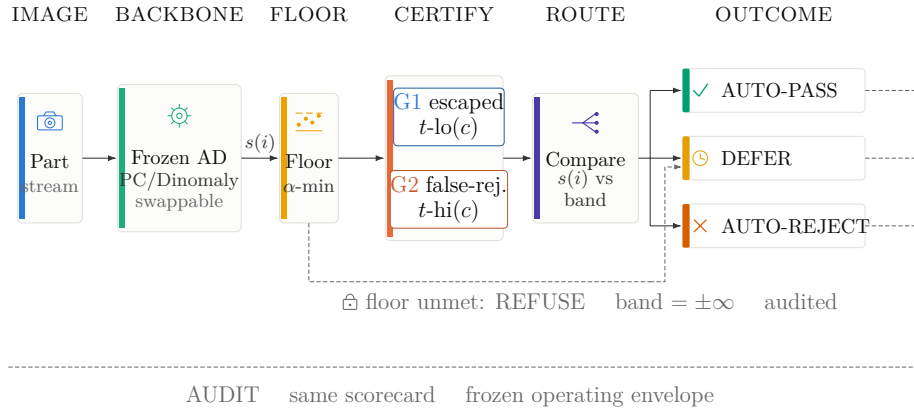
Figure 1: Horizontal method overview. A frozen, interchangeable PatchCore or Dinomaly backbone scores each image. Per-category calibration first checks the certifiability floor \alpha_{\min} = 1/(n_{\text{cal}} + 1) (Section 3.2); when met, the parallel G1 and G2 cards set t_{\text{lo}}(c) and t_{\text{hi}}(c) so that P(s \leq t_{\text{lo}} \mid \text{defective}) \leq \alpha_{\text{miss}} and P(s \geq t_{\text{hi}} \mid \text{good}) \leq \alpha_{\text{fr}} , respectively (Section 3.1). Comparing s_i with this band routes the part to auto-pass, defer, or auto-reject. The dashed floor-control branch is distinct from that data path: an unmet floor refuses the axis (band = \pm\infty ), records audited-not-certified, and forces defer rather than auto-reject. All three outcomes feed the same audit scorecard and frozen operating envelope; the schematic makes no claim that either backbone is superior.
