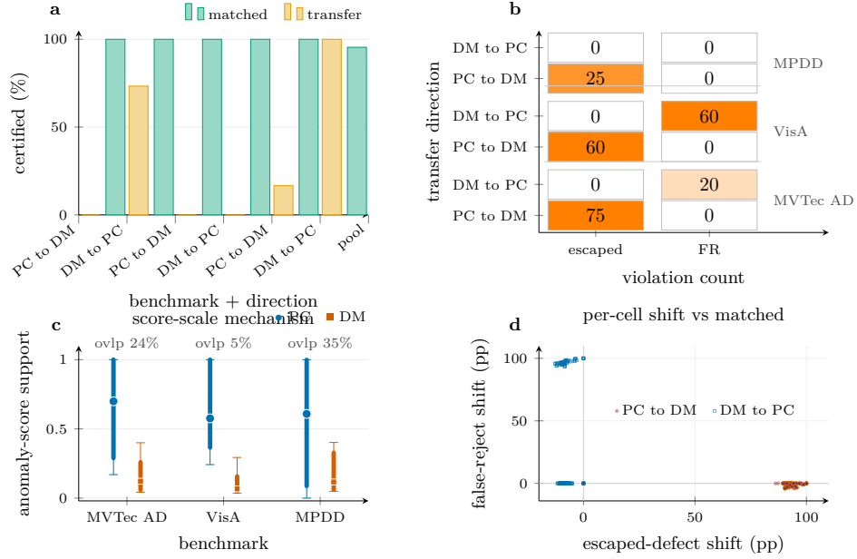
Figure 16: Calibrated gates do not transfer across detectors (post-freeze exploratory, seed-level; frozen transfer record). a : certification rate, transfer vs. partition-matched same-detector diagonal, per benchmark and direction — the diagonal certifies nearly everywhere; the transfer arm collapses. b : guarantee-violation counts per benchmark and direction: 160/165 escaped-defect violations (PatchCore→Dinomaly, abbreviated “PC to DM” in the figure), 80/165 false-reject violations (reverse, “DM to PC”). c : the mechanism — per-detector score-scale ranges barely overlap (support overlap 0.241/0.053/0.353 on MVTec AD/VisA/MPDD), so a threshold calibrated on one detector sits far outside the other’s score support. d : per-cell realized-rate shift vs. the matched diagonal; the two clusters show total inversion in opposite directions. From the frozen transfer record (330 cells; same-detector diagonal reproduces the frozen certification records exactly, 30/30).
