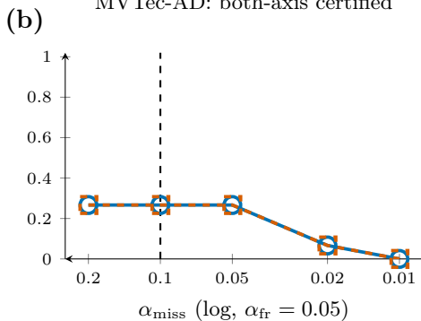
MVTec-AD: both-axis certified
