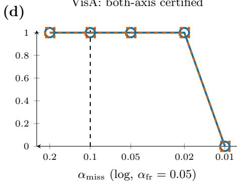
VisA: both-axis certified
