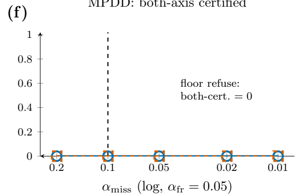
MPDD: both-axis certified
