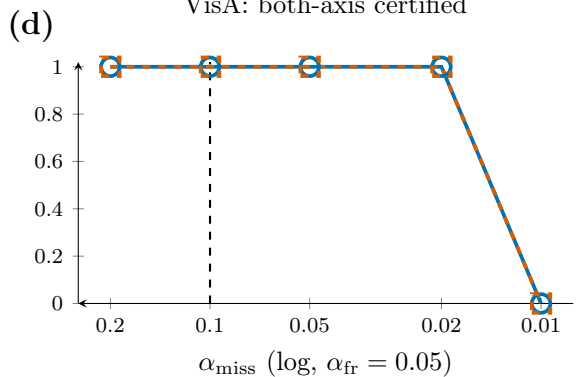
VisA: both-axis certified
