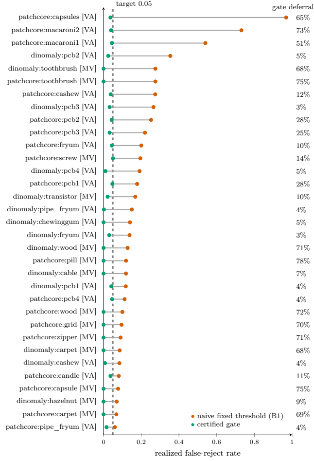
Figure 12: Binding cells on the false-reject axis (post-hoc). Same encoding as Figure 11; the dashed line is the \alpha_{fr} = 0.05 target. The VisA PatchCore capsules cell (top) is the extreme case: a global threshold auto-rejects 96.8% of good parts where the certified gate holds 3.7%.
