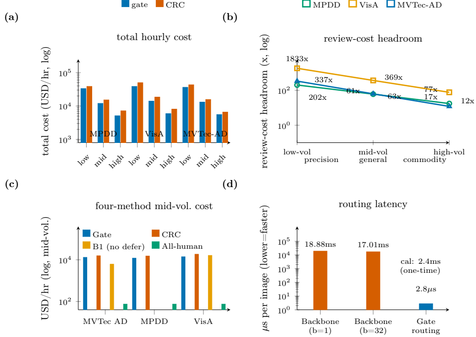
Figure 9: Deployment economics of the certified gate versus the CRC single-threshold baseline at frozen rates. Scenario groups: low-volume precision (100 parts/hour), mid-volume general (600), high-volume commodity (3,000); scenarios are assumed illustrative inputs. a: Total hourly cost (gate vs. CRC) across all nine benchmark-scenario cells: the gate is cheaper in every cell. b: Review-cost headroom — the multiple by which the assumed review cost can rise before the gate stops being cheaper: 12\times – 1833\times (log; break-even at 1\times ). c: Four-method total hourly cost at mid-volume general, including the original B1 binding-demo arm (no deferral, post-hoc, unavailable for MPDD); the gate is cheapest on MVTec AD and VisA. d: Routing latency: the gate adds 2.8\mu s per image amortised (right bar), against 18.9ms backbone inference at batch size 1 and 17.0ms batched (left bars). Calibration is a one-time 2.4ms per reset.
