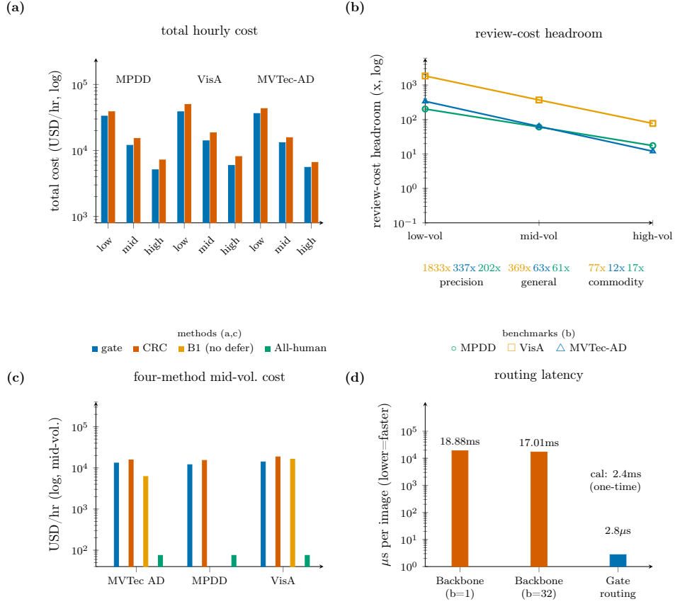
Figure 9: Deployment economics of the certified gate versus the CRC single-threshold baseline at frozen rates. Scenario groups: low-volume precision (100 parts/hour), mid-volume general (600), high-volume commodity (3,000); scenarios are assumed illustrative inputs. a : Total hourly cost across all nine benchmark-scenario cells (blue = gate, orange = CRC): the gate is cheaper in every cell. b : Review-cost headroom — the multiple by which the assumed review cost can rise before the gate stops being cheaper: 12 \times - 1833 \times (log; break-even at 1 \times ); lines are benchmarks (circle MPDD, square VisA, triangle MVTec AD). c : Four-method total hourly cost at mid-volume general (blue gate, orange CRC, gold B1 no-deferral, teal all-human), including the original B1 binding-demo arm (no deferral, post-hoc, unavailable for MPDD); the gate is cheapest on MVTec AD and VisA among automated methods. d : Routing latency: the gate adds 2.8 \mu s per image amortised (blue right bar), against 18.9ms backbone inference at batch size 1 and 17.0ms batched (orange left bars). Calibration is a one-time 2.4ms per reset.
