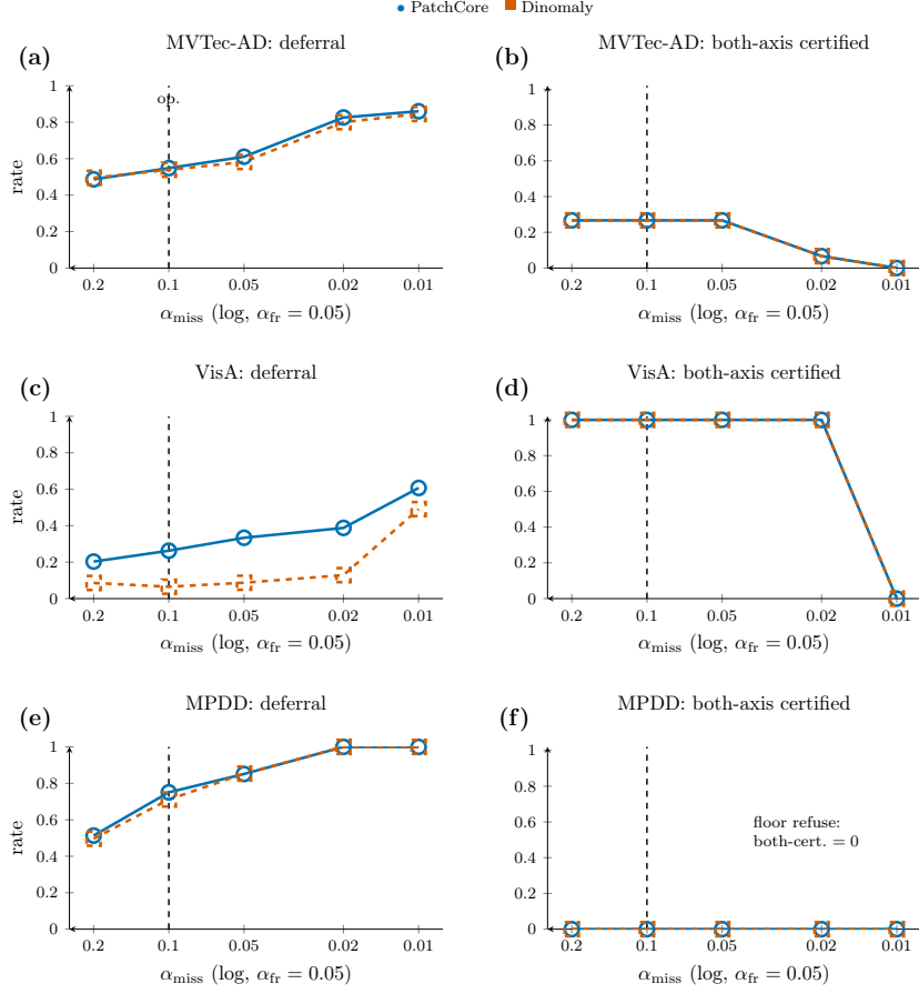
Figure 5: The operating-point frontier on the frozen code path (post-freeze exploratory sweep; the construction reproduces every frozen artifact exactly at the paper’s operating point). Rows are MVTec AD (a,b), VisA (c,d), and MPDD (e,f). Left panels show mean deferral versus the escaped-defect target \alpha_{\text{miss}} at \alpha_{\text{fr}} = 0.05 ; right panels show the fraction of categories certified on both axes. Solid circles denote PatchCore and dashed squares Dinomaly; shaded bands span seed minima to maxima. The vertical dashed line marks the paper’s operating point. The flat zero in panel (f) for MPDD at \alpha_{\text{miss}} \in \{0.02, 0.01\} is a measured refusal: the floor ( \alpha_{\text{min}} = 1/(n_{\text{cal}}^{\text{frac}} + 1) ) refuses all six MPDD categories, so both-certified is identically zero on every repeat and deferral saturates at 1.0 (no silent decisions).
