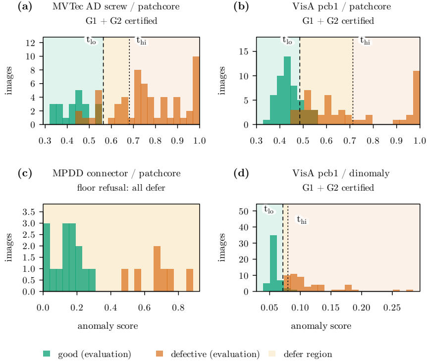
Figure 2: The gate’s mechanism on real scores (seed 0, repeat 0; evaluation-half histograms, thresholds calibrated on the calibration half). Green bars are good evaluation scores, orange bars defective evaluation scores; the beige band is the defer region between dashed t_{\text{lo}} and dotted t_{\text{hi}} . a: MVTec AD screw (PatchCore): both certificates, defer band absorbs the overlap region. b: VisA pcb1 (PatchCore): both certified with a wider band. c: MPDD connector (PatchCore): separation looks clean to the eye yet the gate refuses — pools too small for the 1/(n_{\text{cal}} + 1) floors, both thresholds at \pm\infty (entire support deferred). d: VisA pcb1 under Dinomaly (contrast with b): same category, different scorer; both G1 and G2 certify with a narrow band ( t_{\text{lo}} = 0.072 , t_{\text{hi}} = 0.080 ), showing that a different detector with cleaner score separation can close the defer band substantially.
