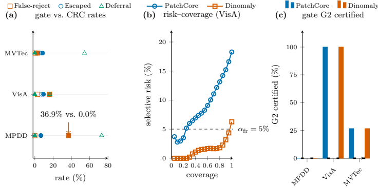
Figure 8: Dual gate versus single-threshold CRC baseline, pooled over both backbones and five seeds (Table 3). a: Escaped-defect (open circles), false-reject (open squares), and deferral (open triangles) rates side by side across all three benchmarks; filled markers highlight CRC where it diverges. CRC has no deferral mechanism, so every non-passed image becomes an auto-reject; on MPDD this drives its false-reject rate to 36.9% against 0.0% for our gate at the same escaped-defect rate. b: Selective-prediction risk-at-coverage curves on VisA (PatchCore circles, Dinomaly squares); the horizontal dashed line is \alpha_{\text{fr}} = 0.05 . The CRC baseline specializes to per-category selective classification with confidence-based abstention, but no coverage level reaches the 5% false-reject guarantee the gate certifies. c: Per-backbone G2 certification (PatchCore blue bars, Dinomaly orange bars): the gate certifies both backbones on VisA (60/60 cells each), one on MVTec AD (20/75 each), and neither on MPDD (0/30 each); CRC certifies zero cells on every benchmark and backbone (0/75 MVTec AD, 0/60 VisA, 0/30 MPDD, per backbone) — it cannot deliver the false-reject guarantee at any coverage.
