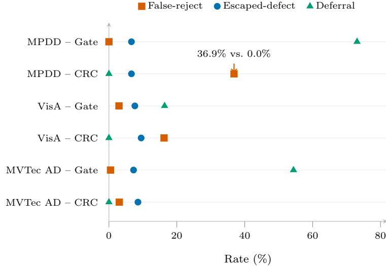
Figure 3: Escaped-defect, false-reject, and deferral rates for our dual gate versus the single-threshold CRC baseline (Table 4), pooled over both backbones and five seeds. CRC has no deferral mechanism, so every non-passed image becomes an auto-reject; on MPDD this drives its false-reject rate to 36.9% against 0.0% for our gate at the same escaped-defect rate.
