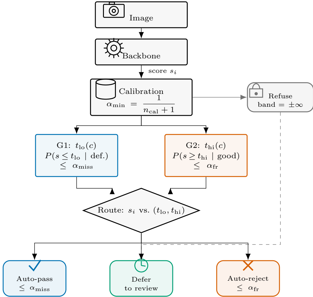
Figure 1: Method overview. A frozen backbone (PatchCore or Dinomaly, interchangeable) scores each image; per-category calibration checks the certifiability floor \alpha_{\min} = 1/(n_{\text{cal}} + 1) (Section 3.2) and, when met, sets the G1 escaped-defect threshold t_{\text{lo}}(c) and the G2 false-reject threshold t_{\text{hi}}(c) (Section 3.1). The three-way route then compares each score against (t_{\text{lo}}, t_{\text{hi}}) to auto-pass, defer, or auto-reject, carrying the stated escaped-defect and false-reject guarantees; an unmet floor instead refuses the axis (band = \pm\infty ), defers, and is reported audited-not-certified.
