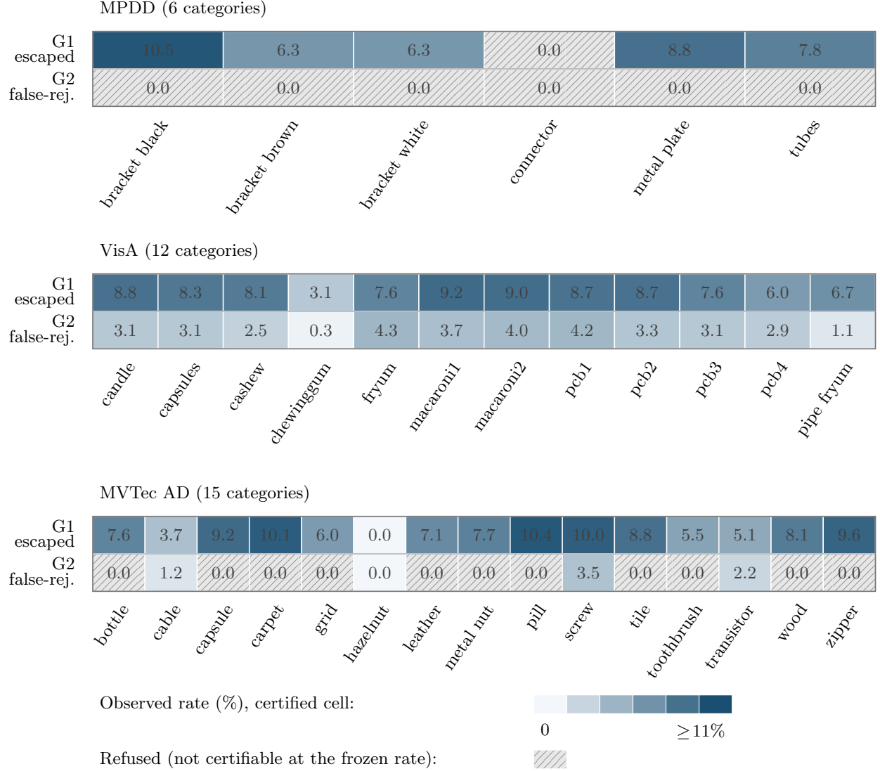
Figure 2: Per-category certification map for escaped-defect (G1) and false-reject (G2) at the frozen rates ( \alpha_{\text{miss}} = 0.10 , \alpha_{\text{fr}} = 0.05 ), pooled over both backbones and five seeds, for MPDD, VisA, and MVTec AD. Colored cells are certified, shaded by the observed rate; hatched gray cells are refused as not certifiable at the frozen rate under the primary protocol (all of MPDD’s G2 column, MPDD’s connector on G1, and the 11/15 MVTec AD categories below the false-reject floor in Table 3).
