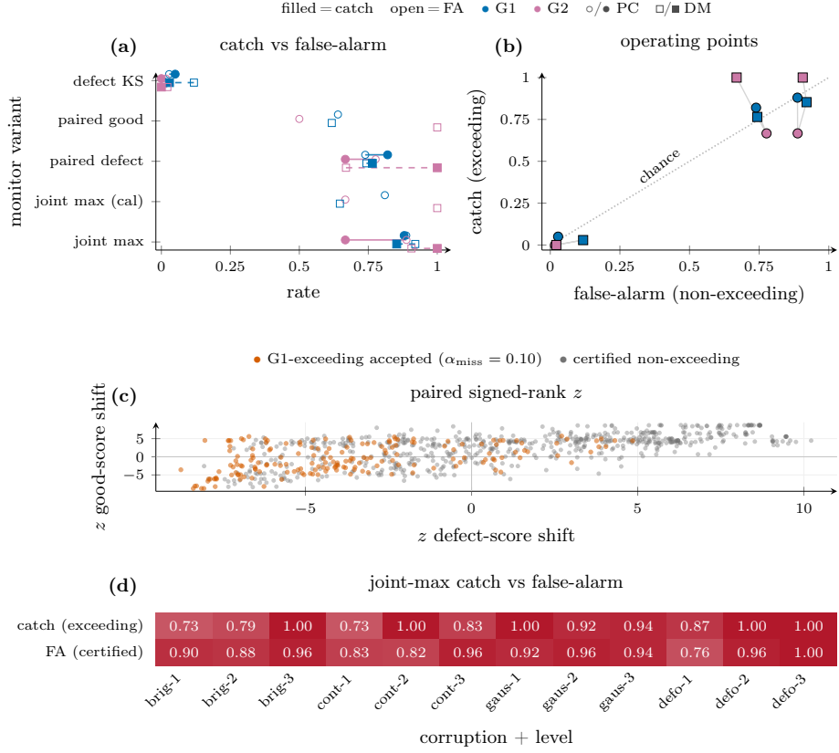
Figure 15: The drift-monitor design space, tested (post-freeze exploratory, seed 0; frozen joint record). a: catch rate (filled) vs. false-alarm rate (open) per monitor variant and detector \times guarantee arm — the frozen defect-marginal KS catches 5.0%/2.9%; the pairing-respecting variants catch more but at matching false-alarm. b: the same arms as operating points against the chance diagonal: no variant separates. c: per-cell paired signed-rank z of good- and defect-score shifts; G1-exceeding accepted cells (vermillion) sit inside the same cloud as certified cells — there is no location-only signature to detect. d: catch vs. false-alarm rate of the joint max-statistic by corruption and severity level: the two rows track each other at every cell, the indiscriminate regime in one view. From the frozen joint-monitor record (792 cells; reproduction gates passed: defect-marginal catches 5/100 and 1/34 reproduced exactly).
