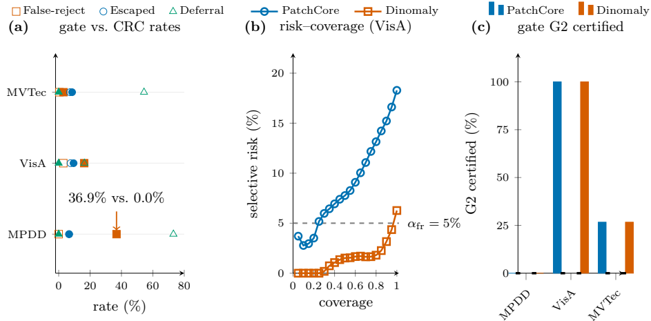
Figure 8: Dual gate versus single-threshold CRC baseline, pooled over both backbones and five seeds (Table 3). a: Escaped-defect, false-reject, and deferral rates side by side across all three benchmarks. CRC has no deferral mechanism, so every non-passed image becomes an auto-reject; on MPDD this drives its false-reject rate to 36.9% against 0.0% for our gate at the same escaped-defect rate. b: Selective-prediction risk-at-coverage curves per backbone on VisA — the CRC baseline specializes to per-category selective classification with confidence-based abstention, but no coverage level reaches the 5% false-reject guarantee the gate certifies. c: Per-backbone G2 certification: the gate certifies both backbones on VisA (60/60 cells each), one on MVTec AD (20/75 each), and neither on MPDD (0/30 each); CRC certifies zero cells on every benchmark and backbone (0/75 MVTec AD, 0/60 VisA, 0/30 MPDD, per backbone) — it cannot deliver the false-reject guarantee at any coverage.
