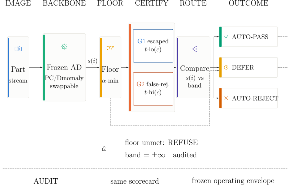
Figure 1: Horizontal method overview. A frozen, interchangeable PatchCore or Dinomaly backbone scores each image. Per-category calibration first checks the certifiability floor \alpha_{\min} = 1/(n_{\text{cal}} + 1) (Section 3.2); when met, the parallel G1 and G2 cards set t_{\text{lo}}(c) and t_{\text{hi}}(c) so that, under classical split conformal, \Pr\{s > t_{\text{hi}}\} \leq \alpha_{\text{fr}} on good scores and \Pr\{s < t_{\text{lo}}\} \leq \alpha_{\text{miss}} on defective scores (marginal over the calibration–test exchangeable pool; Section 3.1). Comparing s_i with this band routes the part to auto-pass, defer, or auto-reject. The dashed floor-control branch is distinct from that data path: an unmet floor refuses the axis (band = \pm\infty ), records audited-not-certified, and forces defer rather than auto-reject. All three outcomes feed the same audit scorecard and frozen operating envelope; the schematic makes no claim that either backbone is superior.
