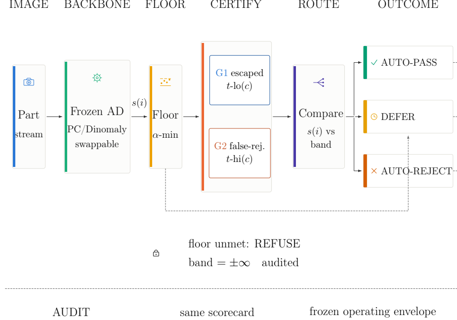
Figure 1: Horizontal method overview. A frozen, interchangeable PatchCore or Dinomaly backbone scores each image. Per-category calibration first checks the certifiability floor \alpha_{\min} = 1/(n_{\text{cal}} + 1) (Section 3.2); when met, the parallel G1 and G2 cards set t_{\text{lo}}(c) and t_{\text{hi}}(c) so that, under classical split conformal, \Pr\{s > t_{\text{hi}}\} \leq \alpha_{\text{fr}} on good scores and \Pr\{s < t_{\text{lo}}\} \leq \alpha_{\text{miss}} on defective scores (marginal over the calibration–test exchangeable pool; Section 3.1). Comparing s_i with this band routes the part to auto-pass, defer, or auto-reject. The dashed floor-control branch is distinct from that data path: an unmet floor refuses the axis (band = \pm\infty ), records audited-not-certified, and forces defer rather than auto-reject. All three outcomes feed the same audit scorecard and frozen operating envelope; the schematic makes no claim that either backbone is superior.
