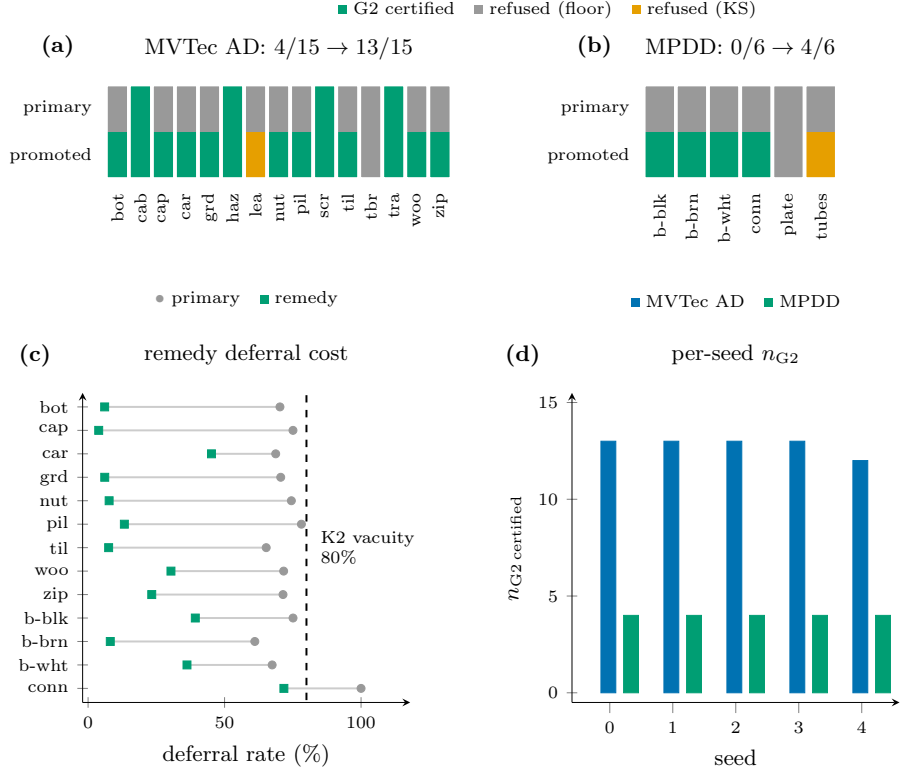
Figure 10: The G2 train-holdout remedy (PatchCore; seeds 0–3 identical, seed 4 differs on screw). a : MVTec AD: 4/15 → 13/15, leather KS-refused every seed. b : MPDD: 0/6 → 4/6. Category codes — MVTec AD: bot/cab/cap/car/grd/haz/lea/nut/pil/scr/til/tbr/tra/woo/zip; MPDD: b-blk/b-brn/b-wht/conn/plate/tubes. Tiles: certified (green), refused at floor (grey), refused by KS (amber). c : Remedy deferral cost per rescued category: promotion opens the auto-reject region and reduces deferral for most categories; connector (MPDD) remains near-vacuous at 71.7%. d : Per-seed n_{G2 \text{ certified}} under the promoted arm: 13/15 stable in seeds 0–3 (screw degrades to 12/15 in seed 4 when KS fails); MPDD holdout certifies 4/6 in all five seeds.
