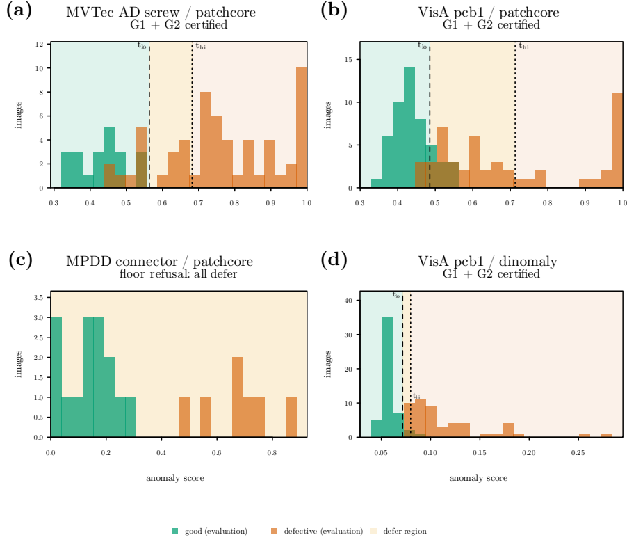
Figure 2: The gate’s mechanism on real scores (seed 0, repeat 0; evaluation-half histograms, thresholds calibrated on the calibration half). a: MVtec AD screw (PatchCore): both certificates, defer band absorbs the overlap region. b: VisA pcb1 (PatchCore): both certificates with a wider band. c: MPDD connector (PatchCore): separation looks clean to the eye yet the gate refuses — pools too small for the 1/(n_{cal} + 1) floors, both thresholds at \pm\infty . d: VisA pcb1 under Dinomaly (contrast with b): same category, different scorer; both G1 and G2 certify with a narrow band ( t_{lo} = 0.072 , t_{hi} = 0.080 ), showing that a different detector with cleaner score separation can close the defer band substantially.
