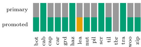
(a) MVTec AD: 4/15 \rightarrow 13/15
