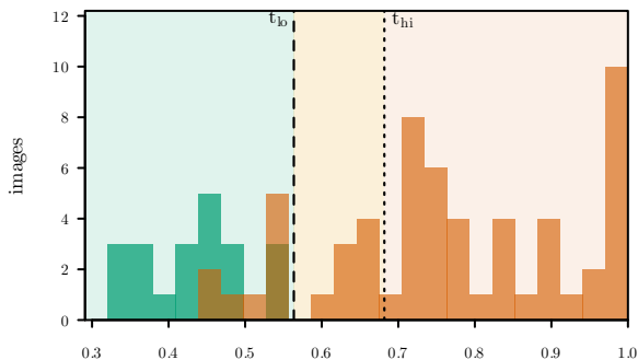
(a) MVTec AD screw / patchcore G1 + G2 certified
