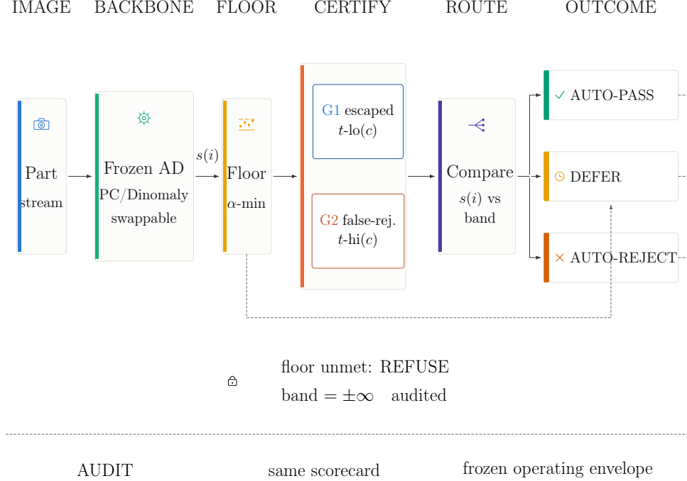
Figure 1: Method overview. A frozen backbone (PatchCore or Dinomaly, interchangeable) scores each image; per-category calibration checks the certifiability floor \alpha_{\min} = 1/(n_{\text{cal}} + 1) (Section 3.2) and, when met, sets the G1 escaped-defect threshold t_{\text{lo}}(c) and the G2 false-reject threshold t_{\text{hi}}(c) (Section 3.1). The three-way route then compares each score against (t_{\text{lo}}, t_{\text{hi}}) to auto-pass, defer, or auto-reject, carrying the stated escaped-defect and false-reject guarantees; an unmet floor instead refuses the axis (band = \pm\infty ), defers, and is reported audited-not-certified.
