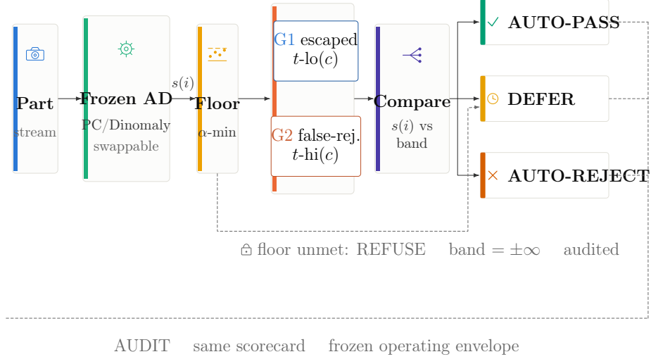
Figure 1: Method overview. A frozen backbone (PatchCore or Dinomally, interchangeable) scores each image; per-category calibration checks the certifiability floor \alpha_{\min} = 1/(n_{\text{cal}} + 1) (Section 3.2) and, when met, sets the G1 escaped-defect threshold t_{\text{lo}}(c) and the G2 false-reject threshold t_{\text{hi}}(c) (Section 3.1). The three-way route then compares each score against (t_{\text{lo}}, t_{\text{hi}}) to auto-pass, defer, or auto-reject, carrying the stated escaped-defect and false-reject guarantees; an unmet floor instead refuses the axis (band = \pm\infty ), defers, and is reported audited-not-certified.
