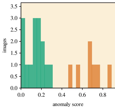
(c) MPDD connector / patchcore floor refusal: all defer
