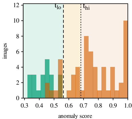
(c) MPDD connector / patchcore floor refusal: all defer
