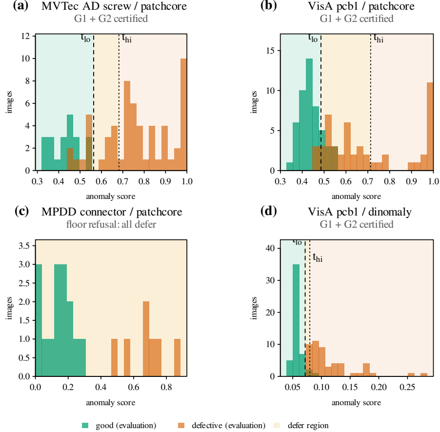
Figure 2: The gate’s mechanism on real scores (seed 0, repeat 0; evaluation-half histograms, thresholds calibrated on the calibration half). a: MVTec AD screw (PatchCore): both certificates, defer band absorbs the overlap region. b: VisA pcb1 (PatchCore): both certified with a wider band. c: MPDD connector (PatchCore): separation looks clean to the eye yet the gate refuses — pools too small for the 1/(n_{\text{cal}} + 1) floors, both thresholds at \pm\infty . d: VisA pcb1 under Dinomaly (contrast with b): same category, different scorer; both G1 and G2 certify with a narrow band ( t_{\text{lo}} = 0.072 , t_{\text{hi}} = 0.080 ), showing that a different detector with cleaner score separation can close the defer band substantially.
