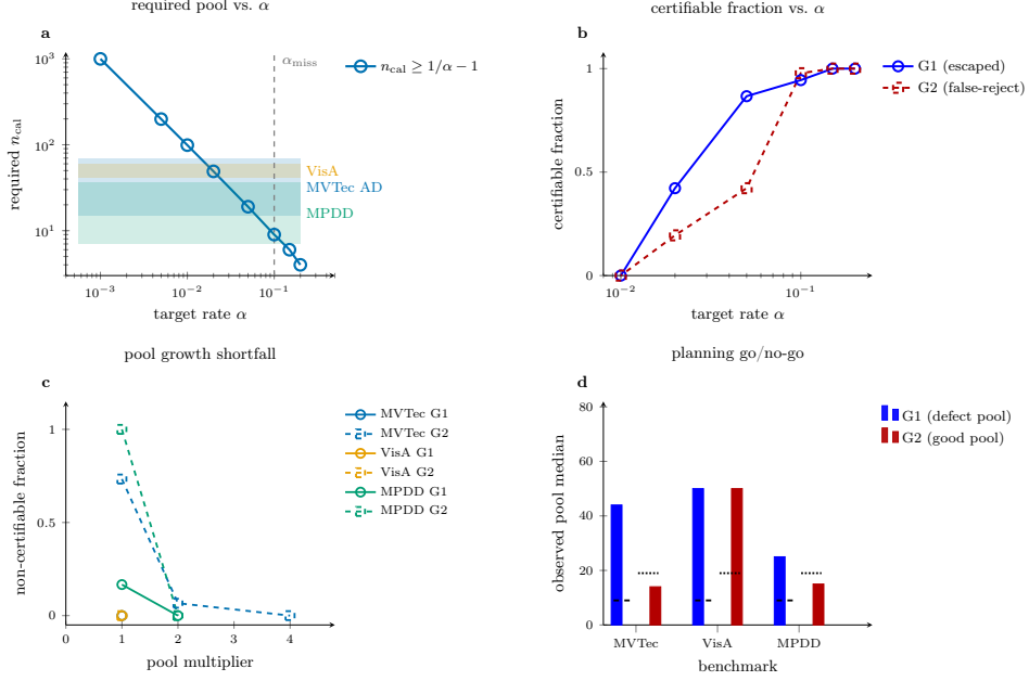
Figure 7: Calibration-pool planning curves, derived from the frozen per-category pool sizes. (a) Required calibration-pool size against target rate \alpha (Equation 9); shaded bands span the observed per-category defective-pool ranges of the three benchmarks, so a band lying above the curve at a given \alpha means that benchmark can pay for that rate. The dashed line marks the paper’s \alpha_{\text{miss}} = 0.10 operating point. (b) Certifiable fraction of categories against target rate, averaged over both backbones, for the escaped-defect (G1, solid) and false-reject (G2, dashed) axes. (c) Effect of pool growth at the paper’s operating point, plotted as the non -certifiable fraction so that the three series which already certify every category coincide on the zero baseline rather than on 1; doubling the pool clears all but a residual few percent, and 4\times clears everything. (d) The planning rule as a go/no-go check: bars are the observed median pool sizes, dashed segments the n_{\text{cal}} each axis requires. MVTec AD and MPDD sit below the line on the good-image pool that G2 draws on (medians 14 and 15 against a required 19), which is exactly why their false-reject certificates are the ones that abstain. All panels are analytic consequences of the floor \alpha_{\text{min}} = 1/(n_{\text{cal}} + 1) evaluated on the frozen pools, verified to reproduce every frozen certified count at the paper’s operating point.
