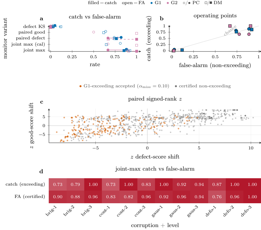
Figure 15: The drift-monitor design space, tested (post-freeze exploratory, seed 0; frozen joint record). a : catch rate (filled) vs. false-alarm rate (open) per monitor variant and detector×guarantee arm — the frozen defect-marginal KS catches 5.0%/2.9%; the pairing-respecting variants catch more but at matching false-alarm. b : the same arms as operating points against the chance diagonal: no variant separates. c : per-cell paired signed-rank z of good- and defect-score shifts; G1-exceeding accepted cells (vermillion) sit inside the same cloud as certified cells — there is no location-only signature to detect. d : catch vs. false-alarm rate of the joint max-statistic by corruption and severity level: the two rows track each other at every cell, the indiscriminate regime in one view. From the frozen joint-monitor record (792 cells; reproduction gates passed: defect-marginal catches 5/100 and 1/34 reproduced exactly).
