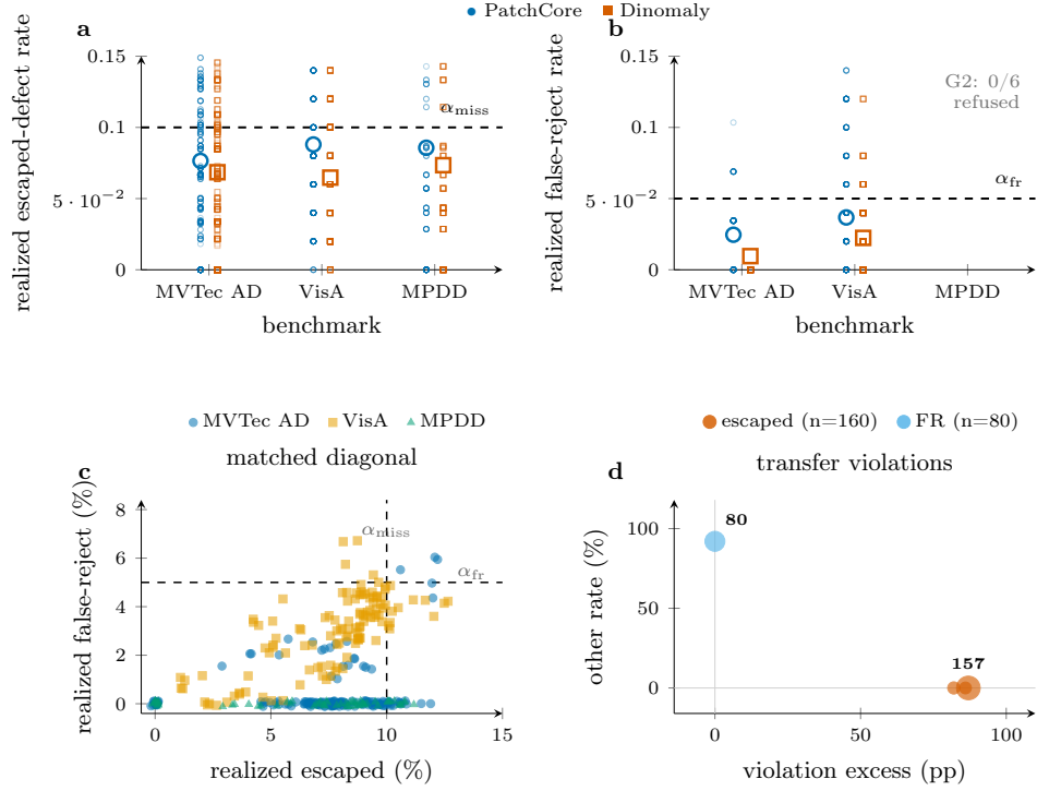
Figure 13: Per-repeat realized rates (frozen protocol; 6,400 escaped-defect and 3,200 false-reject certified-cell measurements). a: Escaped-defect rate vs. \alpha_{\text{miss}} = 0.10 ; b: false-reject rate vs. \alpha_{\text{fr}} = 0.05 (MPDD has no G2-certified cells under the primary protocol). Heavy dashes are per-(benchmark, backbone) means; every mean sits below target. c: Matched-diagonal validity cloud (330 cells, same-detector diagonal from the cross-detector transfer experiment): the certified region sits at or below both targets, confirming the guarantee holds on the same-detector reference. d: Transfer violation cloud: 160 escaped-defect violations (transfer adds 82–87 pp above \alpha_{\text{miss}} ) and 80 false-reject violations; the two violation types separate cleanly by direction.
