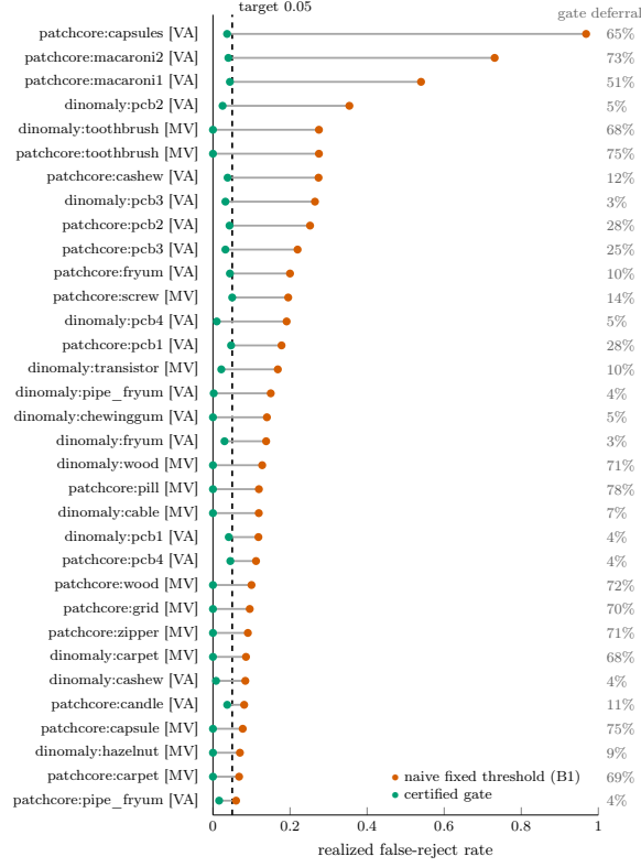
Figure 12: Binding cells on the false-reject axis (post-hoc). Same encoding as Figure 11; the dashed line is the \alpha_{fr} = 0.05 target. The VisA PatchCore capsules cell (top) is the extreme case: a global threshold auto-rejects 96.8% of good parts where the certified gate holds 3.7%.
