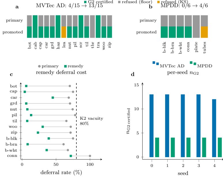
Figure 10: The G2 train-holdout remedy (PatchCore; seeds 0–3 identical, seed 4 differs on screw). a: MVTec AD: 4/15 \rightarrow 13/15, leather KS-refused every seed. b: MPDD: 0/6 \rightarrow 4/6. Category codes — MVTec AD: bot/cab/cap/car/grd/haz/lea/nut/pil/scr/til/tbr/tra/woo/zip; MPDD: b-blk/b-brn/b-wht/conn/plate/tubes. Tiles: certified (green), refused at floor (grey), refused by KS (amber). c: Remedy deferral cost per rescued category: promotion opens the auto-reject region and reduces deferral for most categories; connector (MPDD) remains near-vacuous at 71.7%. d: Per-seed n_{\text{G2 certified}} under the promoted arm: 13/15 stable in seeds 0–3 (screw degrades to 12/15 in seed 4 when KS fails); MPDD holdout certifies 4/6 in all five seeds.
