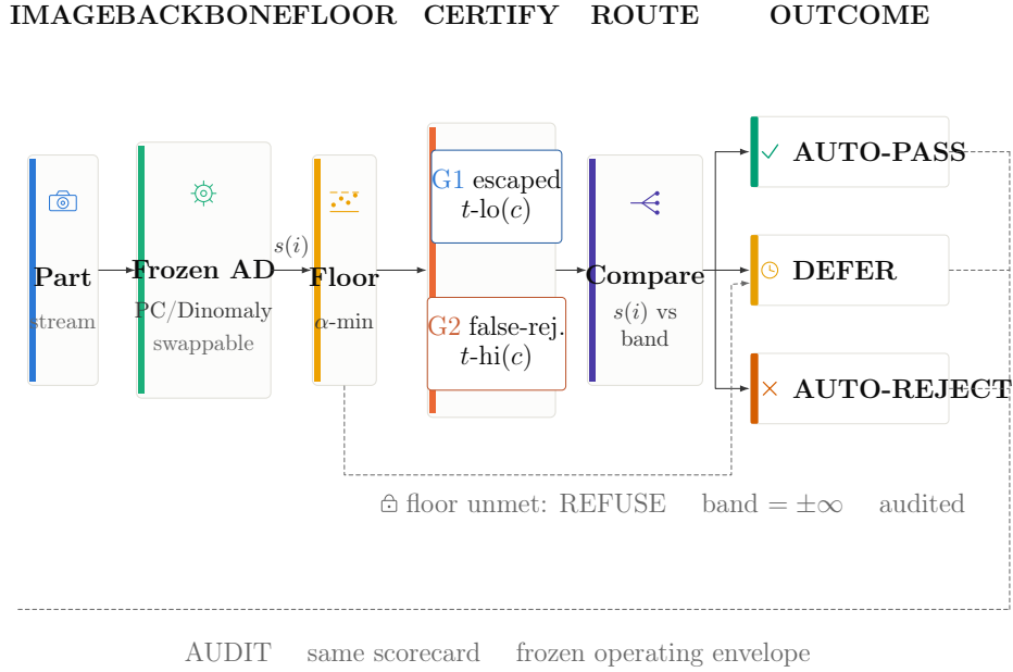
Figure 1: Horizontal method overview. A frozen, interchangeable PatchCore or Dinomally backbone scores each image. Per-category calibration first checks the certifiability floor \alpha_{\min} = 1/(n_{\text{cal}} + 1) (Section 3.2); when met, the parallel G1 and G2 cards set t_{\text{lo}}(c) and t_{\text{hi}}(c) so that P(s \leq t_{\text{lo}} \mid \text{defective}) \leq \alpha_{\text{miss}} and P(s \geq t_{\text{hi}} \mid \text{good}) \leq \alpha_{\text{fr}} , respectively (Section 3.1). Comparing s_i with this band routes the part to auto-pass, defer, or auto-reject. The dashed floor-control branch is distinct from that data path: an unmet floor refuses the axis (band = \pm\infty ), records audited-not-certified, and forces defer rather than auto-reject. All three outcomes feed the same audit scorecard and frozen operating envelope; the schematic makes no claim that either backbone is superior.
