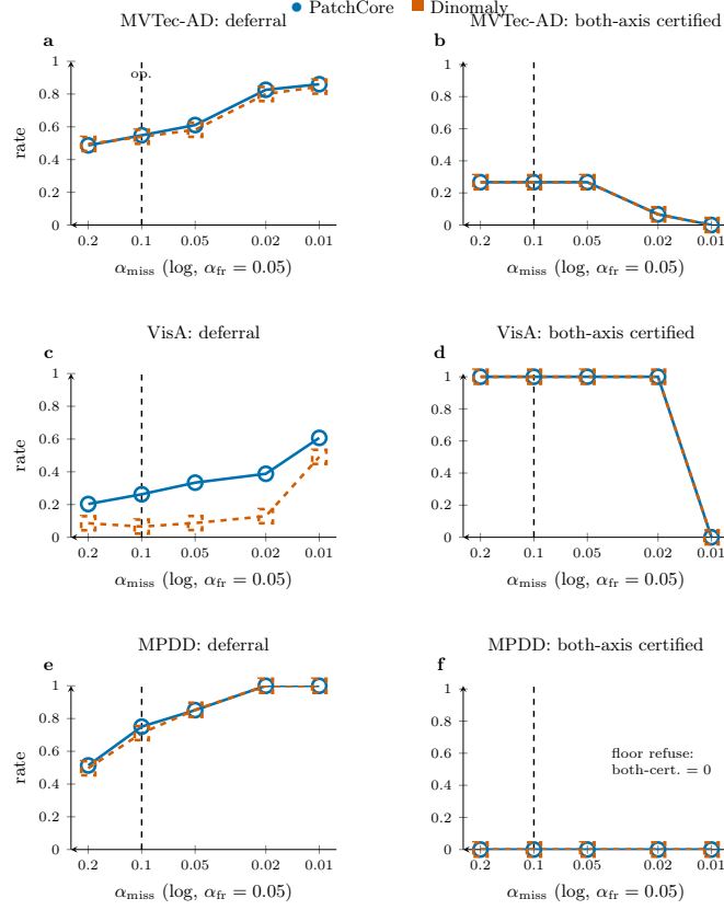
Figure 5: The operating-point frontier on the frozen code path (post-freeze exploratory sweep; the construction reproduces every frozen artifact exactly at the paper’s operating point). Rows are MVTec AD (a,b), VisA (c,d), and MPDD (e,f). Left panels show mean deferral versus the escaped-defect target \alpha_{\text{miss}} at \alpha_{\text{fr}} = 0.05 ; right panels show the fraction of categories certified on both axes. Solid circles denote PatchCore and dashed squares Dinomaly; shaded bands span seed minima to maxima. The vertical dashed line marks the paper’s operating point. The flat zero in panel (f) for MPDD at \alpha_{\text{miss}} \in \{0.02, 0.01\} is a measured refusal: the floor ( \alpha_{\text{min}} = 1/(n_{\text{cal}}^{\text{frac}} + 1) ) refuses all six MPDD categories, so both-certified is identically zero on every repeat and deferral saturates at 1.0 (no silent decisions).
