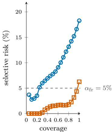
PatchCore Dinomaly b risk-coverage (VisA)
