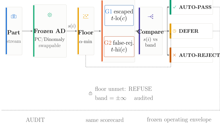
Figure 1: Method overview. A frozen backbone (PatchCore or Dinomaly, interchangeable) scores each image; per-category calibration checks the certifiability floor \alpha_{\min} = 1/(n_{\text{cal}} + 1) (Section 3.2) and, when met, sets the G1 escaped-defect threshold t_{lo}(c) and the G2 false-reject threshold t_{hi}(c) (Section 3.1). The three-way route then compares each score against (t_{lo}, t_{hi}) to auto-pass, defer, or auto-reject, carrying the stated escaped-defect and false-reject guarantees; an unmet floor instead refuses the axis (band = \pm\infty ), defers, and is reported audited-not-certified.
