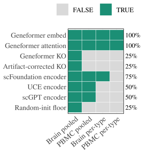
Graph coverage
