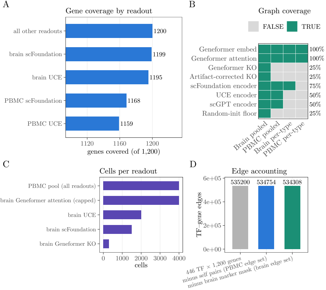
Figure 13: Coverage and fixed-panel quality control on the frozen 446 \times 1,200 TF \times gene panel. (A) Fraction of each encoder’s manifest genes present in the audit gene list. (B) Validated graph availability by tissue and analysis level; coverage is reported rather than assumed balanced. (C) Cell counts used by representative pooled inference runs. (D) Edge accounting from the Cartesian panel through self-pair and brain marker-mask exclusions.
