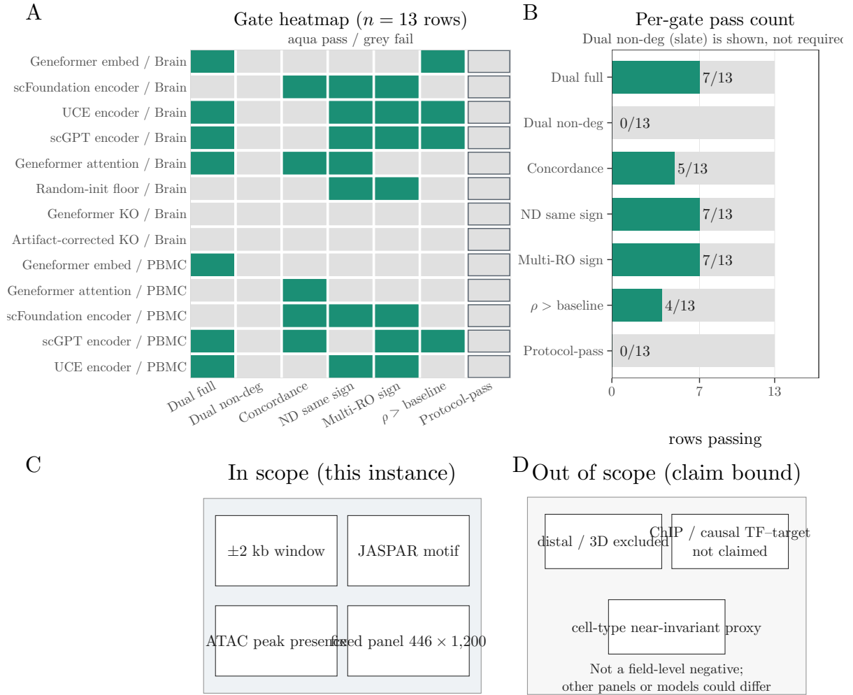
Figure 12: Protocol-pass gates and this audit instance’s scope on the thirteen pooled foundation-model (FM)/readout rows. (A) Binary gate heatmap (aqua pass, grey fail). Dual full / Dual non-deg: both within-family BH q_M, q_D < 0.05 under the named confound specification. Concordance: FM-co-expression Spearman > 0 . ND same sign: full and non-degree partial \rho share sign. Multi-RO sign: all full-spec readouts of the same model family in that tissue agree in sign (single-readout families pass). \rho > \text{baseline} : full-spec \rho exceeds the tissue co-expression baseline on the same edge set. Protocol-pass (outlined column) is the conjunction of Dual full, Concordance, ND same sign, Multi-RO sign, and \rho > \text{baseline} ; Dual non-deg is shown but not required. No row passes (0/13). (B) Column sums of panel A: how many of the thirteen rows pass each gate (slate bar = Dual non-deg, reported only). (C) What this instance scores: JASPAR motif matches in \pm 2 kb-linked ATAC peaks on the frozen 446 \times 1,200 TF \times gene panel. (D) What it does not score: distal/3D structure and ChIP-derived causal TF-target maps; the proxy is cell-type near-invariant on this panel. Failure on this instance cannot be read as a field-level negative.
