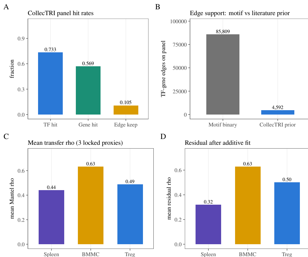
Figure A2. CollectTRI literature prior versus motif-binary support on the fixed panel, with summary transfer statistics. CollectTRI signed TF–gene interactions were projected onto the 446 \times 1,200 panel (absolute weight; maximum over duplicate edges). Motif-binary support is the count of nonzero edges in a magnitude-ablated copy of the brain reference graph. (A) Hit rates: 327/446 TFs (0.733), 683/1,200 genes (0.569), and 4,592/43,536 raw CollectTRI edges kept (0.105). The prior is TF-rich relative to genes and sparse relative to its own table. (B) Edge counts on the panel: motif-binary 85,809 versus CollectTRI 4,592 (about 19 \times sparser). A prior of this density cannot replace the accessibility/motif graph as a reference. (C) Mean Mantel \rho of each overlay against the three reference graphs: spleen 0.44, BMMC 0.63, Treg 0.49. (D) Mean residual \rho after additive removal: spleen 0.32, BMMC 0.63, Treg 0.50. BMMC’s residual mean matching its transfer mean is the low-additive-fraction fact in another view; spleen’s drop 0.44 \rightarrow 0.32 is the complementary additive fact. CollectTRI is not treated as a causal regulon gold standard.
