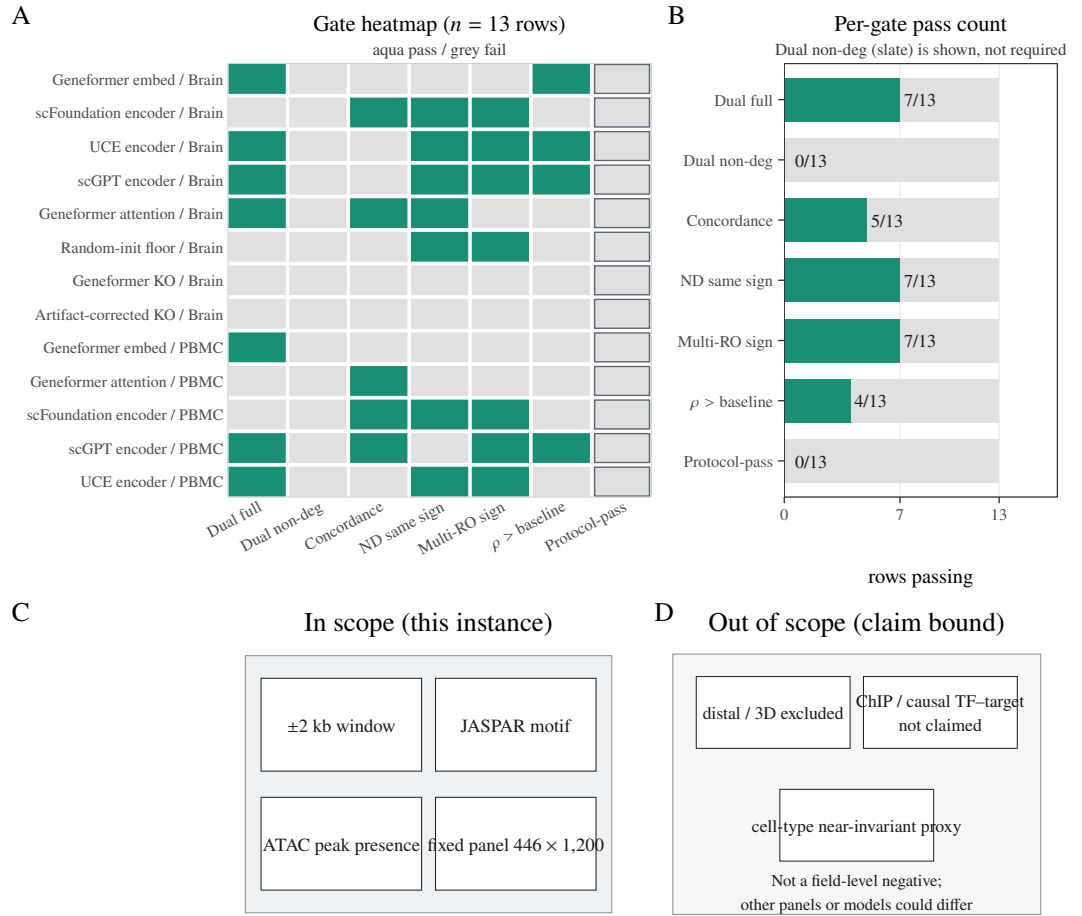
Figure 12. Protocol-pass and instance scope on the thirteen pooled foundation-model (FM)/readout rows. (A) Binary gate heatmap (aqua pass, grey fail). Dual full / Dual non-deg: both within-family BH q_M, q_D < 0.05 under the named confound specification. Concordance: FM-co-expression Spearman > 0 . ND same sign: full and non-degree partial \rho share sign. Multi-RO sign: all full-spec readouts of the same model family in that tissue agree in sign (single-readout families pass). \rho > \text{baseline} : full-spec \rho exceeds the tissue co-expression baseline on the same edge set. Protocol-pass (outlined column) is the conjunction of Dual full, Concordance, ND same sign, Multi-RO sign, and \rho > \text{baseline} ; Dual non-deg is shown but not required. No row passes (0/13). (B) Column sums of panel A: how many of the thirteen rows pass each gate (slate bar = Dual non-deg, reported only). (C) What this instance scores: JASPAR motif matches in \pm 2 kb-linked ATAC peaks on the frozen 446 \times 1,200 TF \times gene panel. (D) What it does not score: distal/3D structure and ChIP-derived causal TF-target maps; the proxy is cell-type near-invariant on this panel. Failure on this instance cannot be read as a field-level negative.
