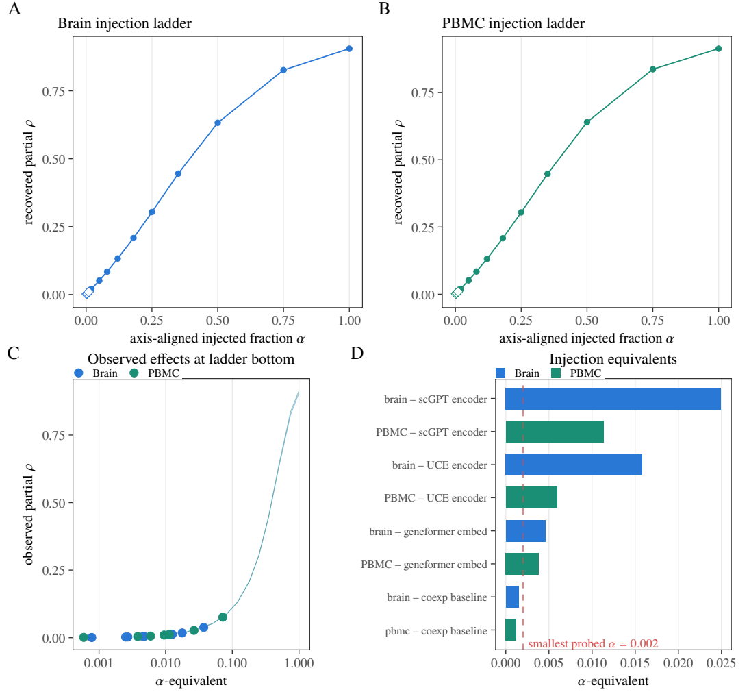
Figure 9. Axis-aligned pipeline-sensitivity diagnostic. \alpha is the injected fraction of the proxy residual mixed with independent Gaussian noise. (A–B) Brain and PBMC ladders: lines are mean recovered partial \rho across 30 independent noise replicates, ribbons the replicate range, diamonds the subdivided low- \alpha points. (C) Observed full-spec effects located on those curves. (D) \alpha -equivalents of the six dual-null supported positive rows versus the smallest probed nonzero \alpha = 0.002 ; the negative brain Geneformer-attention row has no positive \alpha -equivalent. This is not a confidence interval, power curve, minimum detectable effect, or exclusion analysis.
