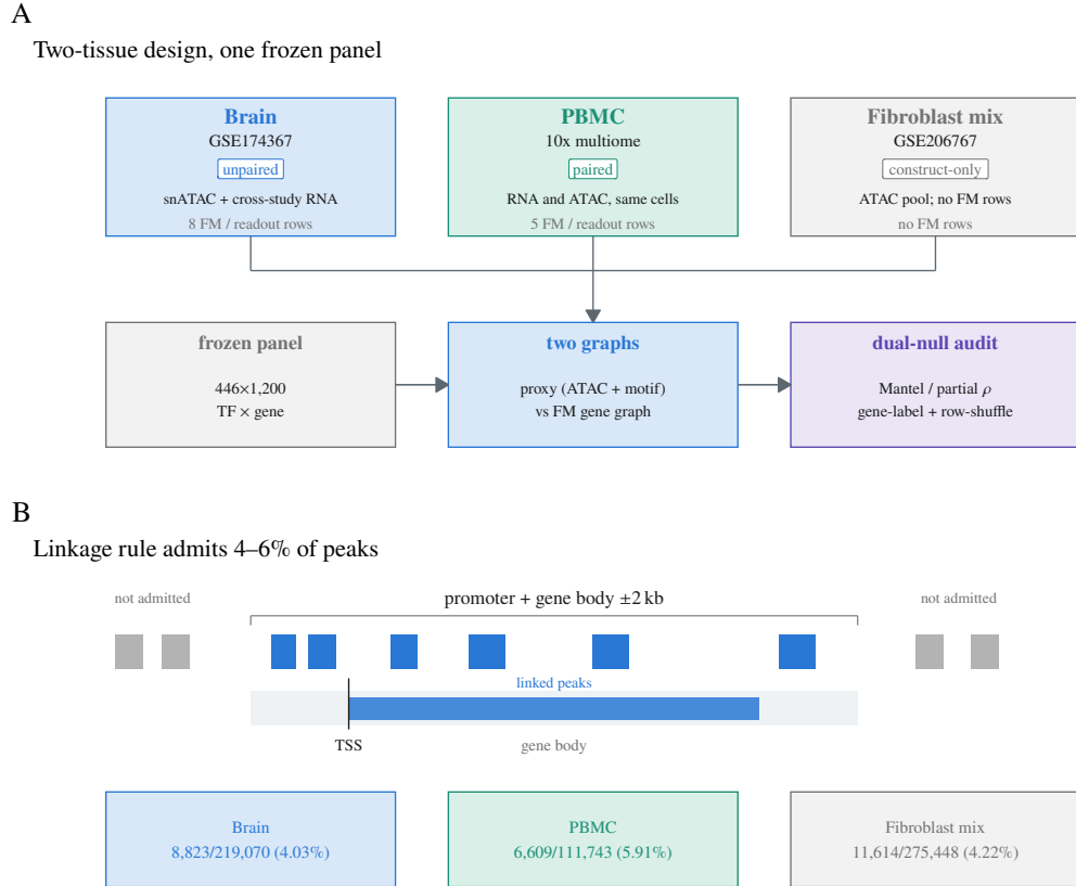
Figure 1. Two-tissue study design and the \pm 2 kb linkage rule. (A) Unpaired brain snATAC (GSE174367) plus cross-study RNA versus paired PBMC 10x multiome RNA/ATAC; the fibroblast mix (GSE206767) is construct-only and contributes no foundation-model (FM) rows. All arms freeze the same 446 \times 1,200 panel, then compare an accessibility/motif proxy graph with each FM gene graph under dual-null Mantel/partial \rho . (B) Peaks are admitted only inside a promoter-plus-gene-body \pm 2 kb window: 8,823/219,070 (4.03%) in brain, 6,609/111,743 (5.91%) in PBMC, and 11,614/275,448 (4.22%) in the fibroblast mix. Distal and three-dimensional contacts are excluded by this rule.
