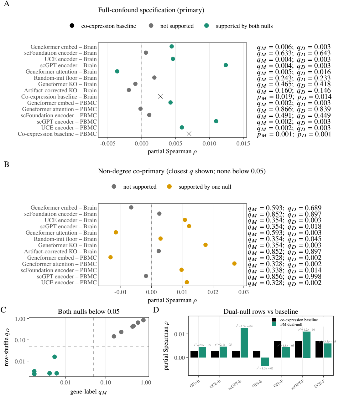
Figure 4. Primary fixed-panel audit of 13 pooled foundation-model (FM) readouts (Geneformer, UCE, scGPT, scFoundation, random-init floor, and Geneformer knockout variants) plus the same-edge co-expression baseline, under both prespecified confound specifications. M is the gene-label (Mantel) null and D the within-TF-row degree-preserving shuffle ( N = 999 each); FM q values are BH-adjusted within tissue-by-specification-by-null families. Dual-null Support requires q_M < 0.05 and q_D < 0.05 . (A) Full-confound rows; labels are BH q_M, q_D for FM rows and uncorrected p_M, p_D for the baseline (aqua = both nulls, yellow = one null, grey = neither, black = baseline). (B) Non-degree co-primary rows; no row is supported by both nulls. (C) Full-confound q_M versus q_D ; dashed lines at 0.05. (D) Dual-null FM rows versus the tissue co-expression baseline; r^2 = \rho^2 on FM bars (tiny effects; several dual-null positives do not exceed baseline). Dual-null Support is not protocol-pass.
