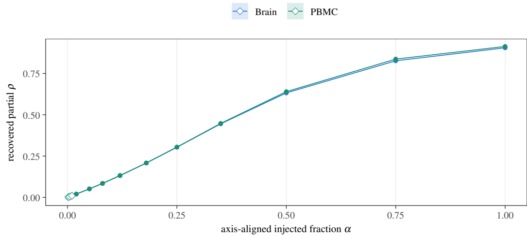
Figure 5. Axis-aligned pipeline-sensitivity diagnostic. Lines show the mean across 30 independent noise replicates and ribbons show the replicate range. This is not a confidence interval, power curve, MDE, or exclusion analysis.
