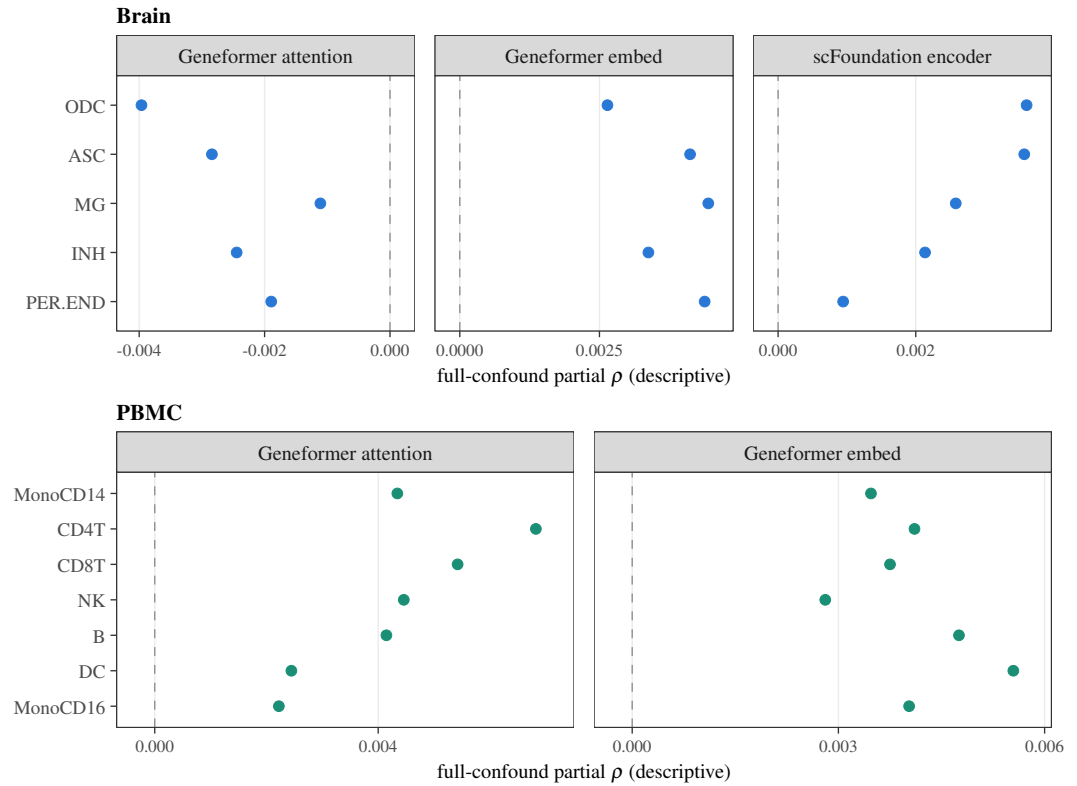
Figure 4. Per-cell-type full-confound estimates. These observed effects are descriptive exploratory robustness checks without randomization p -values or multiplicity claims.
