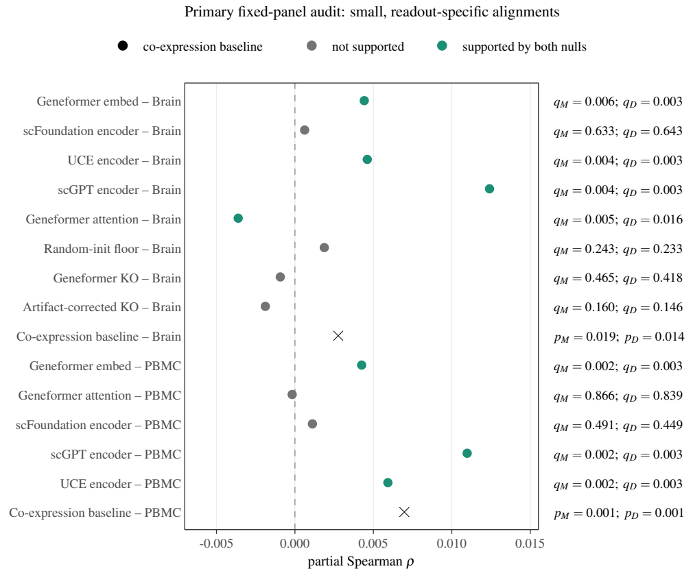
Figure 2. Primary full-confound fixed-panel audit. Points are observed partial Spearman correlations; labels give BH-adjusted gene-label ( q_M ) and row-shuffle ( q_D ) values within prespecified families. Green rows are supported by both nulls at q < 0.05 . Crosses mark the co-expression baseline, tested outside the FM families with uncorrected p -values.
