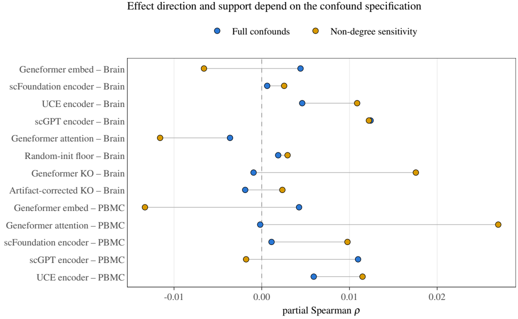
Figure 3. Confound-specification sensitivity. Full and non-degree estimates are joined within each model/readout and tissue. The non-degree specification is reported co-primary and shows null-dependent support.
