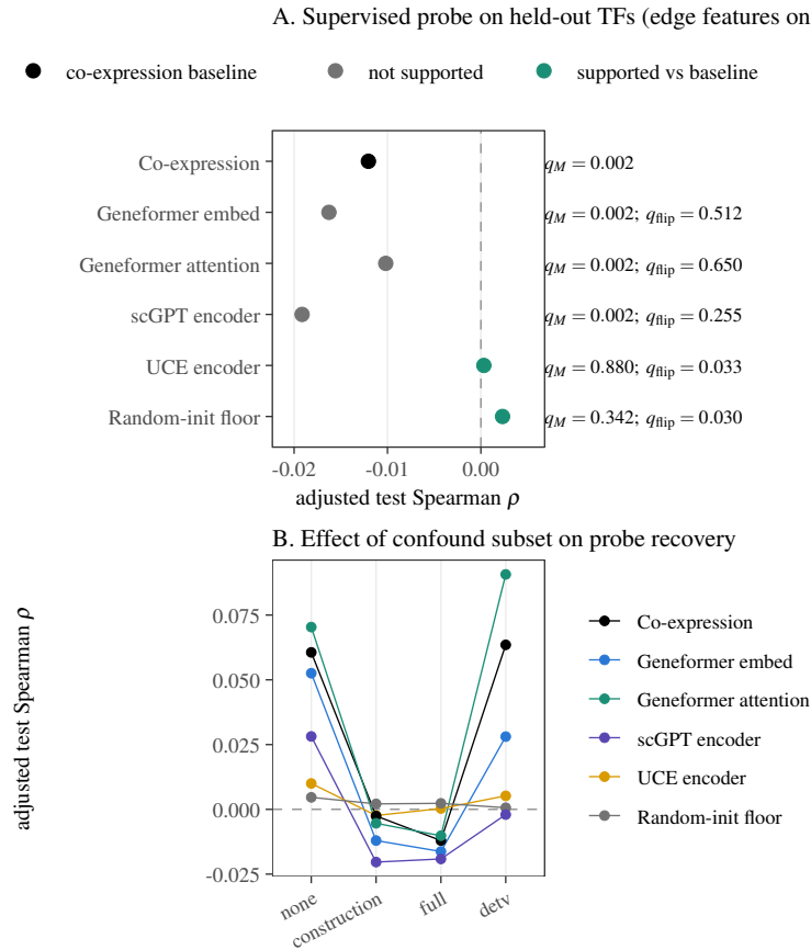
Figure 6. TF-disjoint supervised probe. (A) Confound-adjusted test correlation per family on 135 held-out TFs; labels give the gene-label permutation q_M and, for each FM family, the paired sign-flip q_{\text{flip}} against the co-expression baseline. Green rows are supported against the baseline at q_{\text{flip}} < 0.05 (UCE 0.0325; random-init floor 0.0300), and the supported floor contrast prevents a model-specific reading of UCE. (B) The same readout across confound subsets; recovery collapses once the proxy’s construction covariates (peak count, gene length, GC) are conditioned on, and random-init stays at zero throughout.
