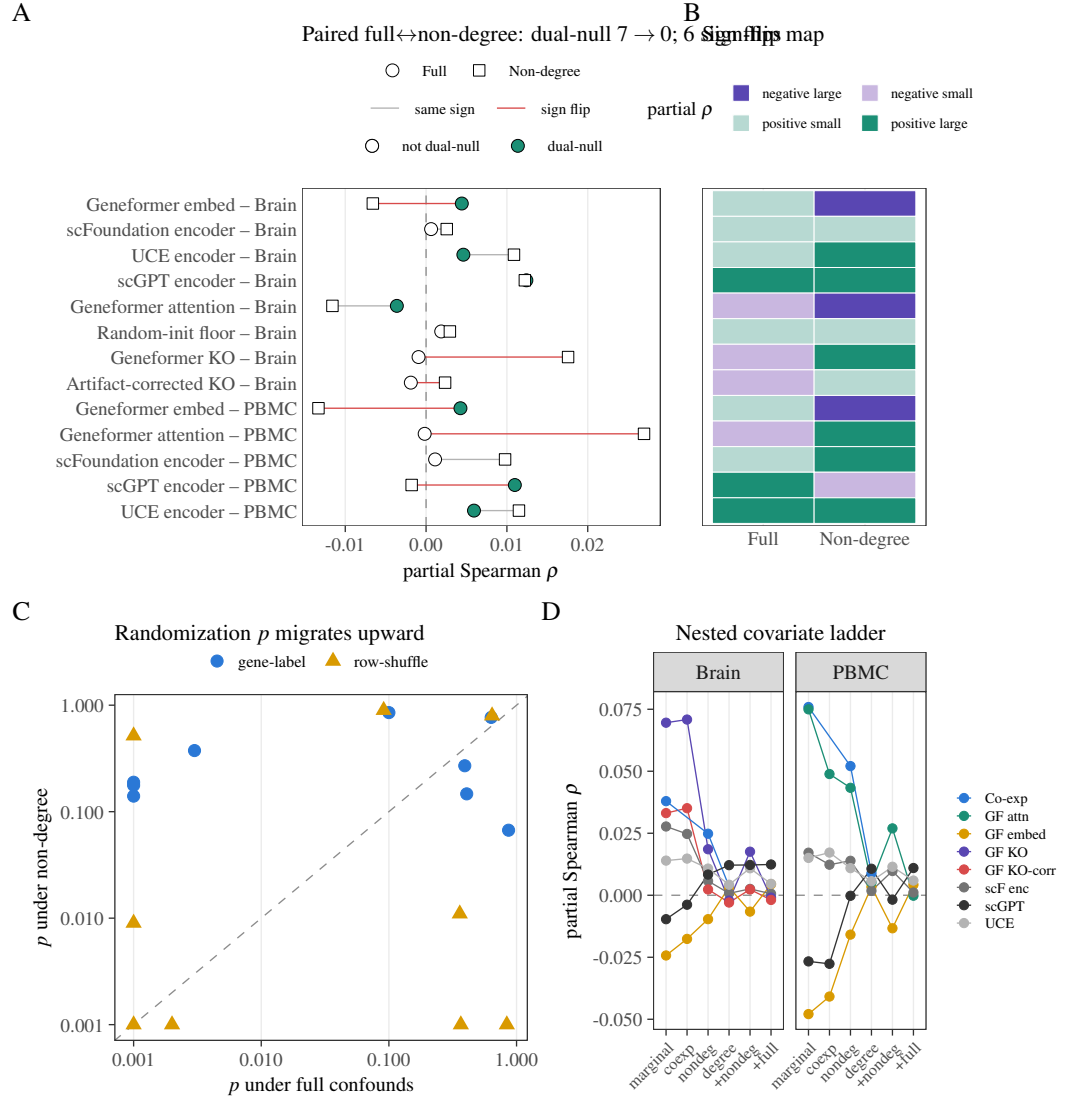
Figure 7. Dependence on the confound specification. (A) Paired full ↔ non-degree partial \rho for all 13 FM rows: circles full, squares non-degree; aqua fill marks dual-null Support (7 under full, 0 under non-degree); red segments mark sign flips. (B) Effect-sign map across specifications. (C) Full-confound versus non-degree randomization p -values for both nulls. (D) Nested covariate ladder from marginal correlation to the primary rung; lines are descriptive and are not a model-selection exercise.
