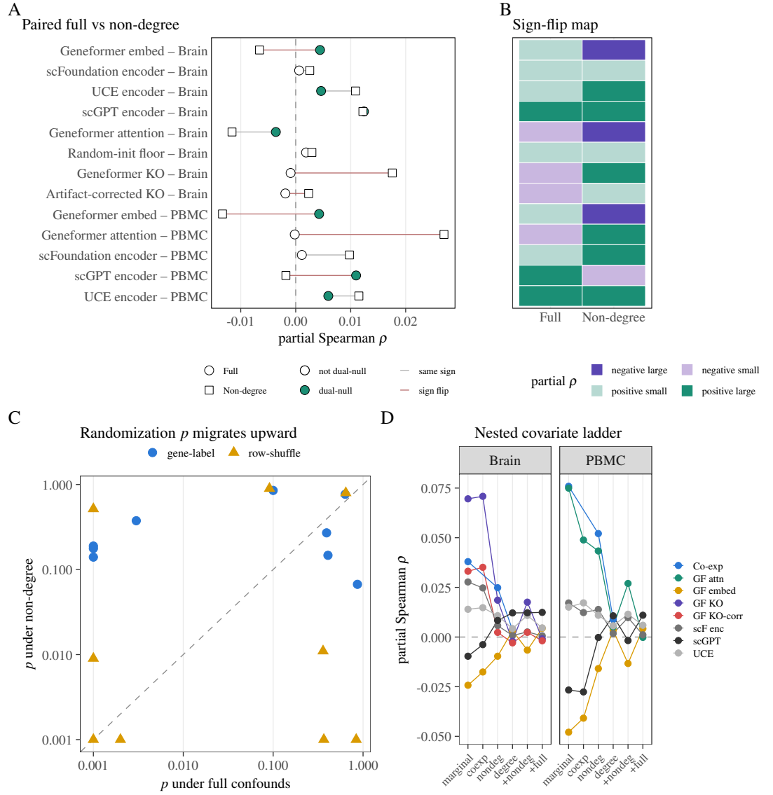
Figure 7. Dependence on the confound specification. (A) Paired full \leftrightarrow non-degree partial \rho for all 13 FM rows: circles full, squares non-degree; aqua fill marks dual-null Support (7 under full, 0 under non-degree); red segments mark sign flips. (B) Effect-sign map across specifications. (C) Full-confound versus non-degree randomization p -values for both nulls. (D) Nested covariate ladder from marginal correlation to the primary rung; lines are descriptive and are not a model-selection exercise.
