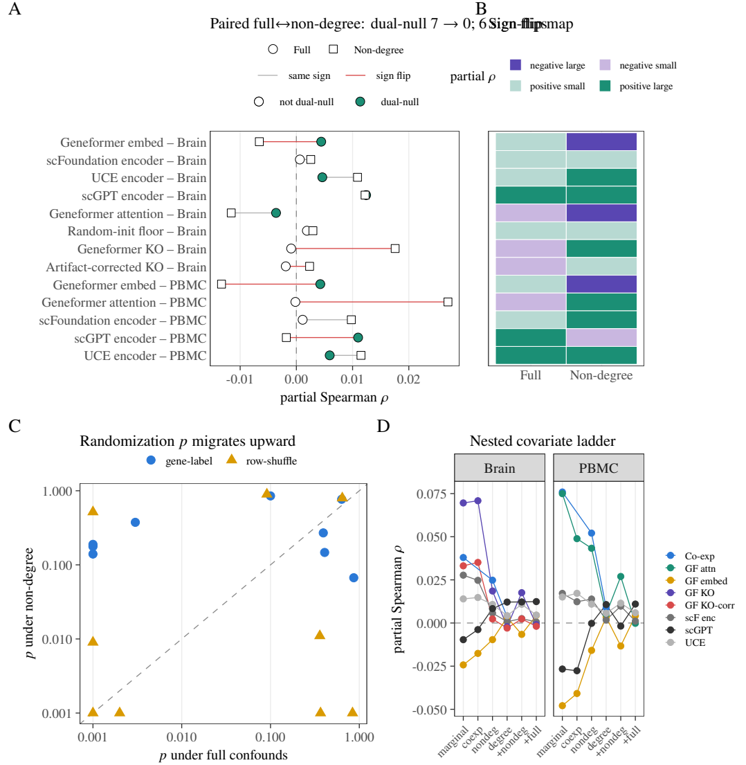
Figure 7. Dependence on the confound specification. (A) Paired full ↔ non-degree partial \rho for all 13 FM rows: circles full, squares non-degree; aqua fill marks dual-null Support (7 under full, 0 under non-degree); red segments mark sign flips. (B) Effect-sign map across specifications. (C) Full-confound versus non-degree randomization p -values for both nulls. (D) Nested covariate ladder from marginal correlation to the primary rung; lines are descriptive and are not a model-selection exercise.
