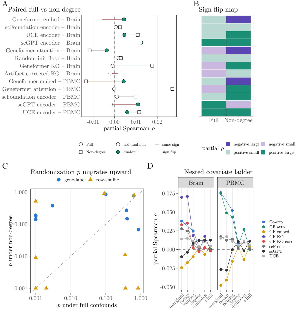
Figure 7: Dependence of foundation-model (FM) alignments on the confound specification. (A) Paired full versus non-degree partial \rho for all 13 FM rows (circles full, squares non-degree); aqua fill marks dual-null Support, which falls from 7 under full to 0 under non-degree, and red segments mark sign flips (6 of 13 rows). (B) Sign map of those paired effects. (C) Full-confound versus non-degree randomization p -values for the gene-label and row-shuffle nulls. (D) Nested covariate ladder from marginal correlation through co-expression, non-degree, and degree rungs to the full specification; the sequence is descriptive and is not a model-selection criterion.
