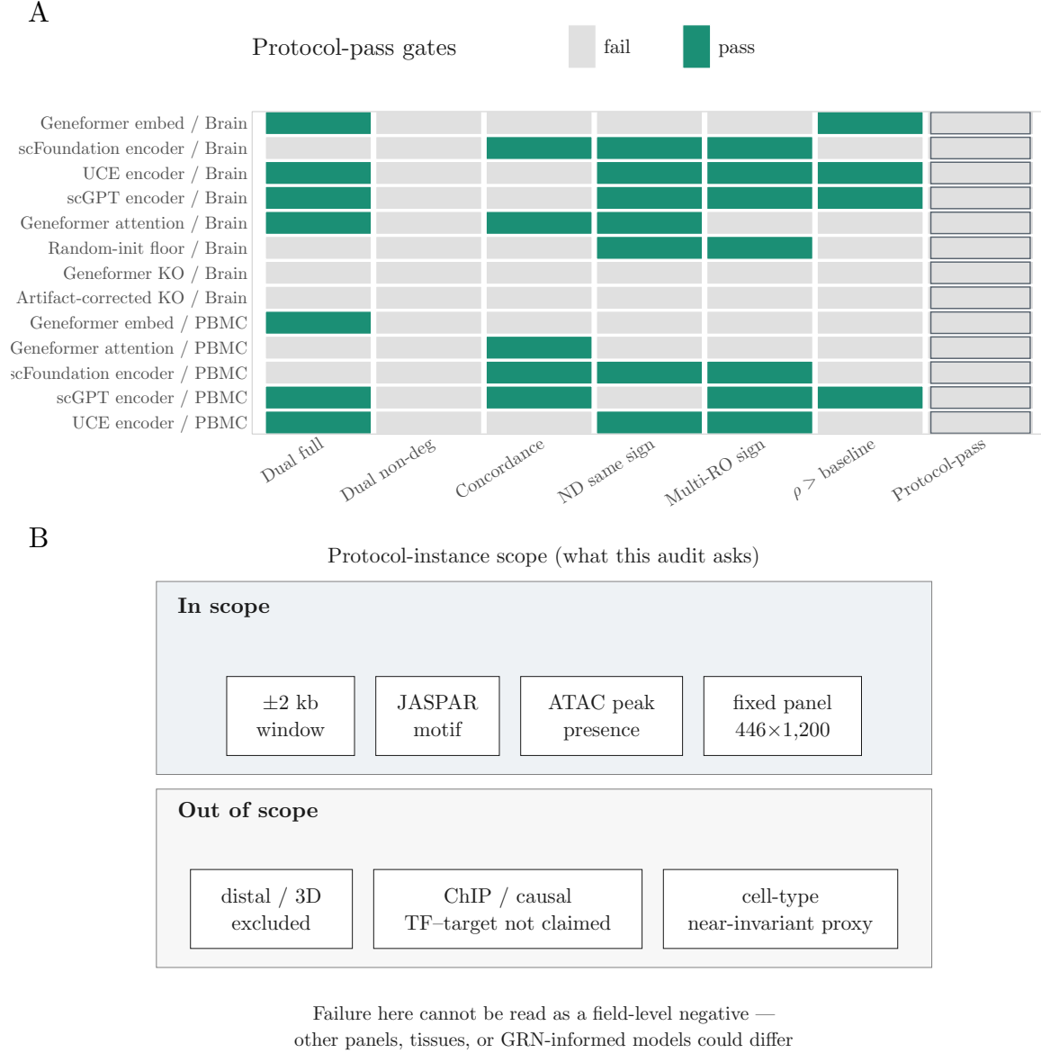
Figure 12: Protocol-pass gates and this audit instance’s scope. (A) Aqua pass / grey fail on thirteen foundation-model (FM) readout rows for six reporting gates plus their conjunction (rightmost column). Gates: dual-null under the full confound specification; dual-null under the non-degree specification (shown, not required); concordance (FM-co-expression Spearman > 0 ); non-degree same sign as the full estimate; multi-readout sign agreement within model family and tissue; and full-spec \rho strictly above the tissue co-expression baseline. Protocol-pass is that conjunction except dual non-degree; 0/13 rows pass. (B) What this instance asks—motif matches in \pm 2 kb-linked ATAC peaks on a fixed 446 \times 1,200 panel—not distal/3D structure and not ChIP-derived causal TF-target maps. This is instance scope, not a field-level negative.
