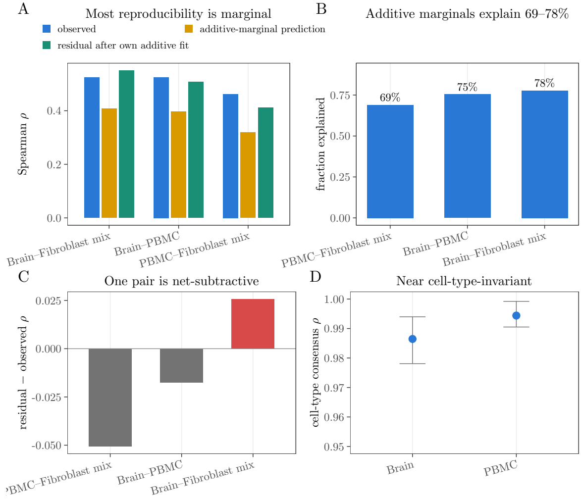
Figure 3: Cross-tissue structure of the regulatory-potential proxy. (A) Observed Spearman \rho , TF-row-plus-gene-column additive prediction, and residual agreement after removing each tissue’s own additive fit. (B) Fraction of observed agreement predicted by those additive marginals (69–78%). (C) Residual minus observed \rho ; the brain–fibroblast mix pair is net-subtractive. (D) Range and mean of pairwise cell-type proxy correlations within brain and PBMC (consensus \rho near 1). These are descriptive fixed-panel quantities without new randomization inference.
