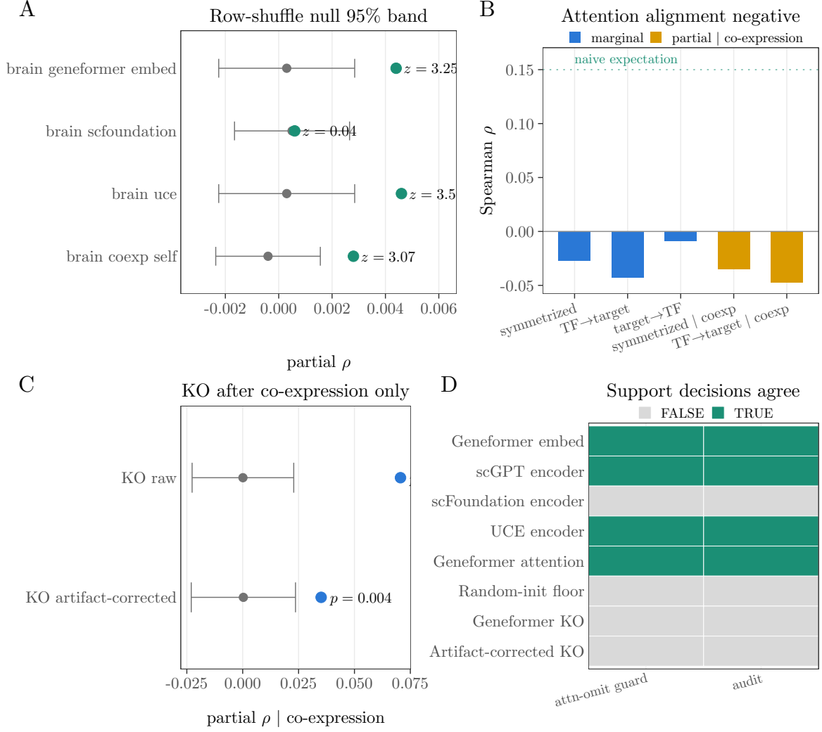
Figure 6: Randomization and readout diagnostics. (A) Observed partial \rho against the within-TF-row degree-preserving row-shuffle null mean and 95% null band for representative rows. (B) Brain Geneformer-attention alignment, marginally and after adjusting for co-expression. (C) Geneformer knockout (KO) raw and artifact-corrected (position-shift) KO both align with the proxy after partialling co-expression alone ( p < 0.001 and p = 0.004 ); the full confound specification removes that alignment. (D) Dual-null Support decisions agree between the authoritative audit and a parallel attention-omission guard (same eight brain rows).
