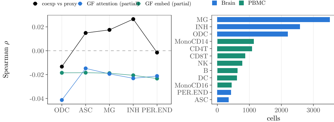
Figure 8: Per-cell-type descriptive robustness summaries. (A) Brain full-confound rows by readout. (B) PBMC full-confound rows by readout. (C) Earlier brain per-type co-expression, Geneformer- embedding, and Geneformer-attention summaries on the same fixed panel. (D) Cell counts underlying the per-type rows. These observed effects have no randomization p -values, multiplicity claims, or population-uncertainty interpretation.
