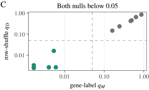
Figure 4. Primary fixed-panel audit under both prespecified confound specifications. (A) Full- confound pooled rows and the same-edge co-expression baseline; labels give BH-adjusted q_M and q_D for FM rows and uncorrected p_M, p_D for the baseline. (B) Non-degree co-primary rows; no row is supported by both nulls. (C) Full-confound q_M versus q_D ; support requires both coordinates below 0.05. (D) Dual-null rows versus the same-edge co-expression baseline with r^2 = \rho^2 on FM bars (tiny effects; several dual-null positives do not exceed baseline).
