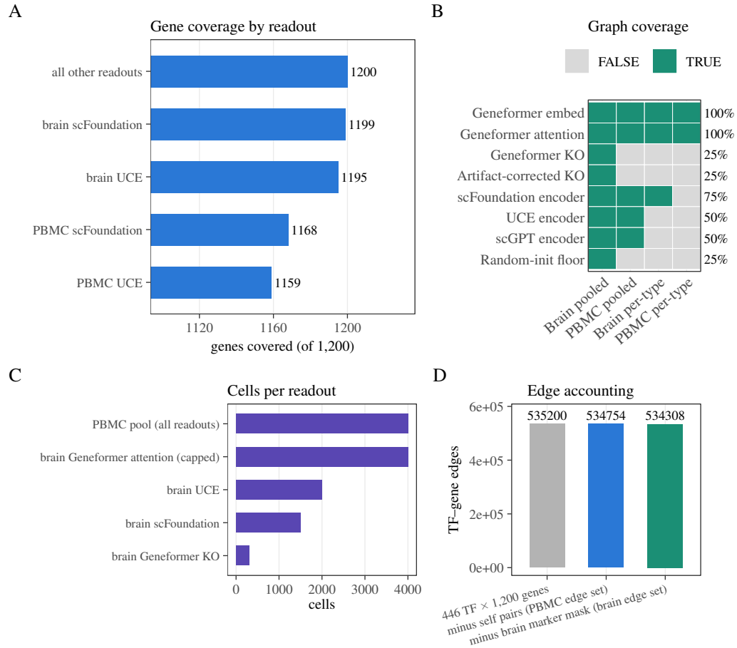
Figure 13. Coverage and fixed-panel quality control. (A) Manifest-gene coverage for encoder readouts. (B) Validated graph availability by tissue and analysis level; coverage is intentionally reported rather than assumed balanced. (C) Cell counts used by representative pooled inference runs. (D) Edge accounting from the 446 \times 1,200 Cartesian panel through self-pair and brain marker-mask exclusions.
