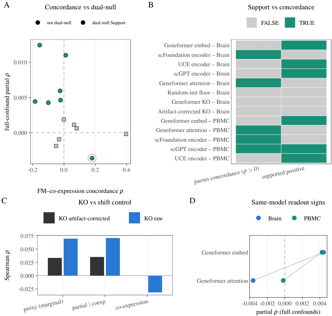
Figure 5. Readout concordance (attention-likeness) and internal consistency. (A) Scatter of FM-co-expression concordance versus full-confound partial \rho for all 13 pooled readouts; fill encodes dual-null Support, and the open red ring marks brain Geneformer attention (concordance passer, dual-null negative). (B) Positive joint-null support and positive concordance as separate binary checks. (C) Marginal and partial behavior of the Geneformer knockout readout and its artifact-corrected knockout readout. (D) Geneformer embedding and attention effects within each tissue; the brain effects have opposite signs.
