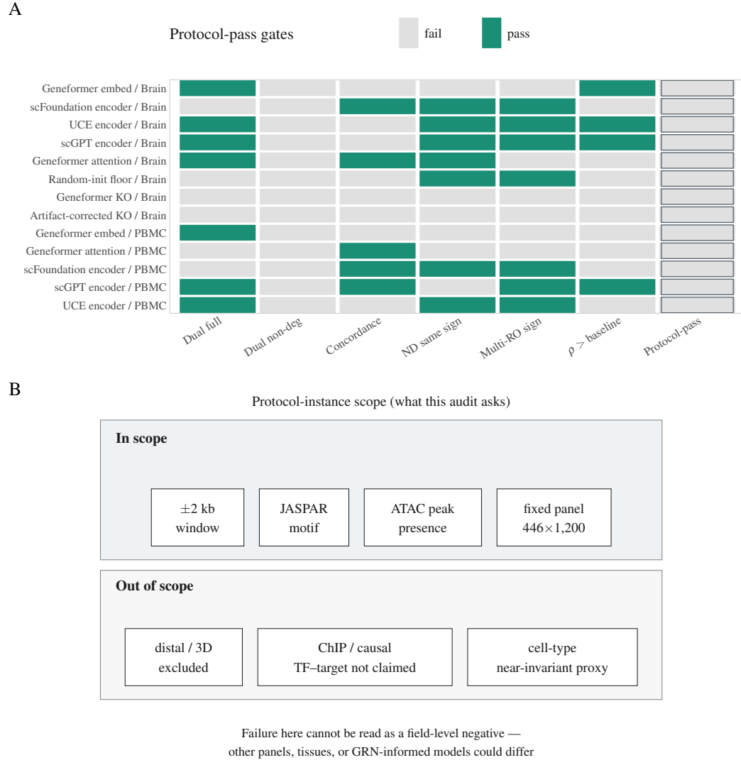
Figure 12. Protocol-pass and instance scope. (A) Binary gate heatmap for the thirteen pooled FM/readout rows (aqua pass, grey fail). Protocol-pass is the conjunction column (outlined); no row passes (0/13). (B) Protocol-instance scope card: the audit scores motif matches in \pm 2 kb-linked ATAC peaks on a fixed panel. Distal/3D structure and ChIP-derived causal TF–target maps are out of scope; the proxy is cell-type near-invariant on this panel. Failure to support a global capability claim therefore cannot be read as a field-level negative.
