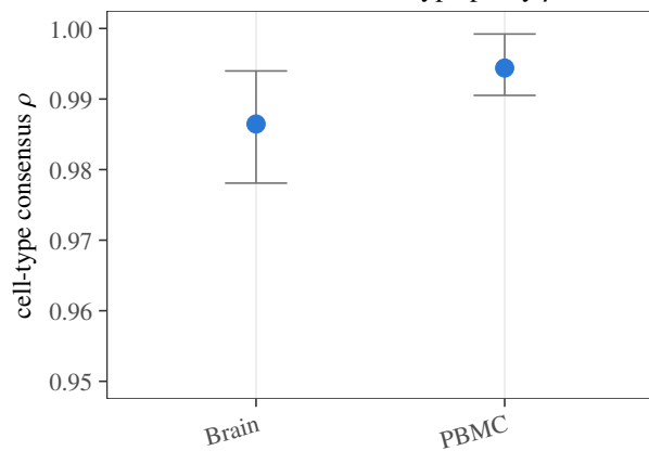
D Within-tissue cell-type proxy \rho
