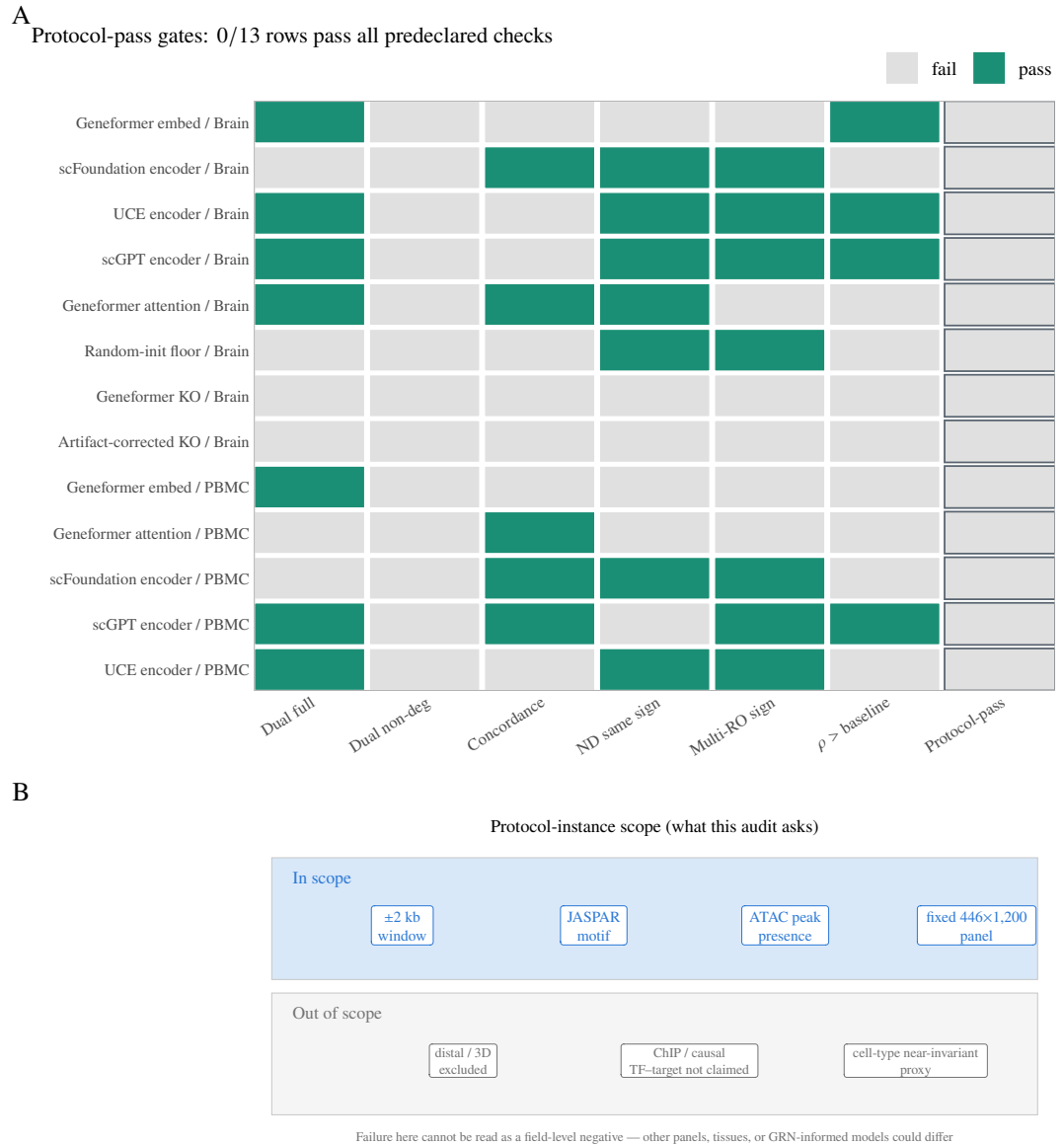
Figure 12. Protocol-pass and instance scope. (A) Binary gate heatmap for the thirteen pooled FM/readout rows (aqua pass, grey fail), companion to Table 4. Protocol-pass is the conjunction column (outlined); no row passes (0/13). (B) Protocol-instance scope card: the audit scores motif matches in \pm 2 kb-linked ATAC peaks on a fixed panel. Distal/3D structure and ChIP-derived causal TF–target maps are out of scope; the proxy is cell-type near-invariant on this panel. Failure to support a global capability claim therefore cannot be read as a field-level negative (Sec. 2.1).
